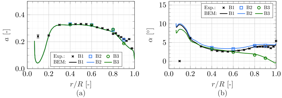
Figure 8. Spanwise distribution of the swept blades' axial induction (a) and angle of attack (b); Comparison between experiment and simulations
