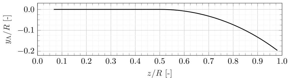
Figure 2. Swept blade axis
