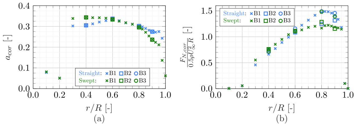
Figure 12. Comparison of corrected experimental results in terms of axial induction factor (a) and normal force distribution (b)
