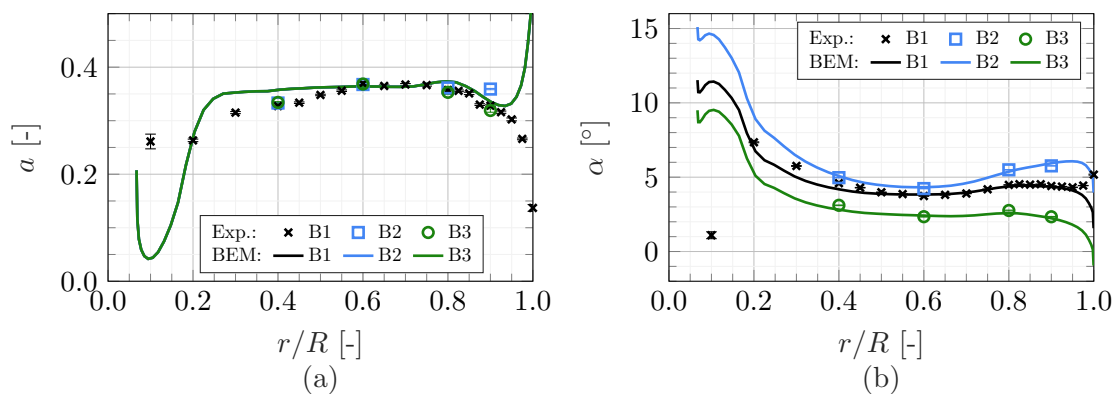
Figure 6. Spanwise distribution of the straight blades' axial induction (a) and angle of attack (b); Comparison between experiment and simulations
