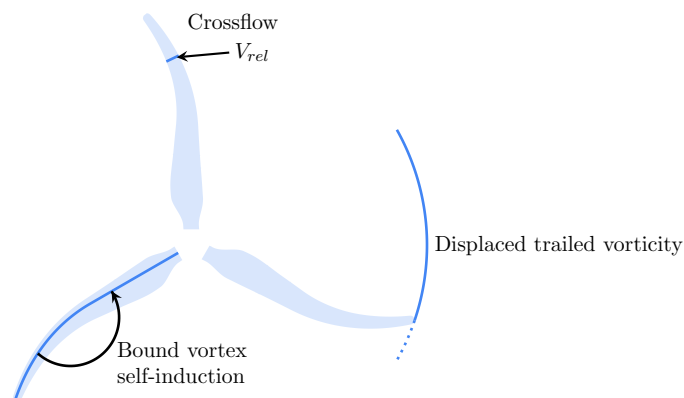
Figure 4. Schematic representation of the sweep-induced changes in blade aerodynamics
