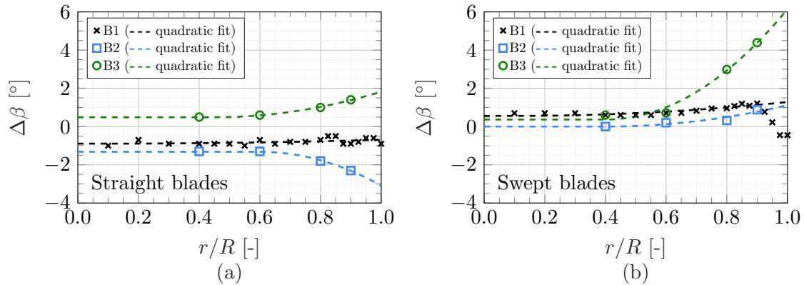
Figure 5. Combined pitch/twist offset \Delta\beta from the original design twist distribution for the straight blades (a) and swept blades (b)
