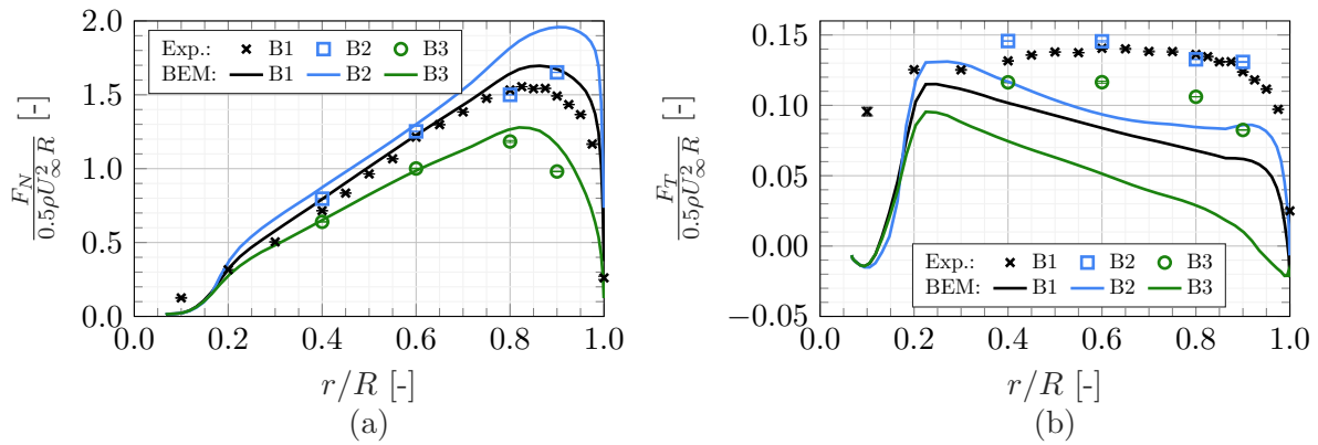
Figure 7. Spanwise distribution of the straight blades' normal (a) and tangential (b) force; Comparison between experiment and simulations
