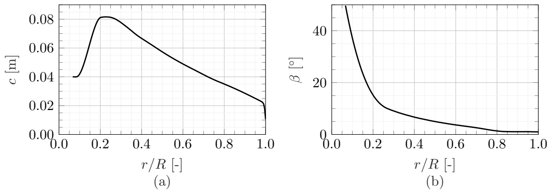
Figure 1. Chord (a) and twist (b) distribution of the scaled wind tunnel model blades
