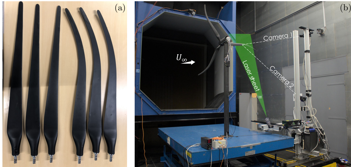
Figure 3. Straight and swept model wind turbine blades (a) and experimental setup including the PIV measurement system (b)
