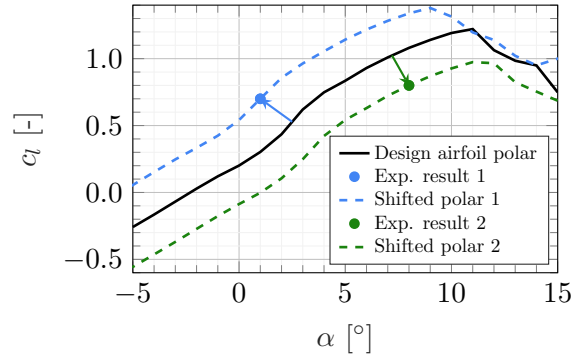
Figure 11. Schematic of the approach used to base the BEM lift polar input files on the experimentally derived lift polar
