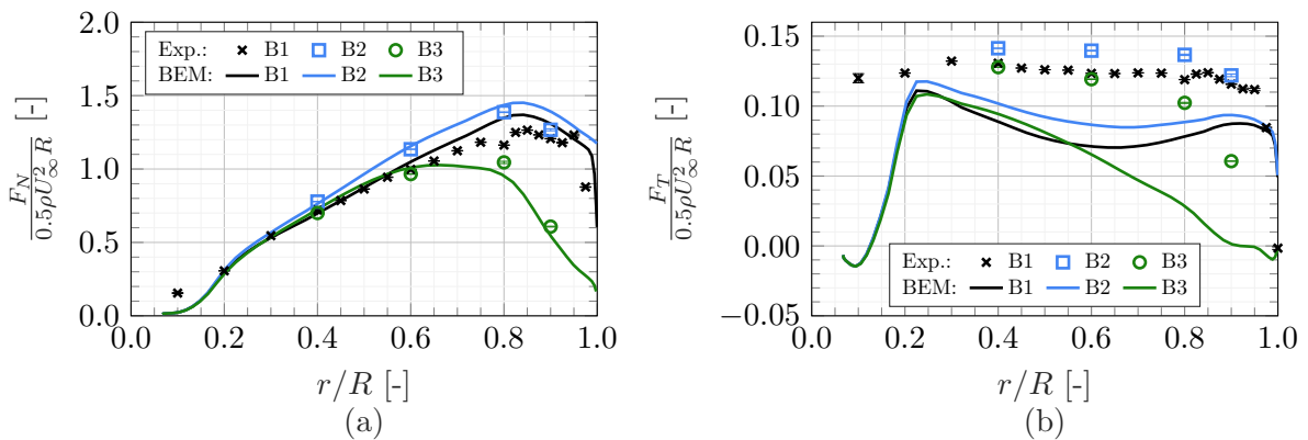
Figure 9. Spanwise distribution of the swept blades' normal (a) and tangential (b) force; Comparison between experiment and simulations
