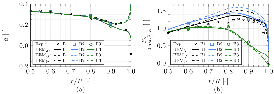
Figure 10. Comparison of various BEM implementations with the experimental results in terms of axial induction factor (a) and normal force distribution (b)
