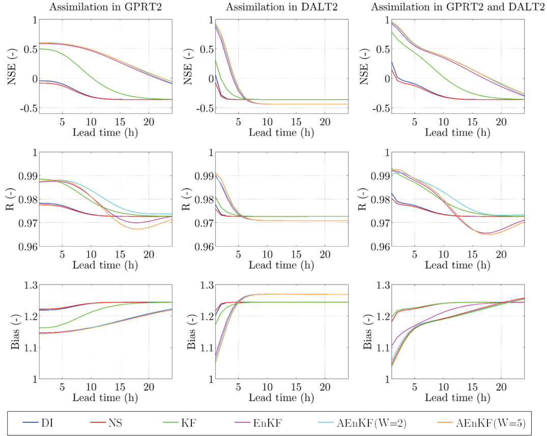
Figure 6.14. Comparison between observations and model predictions, in terms of NSE, R and Bias, in case of different lead time values and different StPh sensors location during peak 1 in the May-June 2015 flood event
