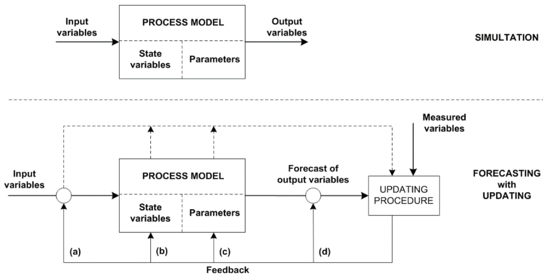
Figure 3.1. Schematic diagrams of simulation and forecasting with emphasis on the four different updating methodologies (modified after WMO 1992)
