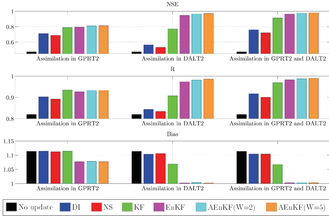
Figure 6.9. Value of NSE, R and Bias obtained using different DA methods in case of different location of the StPh sensors
