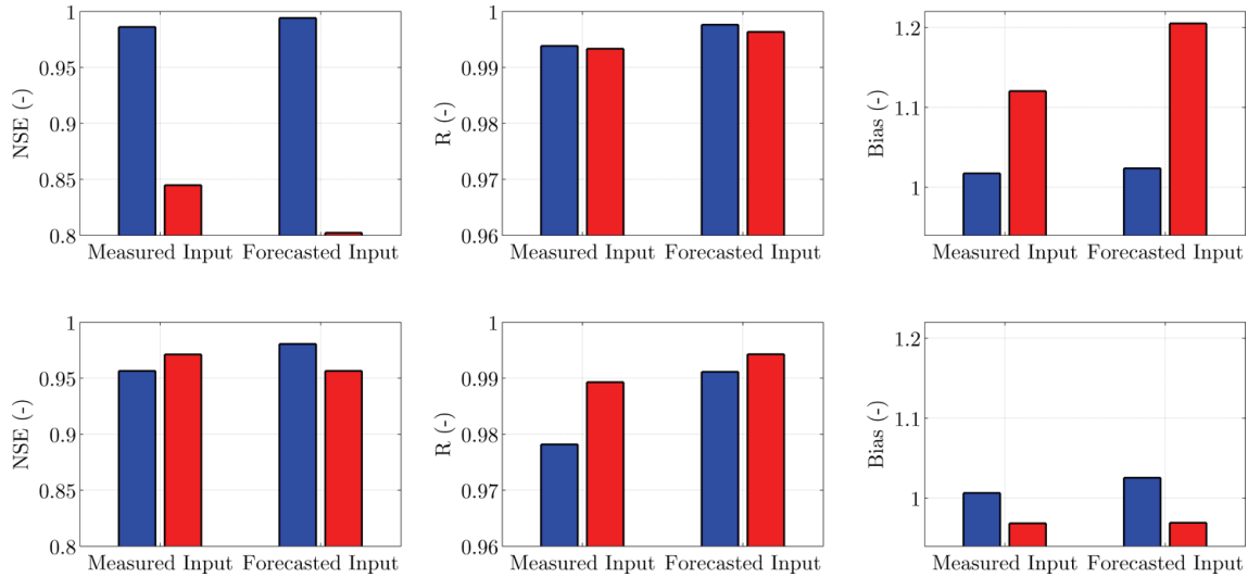
Figure 2.13. Statistical measures obtained comparing results obtained from MIKE11 and Muskingum-Cunge in terms of discharge (blue color) and water depth (red color) at PM (first row) and PA (second row)
