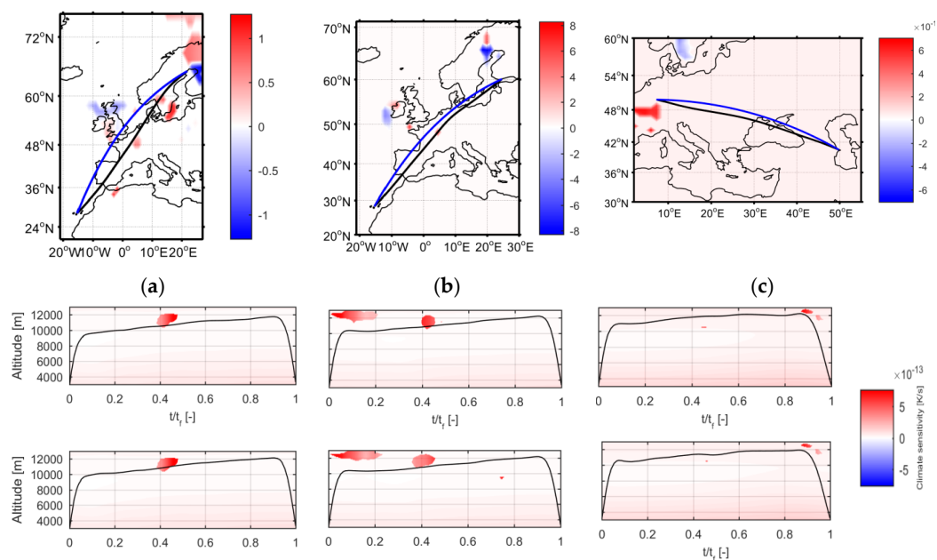
Figure 1. Aircraft trajectories (top row) Lulea–Gran Canaria (ESPA–GCLP, a ), Helsinki–Gran Canaria (EFHK–GCLP, b ), Baku–Luxembourg (UBBB–ELLX, c ): great circle (blue line), fuel-optimal trajectory (black line). Altitude profile: fuel optimal case (middle row) and climate optimized case with 0.5% additional costs (bottom row), indicating along individual cruise trajectories of the connection (altitude, position) by shading algorithmic climate change functions warming (red) and cooling impacts (blue), values provided as 10^{-13} K/s.
