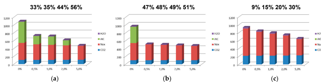
Figure 3. Individual contributions to total climate impact ( ATR_{20} , pK) on Lulea–Gran Canaria (a), Helsinki–Gran Canaria (b), Baku–Luxembourg (c); shown for individual mitigation trajectories allowing fuel increase by 0.5%, 1%, 2% and 5% and fuel optimal (0%). Numbers on top indicating decrease of total climate impact for respective alternative trajectory.
