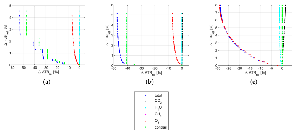
Figure 2. Pareto fronts for aircraft trajectory optimization showing average temperature response ( \Delta ATR_{20} ) vs. fuel increase for Lulea–Gran Canaria (a), Helsinki–Gran Canaria (b), Baku–Luxembourg (c) and individual effects. For given fuel increase, dark blue dots show the optimal climate change impact from the possible routes available. Other individual dot colours indicate the CO_2 and non- CO_2 climate impacts for that alternative route.
