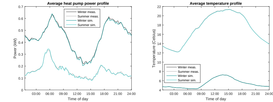
Figure 5.13: Average heat pump load and temperature profile during winter and summer.
