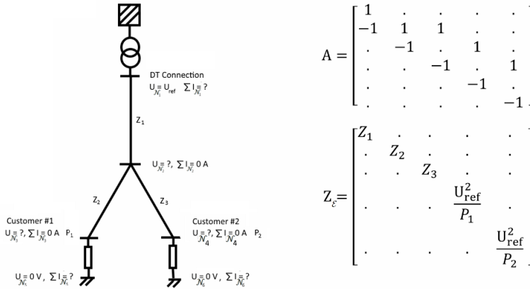
Figure 5.15: An example low voltage distribution network (left) and its corresponding A and Z_{\varepsilon} matrices (right).
