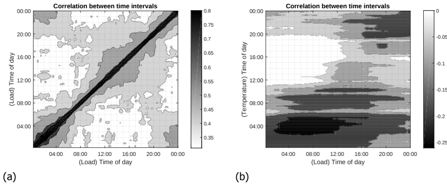
Figure 5.12: Correlation of power consumption at different time intervals, with darker shading indicating a larger magnitude of the correlation factor. (a) autocorrelation of electric load, (b) correlation of load with temperature.
