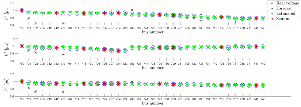
Figure 4.5: Example voltage profile with forecast and estimation update at all the buses, numbered as in Figure 4.4.
