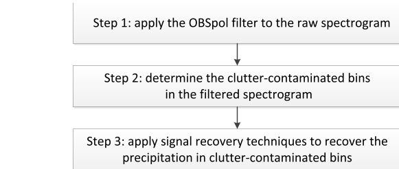
Fig. 1. Flowchart of the signal recovery techniques.
