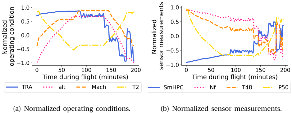
Figure 2.6.: Normalized operating conditions and normalized sensor measurements - flight 1, training engine 2 of DS02, N-CMAPSS.
