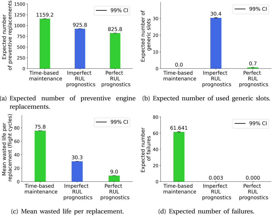
Figure 7.16.: The expected number of engine replacements, used generic slots and failures per ten years, and the mean wasted life per replacement, for i) time-based maintenance, ii) maintenance with probabilistic, imperfect RUL prognostics and iii) maintenance with perfect RUL prognostics. The 99% confidence interval of the mean (CI) is also given.
