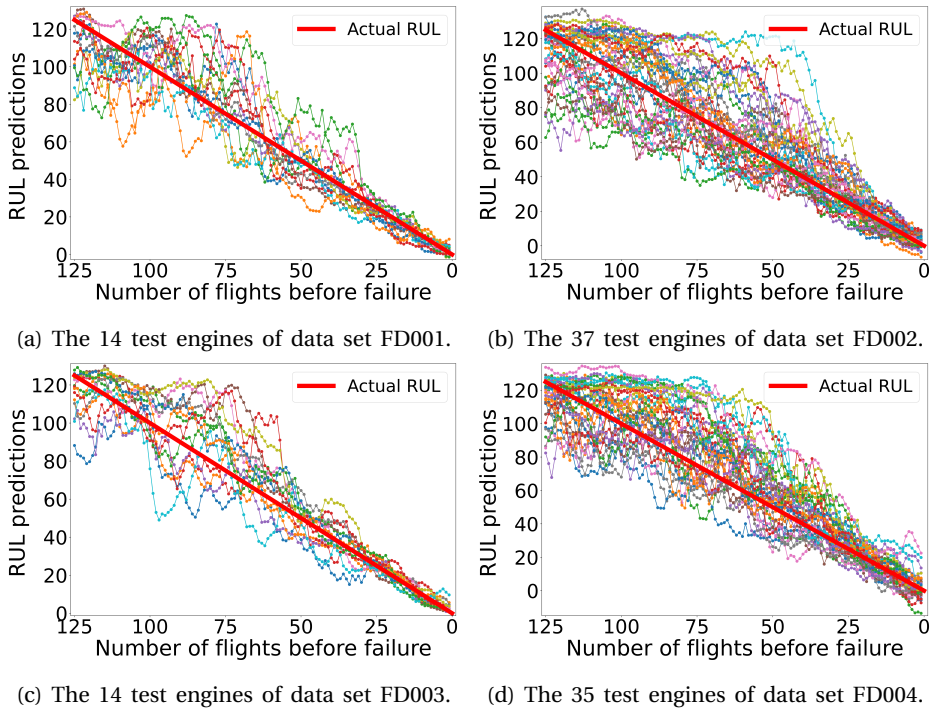
Figure 6.7.: RUL prognostics over time for the engines in E , split over the four C-MAPSS subsets.
