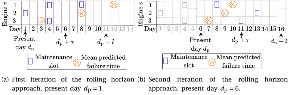
Figure 7.8.: Schematic example of two iterations of the rolling horizon approach, with |V| = 3 engines, \tau = 5 days, l = 10 days, and present days d_p = 1 and d_p = 6 .
