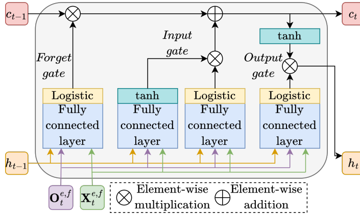
Figure 2.3.: A schematic overview of a LSTM-cell with informative operating conditions.
