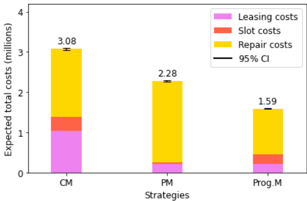
Figure 8.14.: The expected long-term maintenance costs of PM , CM and prognostics-based maintenance model ( Prog.M ) for a period of 60 months and a fleet of 13 wide-body aircraft, including 95% confidence intervals (CI).
