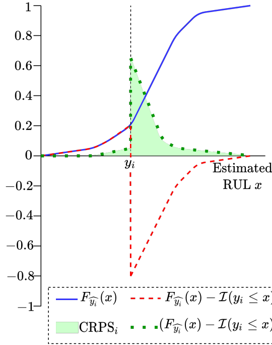
Figure 5.5.: Illustration of the CRPS_i metric for a single component i .
