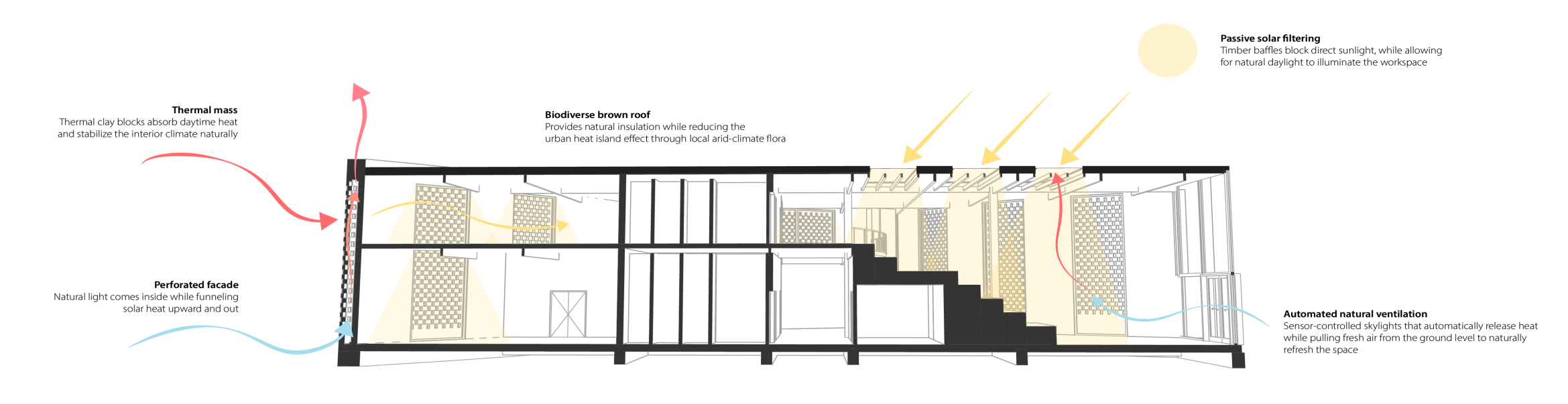
CLIMATE PRINCIPLES DIAGRAM
