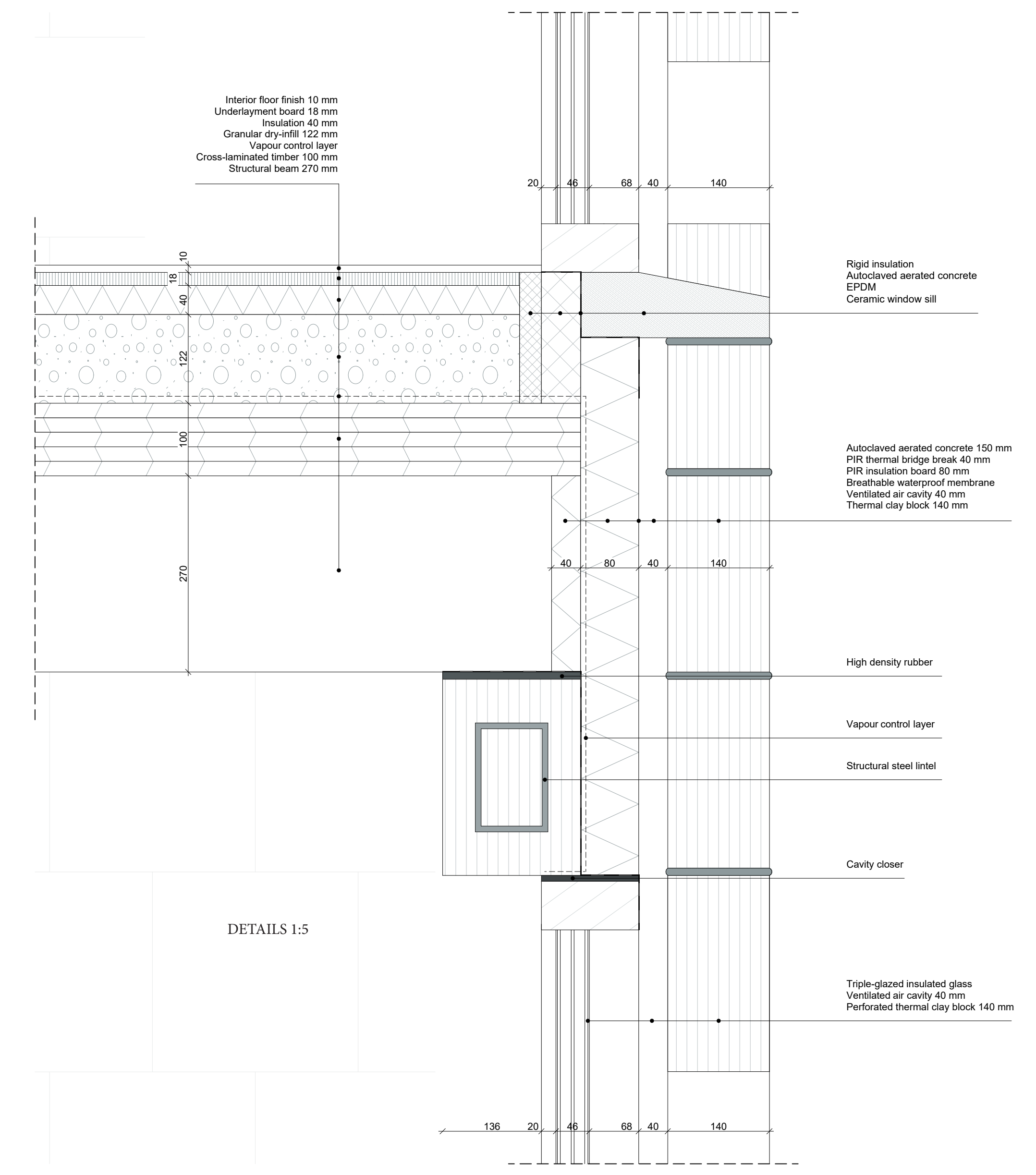
DETAILS 1:5
