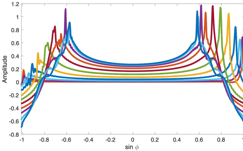
Figure 3.7 The negative power-flux normalized reflection coefficient curves at different, equally spaced lateral locations between 3566 m and 3941 m with a depth of 180 m in the velocity model. The curves closest to zero in amplitude is at 3566 m and the one furthest away is at 3941m in lateral distance. Note that the upper blue curve is the closest to the classical situation that involves two homogeneous half spaces, while the rest are in between this curve and the one with zero amplitude. Also note that not only the value at vertical incidence angle is different for each curve, but also at the other angles.
