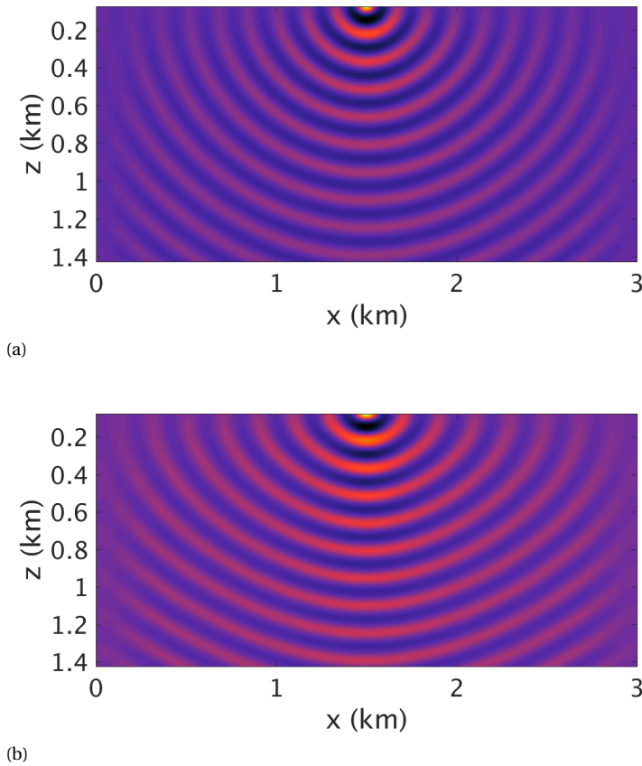
Figure 6.1 Monochromatic wavefield for a homogeneous isotropic model. (b) Monochromatic wavefield for a homogeneous anisotropic medium. Note how stretched the wavefield is in the horizontal and near vertical directions, as expected, compared to the isotropic case.
