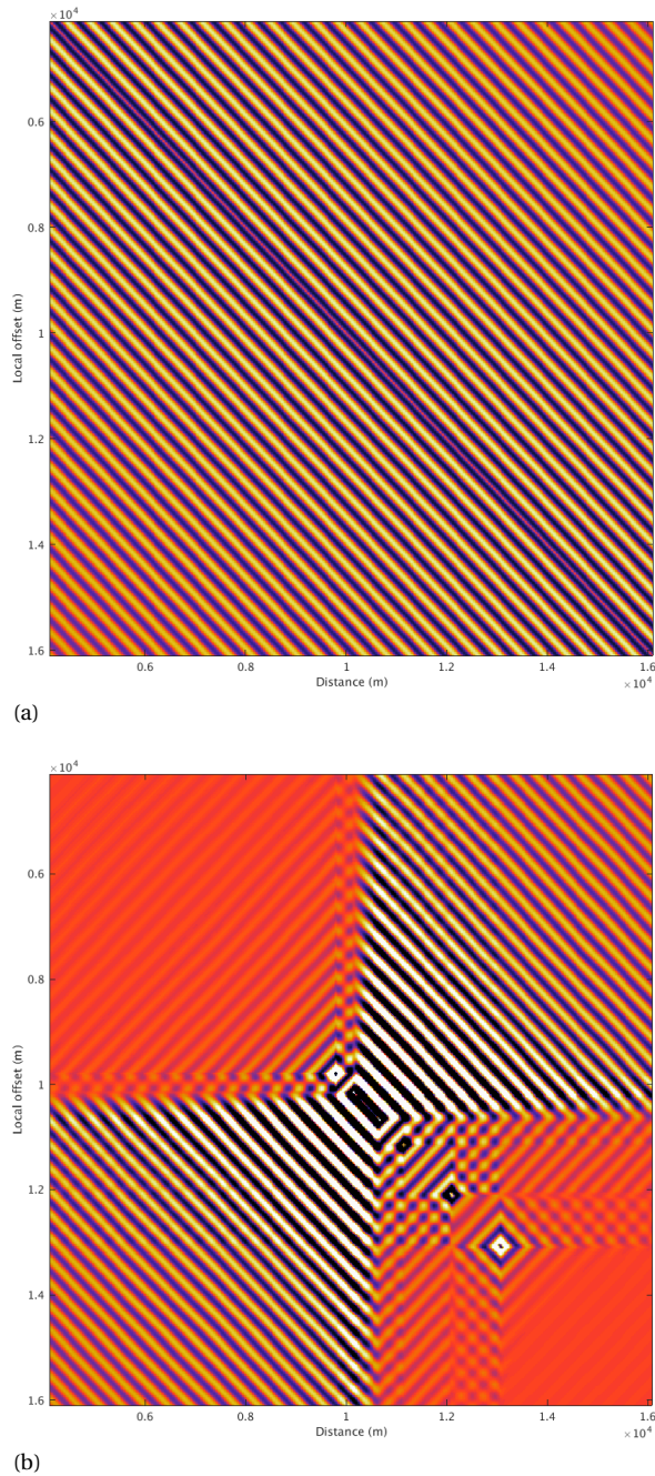
Figure 3.9 Monochromatic reflection and transmission operators for a frequency 8 Hz computed using a) the acoustic equivalent of Zoeppritz equations and b) using the fully inhomogeneous formulation.
