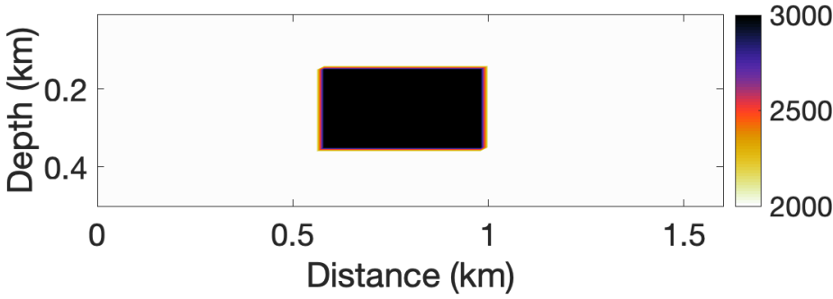
Figure 3.3 Velocity model with lateral heterogeneity used to demonstrate the difference between the formulation involving locally homogeneous media and that of generally heterogeneous media.
