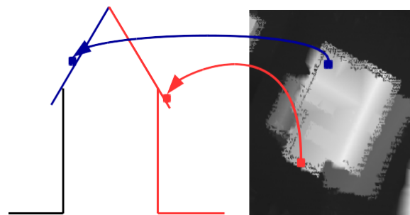
Figure 3. The red edge pixel from an overhanging roof may be interpolated from pixels from three different red planes, so three possible heights can be calculated from three red planes. The blue plane pixel from an interior roof plane is only related to the blue plane, so only one possible height is derived.
