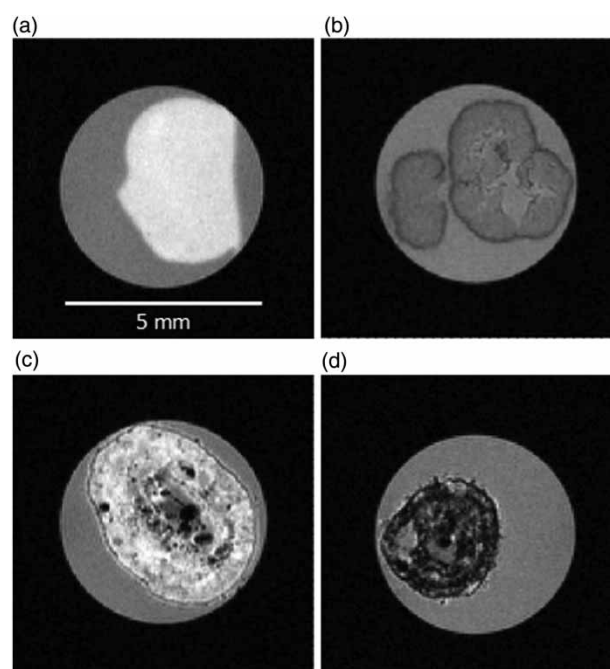
Figure 1 | T_1 -weighted images. Compared to the control EPS bead (a) and saline laboratory granule (b), aerobic granules collected from the PNU reactor (c) and Garmerwolde treatment plant (d) show a heterogeneous internal structure. Lighter regions correspond to regions with diffuse EPS while darker areas suggest denser or highly cross-linked EPS and cell clusters. Black regions indicate a lack of signal due to either a solid inclusion, or signal relaxation on the timescale of the measurement, i.e. faster than 5.3 ms (950 MHz, 47\ \mu\text{m} \times 47\ \mu\text{m} \times 100\ \mu\text{m} , t_E = 5.3\ \text{ms} , T_R = 550\ \text{ms} , 1st echo).
