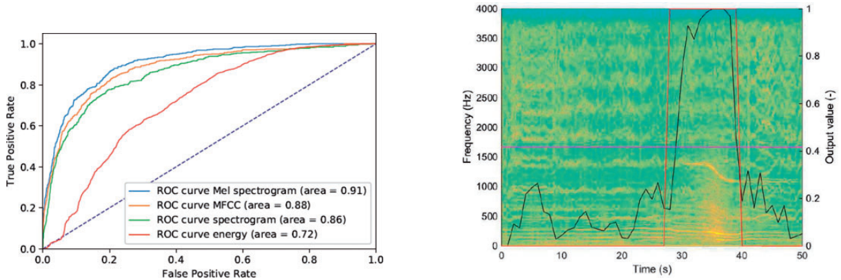
Figure 9. ROC curves of each feature for the basis run. Also the energy of the signal is used as an input for the ROC curve to show that the model does not base its output only on the energy in the signal. The Mel spectrogram is the best performing feature, MFCC second best, the spectrogram is the worst feature and energy performs significantly worse than all features.
