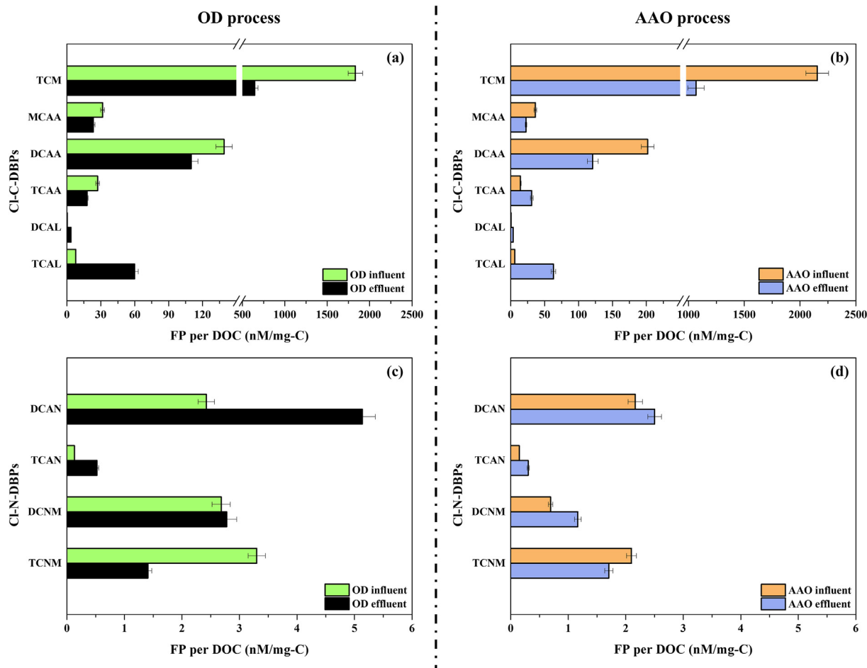
Fig. 4. Effect of OD and AAO processes on Cl-DBP formation reactivity. Experimental conditions: DOC = 2 mg/L, chlorine dose = 1.0–2.0 mg/L residual after 72 h reaction, T = 25 \pm 0.5 °C, pH = 7 \pm 0.2 .
