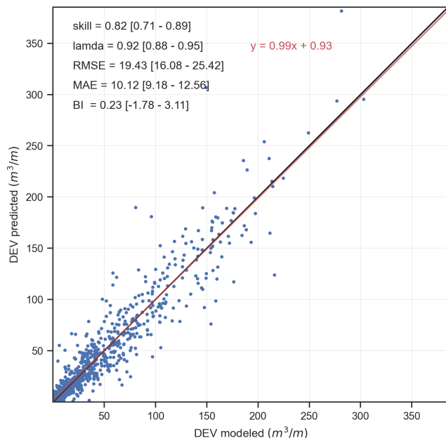
Figure 9. Scatterplot between the XBeach-simulated ( x axis) and ANN-predicted ( y axis) DEV for the validation cases with \text{DEV} > 0 \text{ m}^3 \text{ m}^{-1} using the selected regression ANN configuration (three hidden layers of 32 neurons each). The scatterplot shows the validation cases for one of the randomizations, while statistics in the upper left show the mean over the 10 randomizations of the benchmark cases, with brackets giving the min–max values. The black line indicates the 1 : 1 line, while the red line is the linear regression fit (equation given in red).
