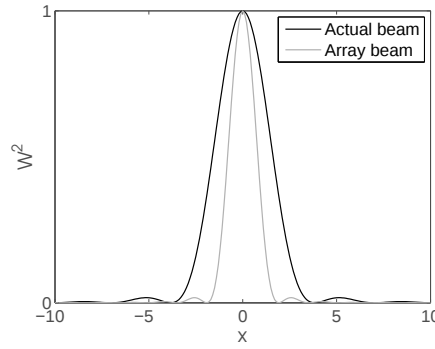
Figure 10: Cross-section of Figure 2 through (0,0) of Airy pattern for the maximum array aperture (array beam) and aperture typically encountered during the optimization (actual beam). Actual beams are always larger or equal to the array beam.
