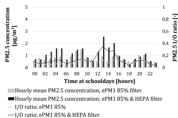
Fig. 10 - Continuous measurements comparing a classroom with an improved filter only and a classroom with an improved filter and HEPA filter.
