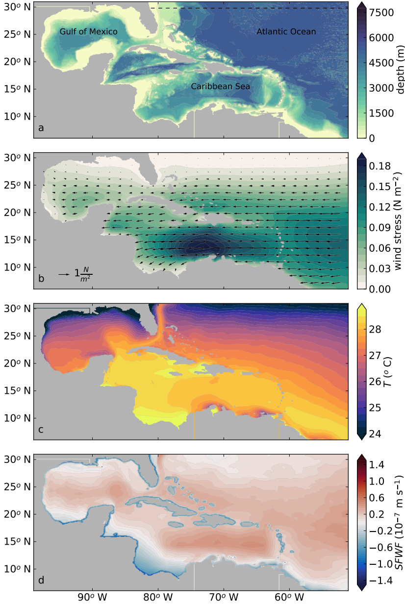
Figure 4.1: Setup of the regional model in MITgcm. (a) Bathymetry in m. The sponge layer is indicated with the dashed line. (b) Magnitude of the wind stress. The direction is indicated with the vectors. Not all velocity vectors are shown for clarity purposes. (c) Surface temperature field in ^{\circ}\text{C} used for restoring. (d) Surface fresh water flux in \text{m s}^{-1} . Positive values correspond to a net surface buoyancy loss.
