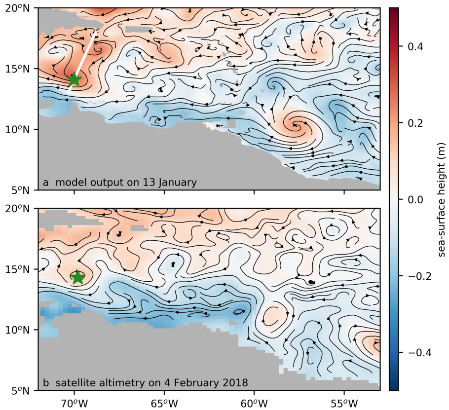
Figure 3.4: Sea-surface height (a) in the CS-nest simulation on 13 January and (b) from satellite altimetry on 4 February 2018. Streamlines of the flow are indicated with black curves. Green stars highlight the location of anticyclones discussed in Section 3.3.2. The white line indicates the location of the cross sections depicted in Fig. 3.5. The sea-surface height from satellite altimetry in (b) is computed from multi-mission altimeter satellite gridded sea-surface heights, downloaded from the Copernicus Marine Environment Monitoring Service ( http://marine.copernicus.eu ).
