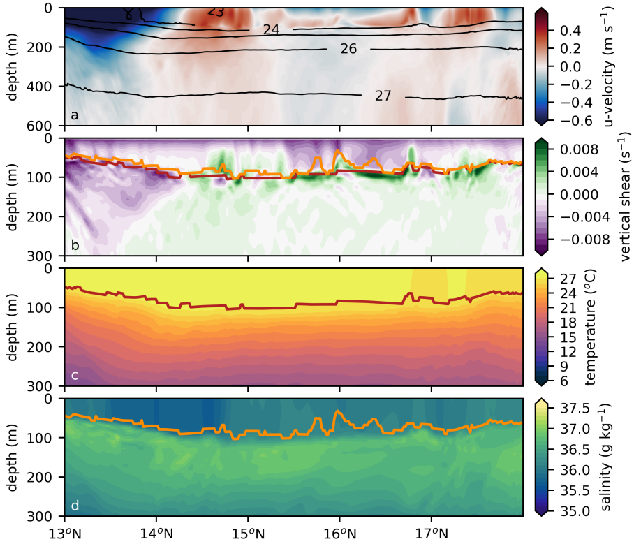
Figure 3.5: Characteristics of a modeled shallow anticyclone in the Caribbean Sea in winter, by means of cross sections of the (a) velocity perpendicular to the cross section ( \text{m s}^{-1} ), (b) vertical shear of this velocity ( \text{s}^{-1} ), (c) conservative temperature ( ^{\circ}\text{C} ) and (d) absolute salinity ( \text{g kg}^{-1} ) on 13 January. Contour lines in panel (a) show the isopycnals. The thermocline and halocline, indicated with the red and orange curve respectively, were computed following Mignot et al. (2012).
