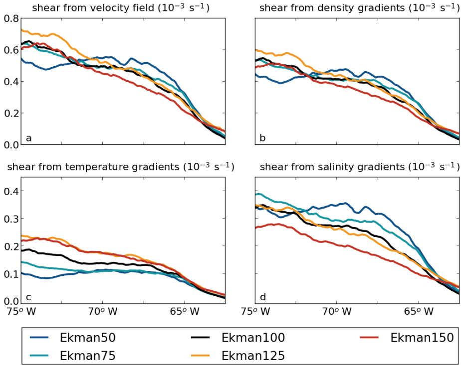
Figure 4.13: Zonal variation of the meridional average (12.5°N-17.5°N) of the (a) average vertical shear of the anticyclones, (b) horizontal density gradients, (c) horizontal density gradients induced by temperature gradients and (d) horizontal density gradients induced by salinity gradients. All properties are computed over the upper 50 m of the water column.
