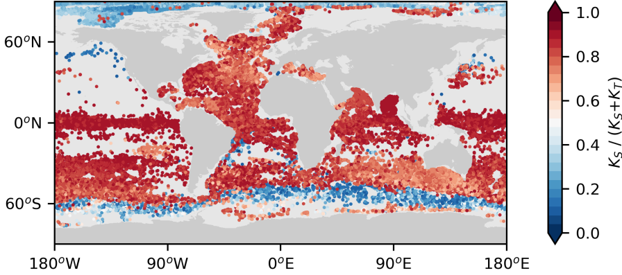
Figure 6.6: Relative magnitude of the effective diffusivity of salt compared to the combined effective diffusivities of heat and salt ( K_S / (K_S + K_T) ). Thermohaline staircases in the salt-finger regime ( K_S > K_T ) are denoted by red dots and thermohaline staircases in the diffusive convection regime ( K_T > K_S ) are denoted by blue dots
