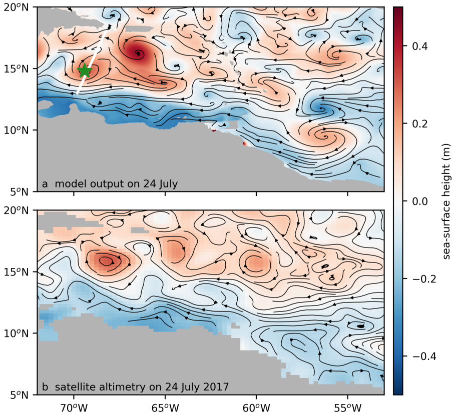
Figure 3.6: Sea-surface height (m) in the (a) CS-nest on 24 July of year 6 and (b) from satellite altimetry on 24 July 2017. Streamlines of the flow are indicated with black curves. The green star highlights the location of anticyclones discussed in Section 3.3.2. The white line indicates location of cross section of Fig. 3.7. The sea-surface height from satellite altimetry is computed from multi-mission altimeter satellite gridded sea-surface heights, downloaded from the Copernicus Marine Environment Monitoring Service ( http://marine.copernicus.eu ).
