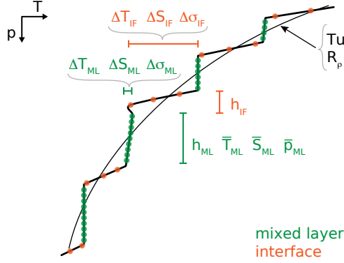
Figure 5.3: Schematic of a typical temperature profile with staircases, indicating the definitions of the quantities used to detect the thermohaline staircases (green: mixed layer; orange: interface). The overbar indicates layer-averaged properties.
