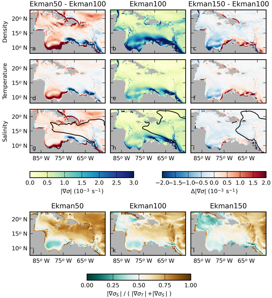
Figure 4.14: (a-c) Average strength of the horizontal density gradients ( |\nabla\sigma| ) in Ekman50, Ekman100, Ekman150 (see Section 4.2). The middle column shows the magnitude of the density gradients in Ekman100. Left and right columns contain the difference between Ekman50 and Ekman150 and Ekman100, respectively. Red colors indicate an increase of the horizontal density gradient. (d-f) Average strength of the horizontal density gradients due to temperature variations ( |\nabla\sigma_T| ). (g-i) Average strength of horizontal density gradients due to salinity variations ( |\nabla\sigma_S| ). The solid black line indicates where S = 35.5 psu. (j-l) Relative magnitude of density gradients due to salinity compared to density gradients due to temperature ( \frac{|\nabla\sigma_S|}{|\nabla\sigma_T| + |\nabla\sigma_S|} ). All properties are averaged over 20-years and over the upper 50 m of the water column.
