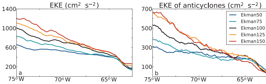
Figure 4.12: (a) Zonal variation of the maximum of EKE between 12.5°N-17.5°N, from 65°W to 75°W for each simulation. (b) As (a), but for the anticyclones with long tracks only. The EKE was averaged over the upper 50 m. Note the difference in scale between the two panels.
