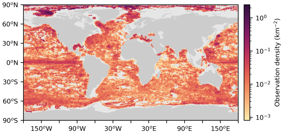
Figure 5.2: Observation density of the number of profiles obtained from the Argo floats and Ice-Tethered Profilers after quality control (in \text{km}^{-2} ). Observation density is binned per degree longitude and degree latitude. Empty bins indicate that no data was available at that location.
