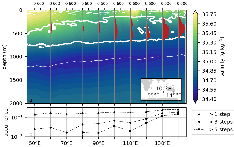
Figure 6.5: Thermohaline staircases in the southern Indian Ocean. (a) Red histograms show the vertical distribution of number of detected mixed layers in thermohaline staircases per 10 degrees longitude. The thick (thin) white contour corresponds to Turner angles (Ruddick, 1983) of Tu = 71.6^\circ ( Tu = 45^\circ ), indicating the susceptibility of the water column to double diffusion in the salt-finger regime ( 45^\circ < Tu < 90^\circ ). Background shading indicates the mean vertical salinity profile obtained from the World Ocean Atlas 2018 (Zweng et al., 2019). The inlay shows the considered region: 45^\circ\text{E} - 145^\circ\text{E} , 32^\circ\text{S} - 42^\circ\text{S} . (b) Occurrence of number of steps per profile in per 10 degrees longitude (note the logarithmic vertical axis).
