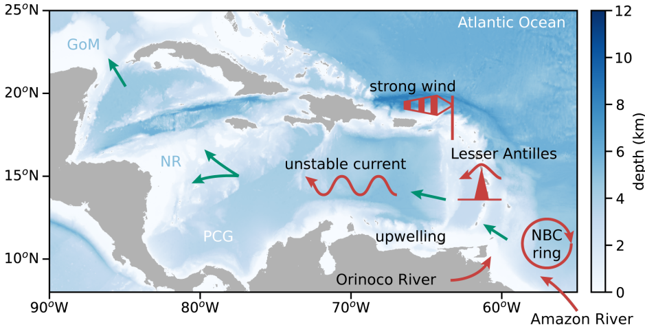
Figure 1.5: Bathymetry of the Caribbean Sea. The green arrows indicate the direction of the mean surface currents. The red icons show the mechanisms that have been suggested as potential formation mechanisms of Caribbean anticyclones. NR = Nicaraguan Rise, GoM = Gulf of Mexico, PCG = Panama Colombia Gyre
