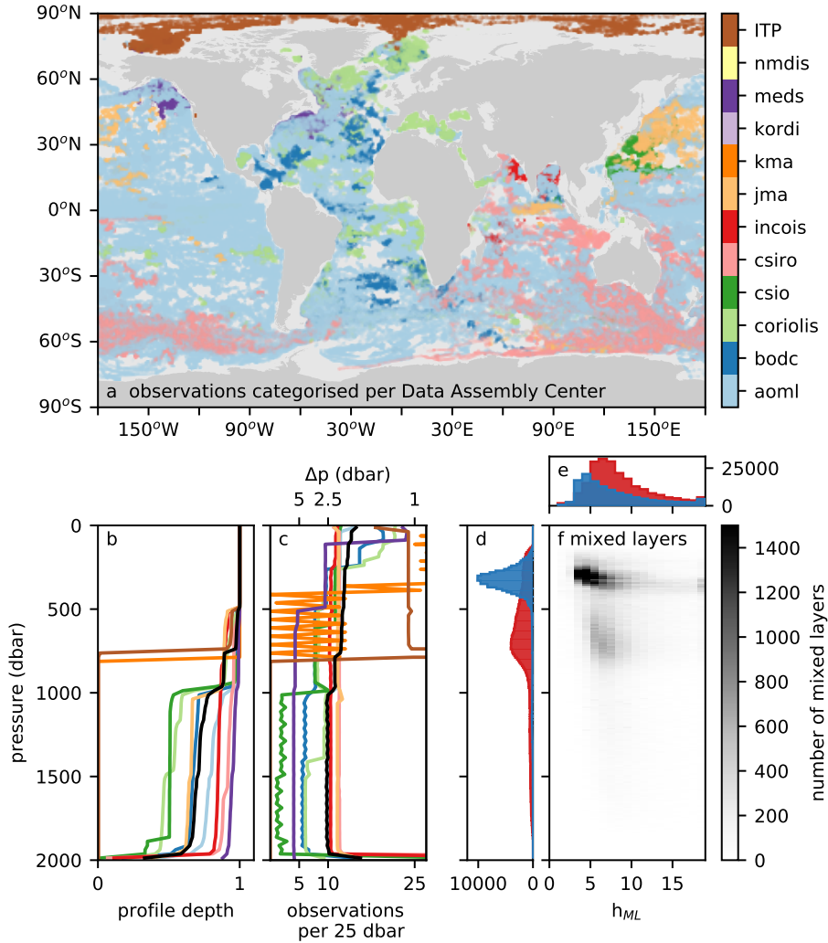
Figure 5.1: (a) Locations of observations categorized by Data Assembly Centers (DAC) when obtained by an Argo float. Profiles obtained with Ice-Tethered Profilers are indicated with ITP (b) Cumulative fraction of profiles that reached a given pressure in 25-dbar intervals from 0 to 2,000 dbar per DAC. (c) Average number of observations in 25-dbar intervals from 0 to 2,000 dbar. (d) Distribution of detected mixed layer pressures in the salt-finger (red histogram) or diffusive-convective (blue histogram) regime. (e) Number of detected mixed layers height in the salt-finger (red histogram) or diffusive-convective (blue histogram) regime. (f) Distribution of detected mixed layer heights in thermohaline staircases per pressure level. Panels (b) and (c) were obtained following Wong et al. (2020). Black lines indicate the averages in total global dataset. More details on abbreviations of DAC can be found in Argo (2019)
