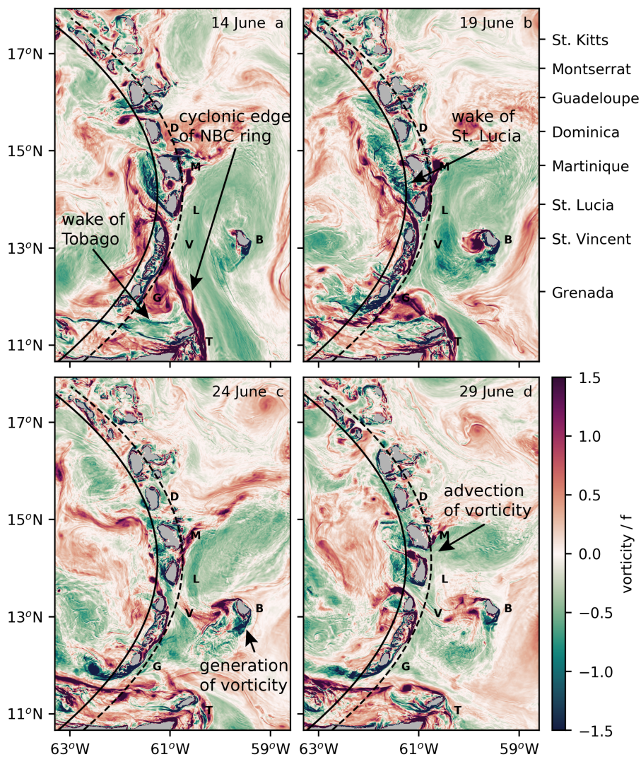
Figure 3.13: Similar as Figure 3.12, but then for the LA-nest simulation on (a) 14 June, (b) 19 June, (c) 24 June, (d) 29 June.
