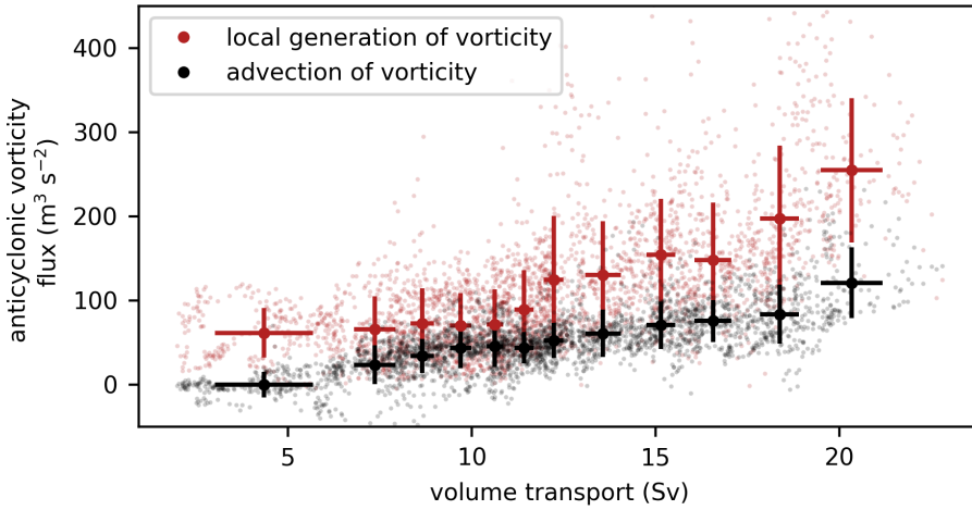
Figure 3.11: Relation between the total volume transport and the anticyclonic vorticity flux into the Caribbean Sea, distinguishing the local generation of vorticity (red symbols) and the advection of vorticity from the Atlantic Ocean (black dots). The local generation of vorticity is defined as the difference between the 6-hourly snapshots of the vorticity flux west and east of the Lesser Antilles (similar to grey shading in Fig. 3.10b). The advection of vorticity corresponds to the anticyclonic vorticity flux east of the Lesser Antilles (similar to Fig. 3.10b). The thick dots indicate average values per 250 data points, where the error bars correspond to one standard deviation.
