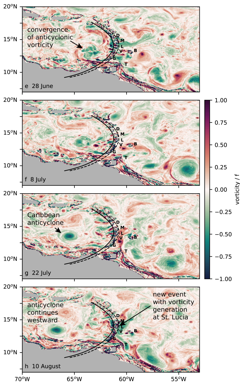
Figure 3.12: (continued) (e) 28 June, (f) 8 July, (g) 22 July, (h) 10 August.
