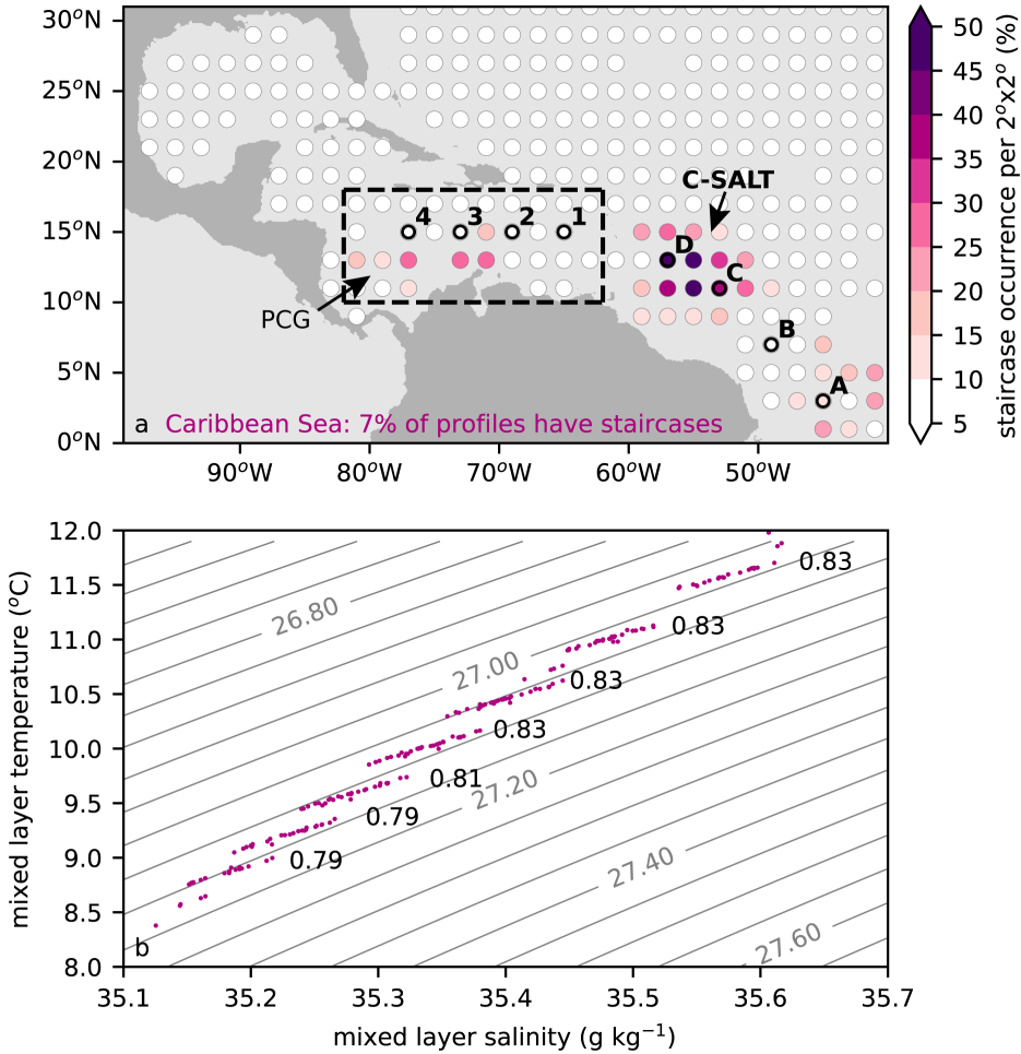
Figure 7.3: (a) Occurrence of thermohaline staircases in the Caribbean Sea and North Atlantic Ocean averaged per 2^\circ \times 2^\circ and obtained from a global dataset of thermohaline staircases (Chapter 5 of this thesis). Only data points containing more than 10 observations are shown. Dashed box ( 62^\circ\text{W} – 82^\circ\text{W} and 10^\circ\text{N} – 18^\circ\text{N} ) is used to compute the occurrence of staircases in the Caribbean Sea. Numbers 1–4 and Letters A–D indicate the same locations as in Fig. 7.1. (b) Temperature and salinity in the thermohaline staircases with more than 4 steps in the Caribbean Sea (dashed box in panel a); grey contour lines highlight the isopycnals ( \sigma_0 ). Numbers indicate the slope the aligned points, corresponding to the lateral density ratio ( R_{\rho} ) and are approximately equal to flux ratio ( \gamma ). The locations of the Panama Colombia Gyre (PCG) and C-SALT and indicated in panel (a).
