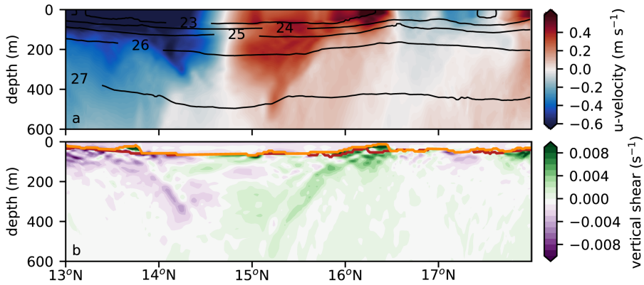
Figure 3.7: Characteristics of a modeled deep anticyclone in summer, by means of cross sections of the (a) u-component of the velocity ( \text{m s}^{-1} ), (b) vertical shear of the u-component of the velocity ( \text{s}^{-1} ), taken at the location indicated in Fig. 3.6 on 24 July year 6. Contour lines in panel (a) show the isopycnals. The thermocline and halocline, indicated with the red and orange line respectively, were computed following Mignot et al. (2012). Note that the vertical axis of panel (b) extends deeper than the one in Figure 3.5b.
