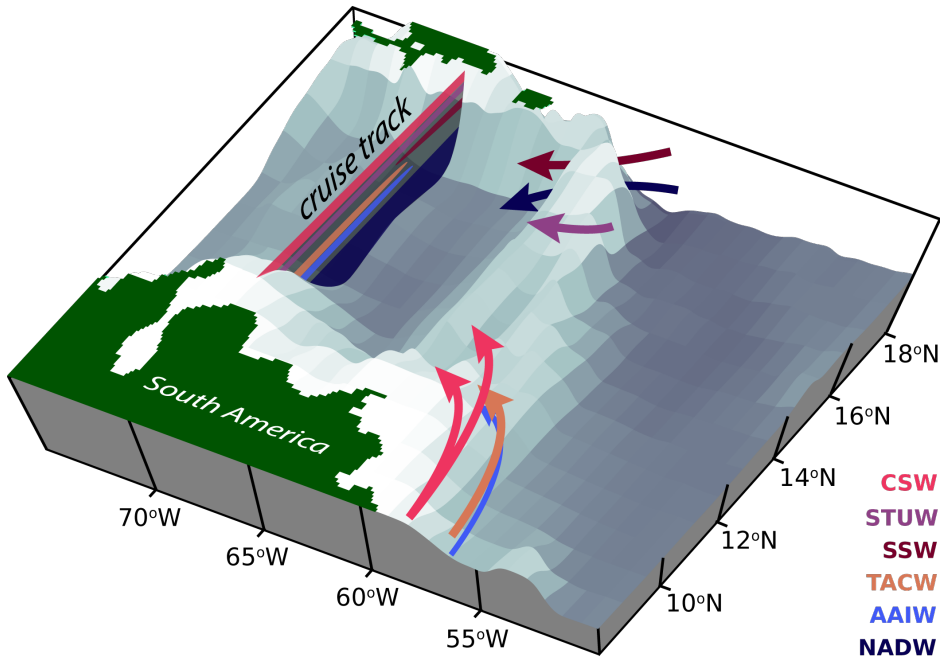
Figure 1.4: 3D Schematic of how water masses enter the eastern Caribbean Sea. Indicated water masses are AAIW = Antarctic Intermediate Water, CSW = Caribbean Surface Water, NADW = North Atlantic Deep Water, SSW = Sargasso Sea Water, STUW = Subtropical Underwater, TACW = Tropical Atlantic Central Water.
