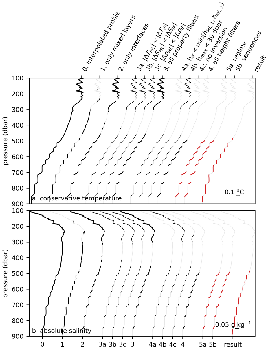
Supplementary Figure 5.10: as Supplementary Figure 5.9, but for a profile in the Mediterranean Sea. Original profile is taken from Argo float 6901769 at 8.9^\circ\text{E} and 37.9^\circ\text{N} on 31 October 2017.
