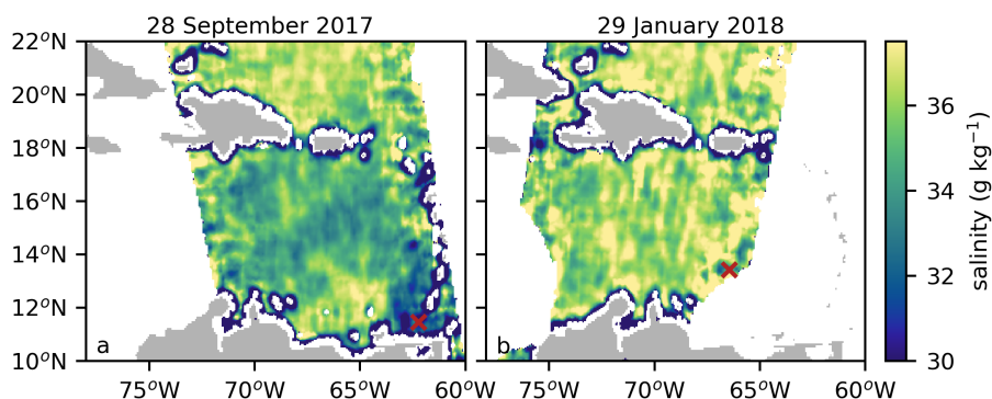
Figure 2.4: Sea-surface salinity from the 'Soil Moisture and Ocean Salinity' satellite at (a) 28 September 2017 and (b) 29 January 2018. The approximate formation region of the anticyclone is indicated with the red cross. The location of the anticyclone at 29 January 2018 was obtained from satellite altimetry with the py-eddy tracker and is indicated with the red cross.
