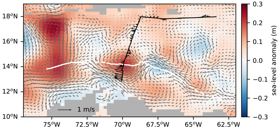
Figure 2.2: Gridded sea-level anomaly (m) on 5 February 2018 with the geostrophic surface velocities (grey vectors) obtained from gridded altimetry from E.U. Copernicus Marine Service Information. The cruise track is indicated by the solid black line. The black arrows show the velocities of the ADCP averaged over the upper 25-35 m (below the blanking distance). The white line indicates the track of the anticyclone.
