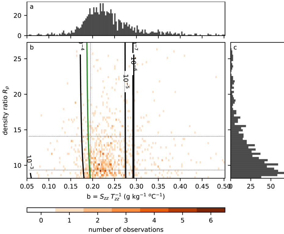
Figure 7.4: (a) Histogram of values of b obtained from observations from Argo floats profiles between 600 and 750 dbar. (b) Effective diffusivity of salt ( K_S ) as a function of b and R_\rho . The green line corresponds to observations of (Schmitt, 2005). The orange shading shows the number of observations with values of b and R_\rho . (c) Histogram of values of the density ratio, R_\rho , obtained from Argo floats profiles between 600 and 750 dbar. Dashed lines in panel (b) indicated the 25th and 75th percentile of the values in panels (a) and (c). The ranges of the axes in panels (a) and (c) correspond to the 5th and 95th percentile of the observed values of b and R_\rho . Details on the computations of R_\rho , K_S , and b can be found in the Section 7.A
