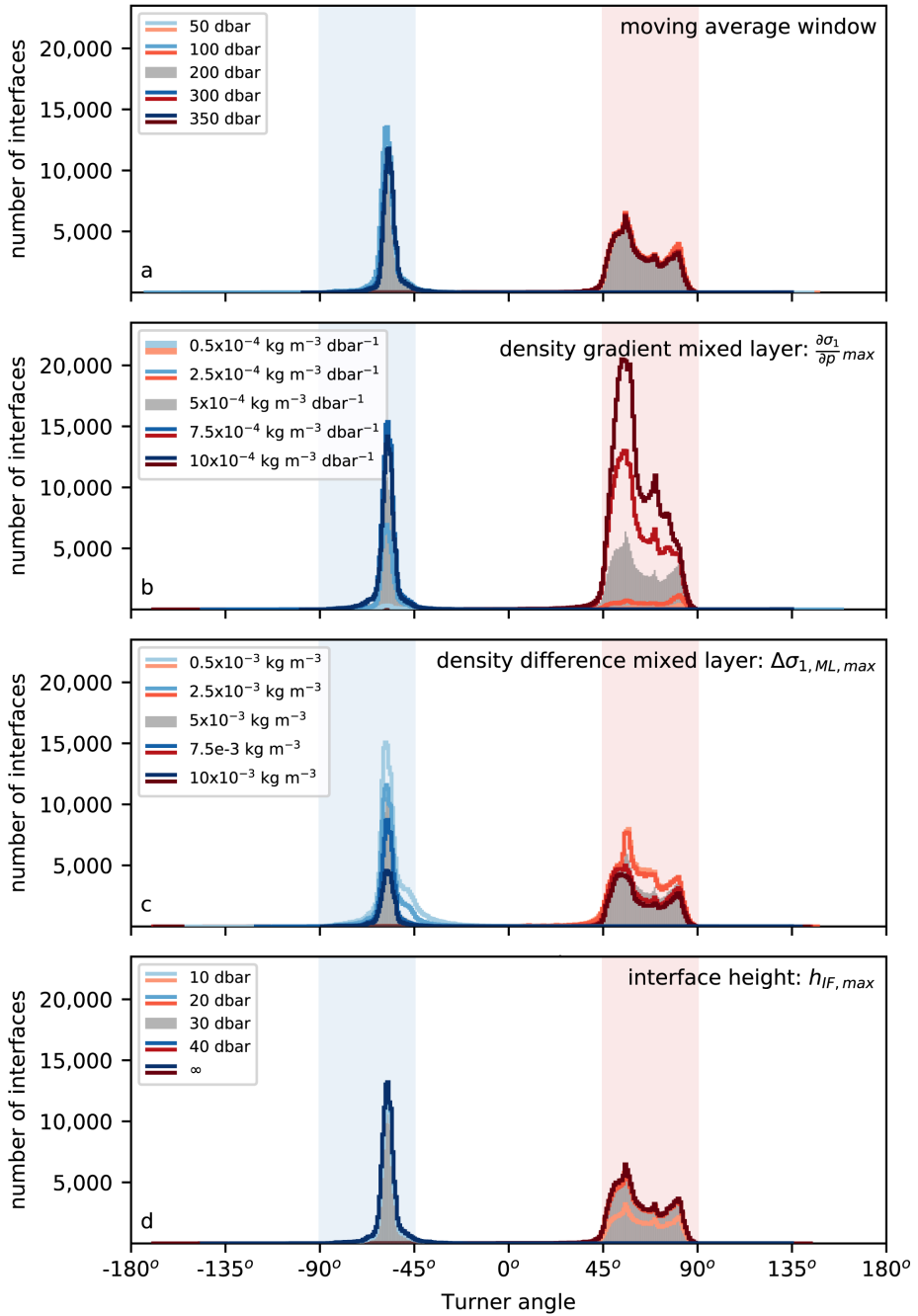
Figure 5.8: Number of detected interfaces obtained with the detection algorithm for different input parameters. Each sub-panel shows the sensitivity of the algorithm to one input parameter: (a) moving average window, (b) density gradient of the mixed layer, (c) density difference within the mixed layer and (d) the maximum height of the interface. The grey histograms correspond to the default parameters (Table 5.2). The colored lines correspond to the varying parameter. Shaded regions indicate Turner angles in the diffusive-convective (blue) and salt-finger (red) regime.
