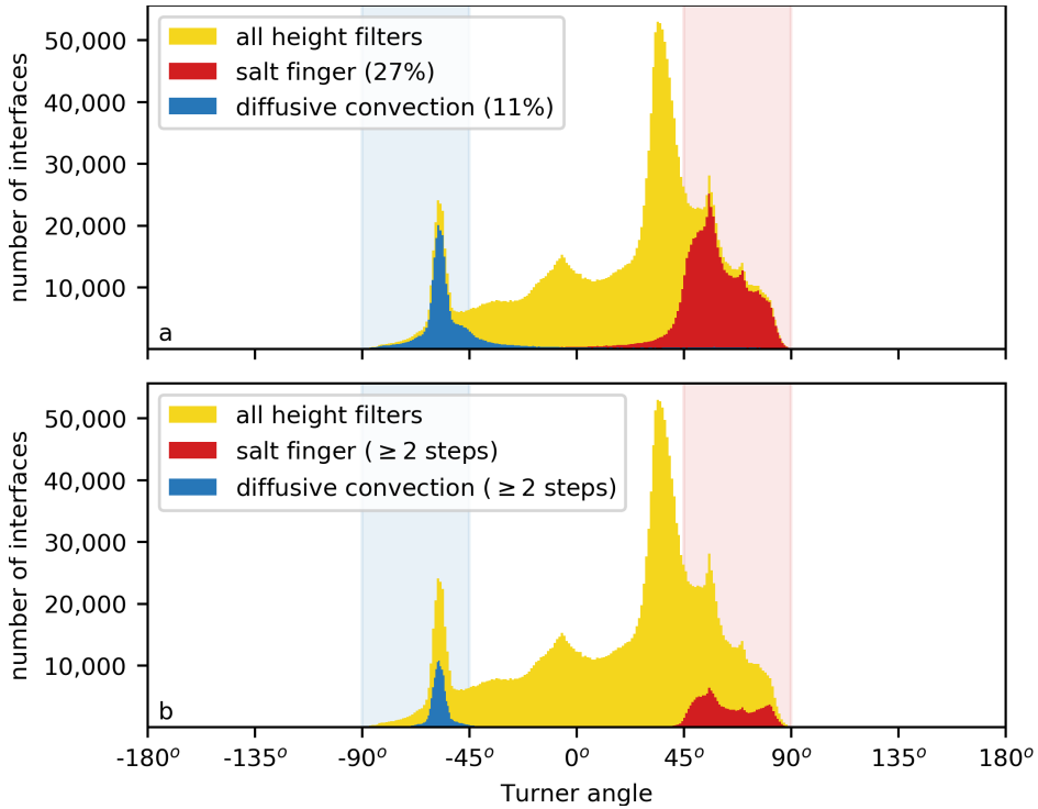
Figure 5.6: Histogram of the number of detected interfaces as a function of the Turner angle (Tu) after (a) classification of the double-diffusive regime and (b) selection of sequences of the interfaces. Each panel shows the data remaining compared to the interfaces detected based on interface height requirement shown in Fig. 5.5d (yellow shading). Vertical shaded bands correspond to Turner angles in the diffusive-convective (blue) and salt-finger (red) regime.
