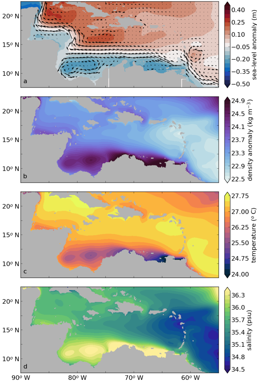
Figure 4.3: 20-year near-surface average properties of the Caribbean Sea in Ekman100. (a) Mean sea-level anomaly (SLA) in m with velocity vectors. Surface current vectors are only shown every eighth grid cells for clarity purposes. (b) Density ( \sigma = \rho - 1000 ) in \text{kg m}^{-3} , (c) Temperature in ^{\circ}\text{C} and (d) Salinity in psu. Properties in panel b-c-d are averages over the upper 50 m.
