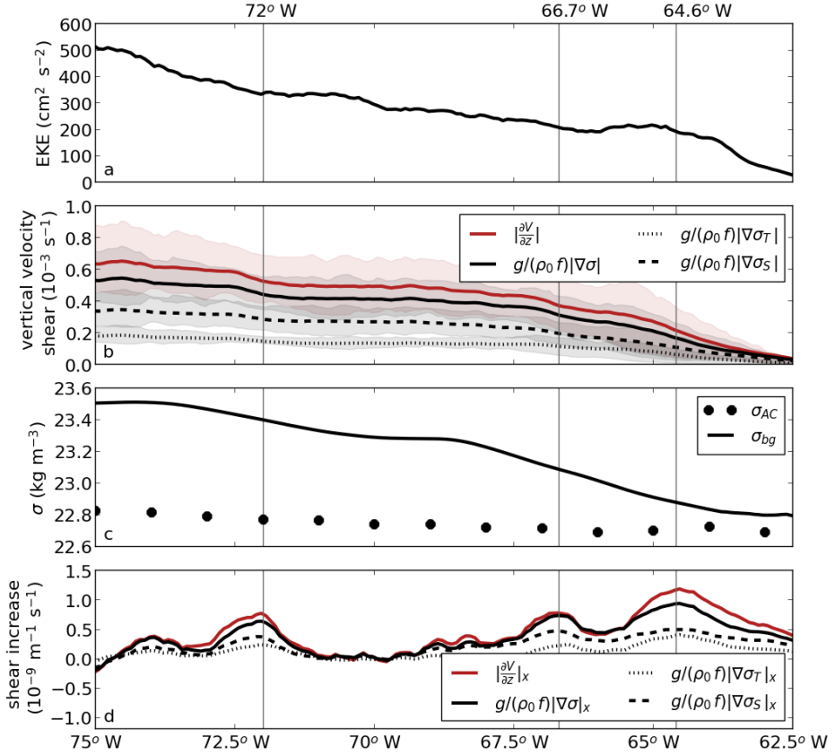
Figure 4.8: (a) Zonal variation of the (a) meridional maximum eddy kinetic energy, and (b) vertical velocity shear and shear computed from horizontal density gradients between 12.5°N and 17.5°N of the anticyclones with long tracks. The shaded regions indicate the 25th and 75th percentile. All properties are averaged over the upper 50 m of the water column. (c) Density anomaly of the background ( \sigma_{bg} ) and anticyclones ( \sigma_{AC} ), averaged over the upper 50 m. The density anomaly of the anticyclones is averaged per degree longitude. (d) The variations of vertical shear and horizontal density gradients with longitude in westward direction of the anticyclones with long tracks.
