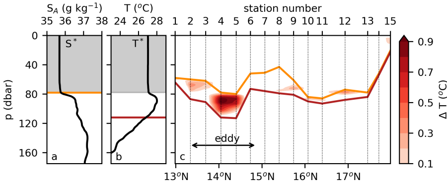
Figure 2.6: (a) Absolute salinity profile of the upper 180 dbar of the water column at station 4. The orange solid line shows the depth of the halocline at that location. The grey shaded area indicates the depth over which the mixed layer salinity ( S^* ) is determined. (b) Conservative temperature profile at station 4. The red solid line shows the depth of the thermocline, which was defined as the depth where the temperature decreased with 0.2\text{ }^{\circ}\text{C} compared to the temperature of the mixed layer. The grey shaded area indicates the depth over which the mixed layer temperature ( T^* ) is determined. (c) Magnitude of the temperature inversion, defined as the temperature of the barrier layer minus the temperature of the mixed layer along the hydrographic section. The depth of the halocline and thermocline are indicated by the orange and red lines, respectively.
