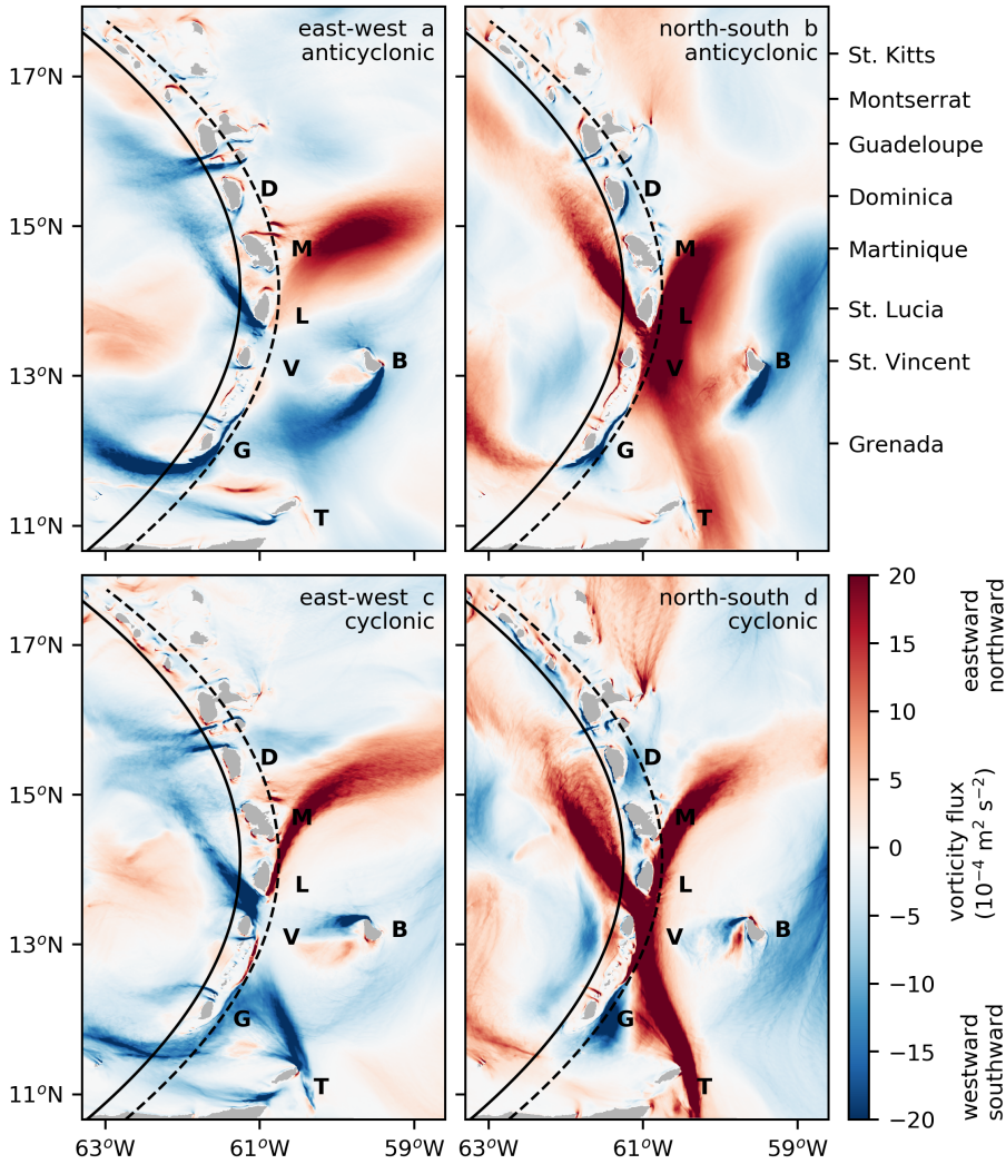
Figure 3.14: Directional vorticity flux integrated over the upper 300 m of the water column and averaged between 3 June and 28 June ( LA-nest ). (a,b) Anticyclonic vorticity flux in (a) eastward and (b) northward direction; (c,d) Cyclonic vorticity flux in (c) eastward and (d) northward direction. Dashed and solid lines indicate the locations of the cross sections east and west of the Lesser Antilles, respectively. Letters are placed east of the islands to indicate their location: D = Dominica, M = Martinique, L = St. Lucia, V = St. Vincent, G = Grenada, T = Tobago, B = Barbados.
