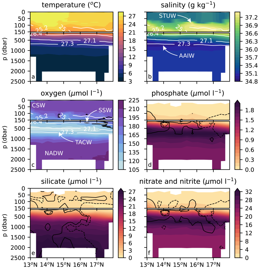
Supplementary Figure 2.9: Section of conservative temperature ( T ), absolute salinity ( S_A ), oxygen ( O_2 ), phosphate ( PO_4 ), silicate ( Si ) and combined nitrate and nitrite ( NO_3 + NO_2 ) along the cruise track. Indicated water masses are AAIW = Antarctic Intermediate Water, CSW = Caribbean Surface Water, NADW = North Atlantic Deep Water, SSW = Sargasso Sea Water, STUW = Subtropical Underwater, TACW = Tropical Atlantic Central Water. The white contour line indicate the isopycnals in the core of a water mass. The black contour lines show positive (solid) and negative (dashed) anomalies from the depth-averaged mean for O_2 (contour drawn at 15 \mu\text{mol l}^{-1} ), PO_4 (contour drawn at -0.05 and 0.05 \mu\text{mol l}^{-1} ), Si (contour drawn at -0.2 and 0.2 \mu\text{mol l}^{-1} ) and NO_3 + NO_2 (contour drawn at -0.5 and 0.5 \mu\text{mol l}^{-1} )
