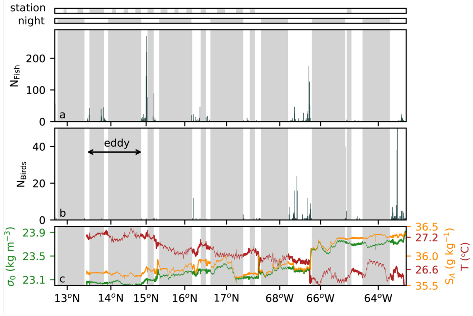
Figure 2.8: (a) Number of flying fish ( N_{\text{Fish}} ) observed along the track per 10-minute count. (b) Number of birds ( N_{\text{Birds}} ) observed per 10-minute count. (c) Surface temperature ( T ), salinity ( S_A ) and density anomaly ( \sigma_0 ) as observed with the ship-board thermo-salinograph. The shaded grey regions indicate locations without observations during stations (top bar) and during nights (2nd bar). These periods without observations are also indicated by the shaded grey in panels a, b and c. The dark grey solid line distinguishes the first part of the track (northward; hydrographic survey) from the second part (eastward en route to St. Maarten).
