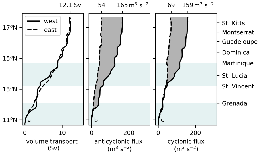
Figure 3.9: Total (a) volume transport (b) anticyclonic vorticity flux and (c) cyclonic vorticity flux at the Lesser Antilles integrated along the eastern (dashed lines) and western (black solid line) cross section (Fig. 3.1) integrated over the upper 300 m of the water column. The grey shaded area indicates the generation of vorticity between the cross sections. (d) Maximum sea-level anomaly between Barbados and Tobago along the yellow curve in Fig. 3.8. The blue shading indicates the collision of an NBC ring with the Lesser Antilles that is described in Section 3.6. The data is smoothed with a Hanning function with a window of 30 days. 5 October and 19 June indicate the times of minimum and maximum volume transport through the Lesser Antilles.
