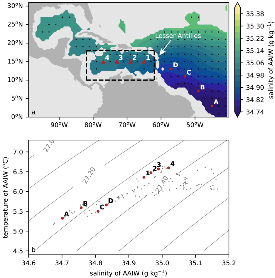
Figure 7.1: (a) Salinity of the AAIW core obtained from MIMOC (Schmidt et al., 2013). The dashed box (62°W–82°W and 10°N–18°N) is used to compute properties of AAIW in the Caribbean Sea. (b) Conservative temperature and absolute salinity of AAIW core averaged per 2°x2°. Location of the data points are indicated with black dots in panel (a). Grey contours highlight the isopycnals ( \sigma_0 ). Letters A–D correspond to the path of AAIW in the Atlantic Ocean; Numbers 1–4 correspond to the path of AAIW in the Caribbean Sea.
