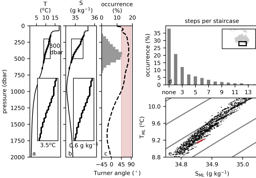
Figure 6.4: Properties of thermohaline staircases in the Great Australian Bight (32°S-42°S, 125°E-145°E). (a) Example temperature and (b) salinity profile with a thermohaline staircase obtained by an Argo float (float-id: 5905189) at 37.6°S, 135.1°E on 8 April 2019. The inlays show a zoom of the profiles between 200 and 500 dbar. (c) Distribution of mixed layers over depth (grey bars) and the average Turner angle (Ruddick, 1983) in the Great Australian Bight (dashed line). The red shading indicates Turner angles corresponding to the salt-finger regime ( 45^\circ < Tu < 90^\circ ). (d) Distribution of number of steps per profile in percentage. (e) Scatter plot of the temperature and salinity of the mixed layers of the detected staircases, where red dots indicate mixed layers that are used to compute the lateral coherence. Data in panels (c), (d) and (e) is obtained between 23 April 2007 and 13 May 2020. Inlay in (d) shows the considered region.
