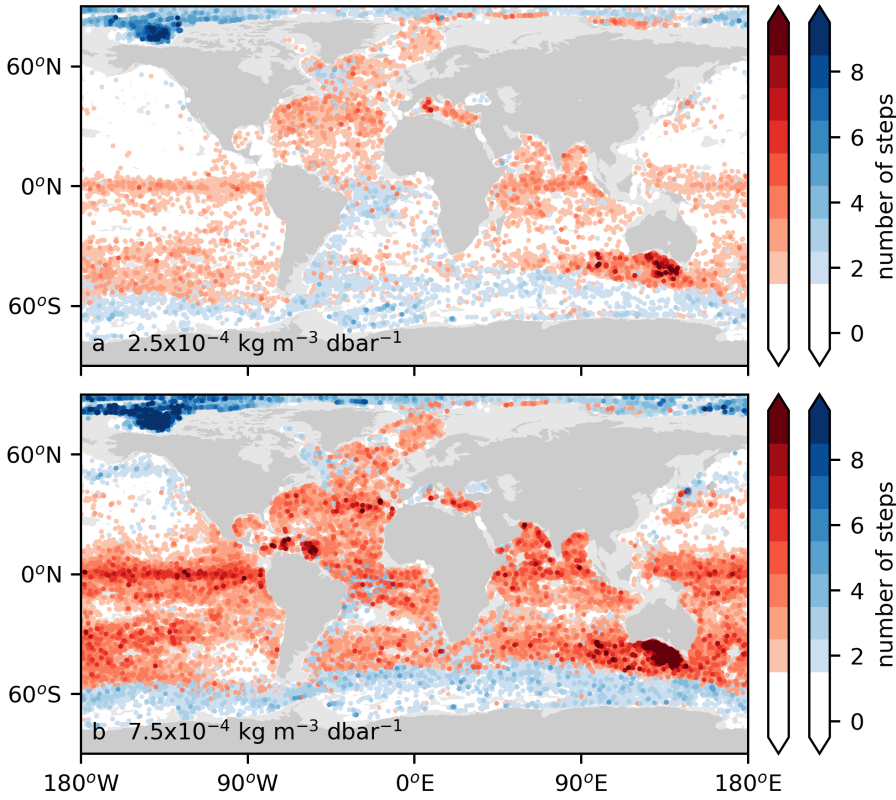
Figure 6.1: Sensitivity of the number of staircases detected resulting for different input parameters of the staircase detection algorithm (Chapter 5 of this thesis). (a) \partial \sigma_1 / \partial p_{\max} = 2.5 \times 10^{-4} \text{ kg m}^{-3} \text{ dbar}^{-1} (b) \partial \sigma_1 / \partial p_{\max} = 7.5 \times 10^{-4} \text{ kg m}^{-3} \text{ dbar}^{-1} . For each profile, the number of steps per staircase in the salt-finger regime (red dots) and diffusive-convective regime (blue dots) is plotted. Profiles with the largest numbers are plotted last for clarity. Figure 6.2 shows the same for the standard value of \partial \sigma_1 / \partial p_{\max} = 5.0 \times 10^{-4} \text{ kg m}^{-3} \text{ dbar}^{-1}
