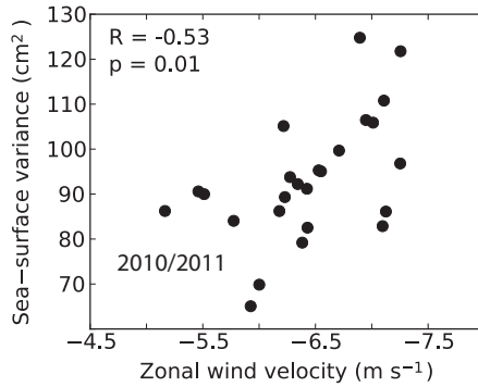
Figure 4.15: Year-averaged sea-level variance and coastal zonal wind velocities. Sea-surface spatial variance is obtained from daily sea-level anomaly fields from years 1993-2017 from satellite altimetry (CMEMS) and averaged over the interior of the Caribbean Sea (12.5°N - 17.5°N, 65°W - 75°W). Coastal zonal winds in the upwelling region (10°N -12.5°N, 65°W - 75°W) are obtained from years 1993-2017 from ECMWF (ERA-Interim, Dee et al., 2011). Each dot represents one year.
