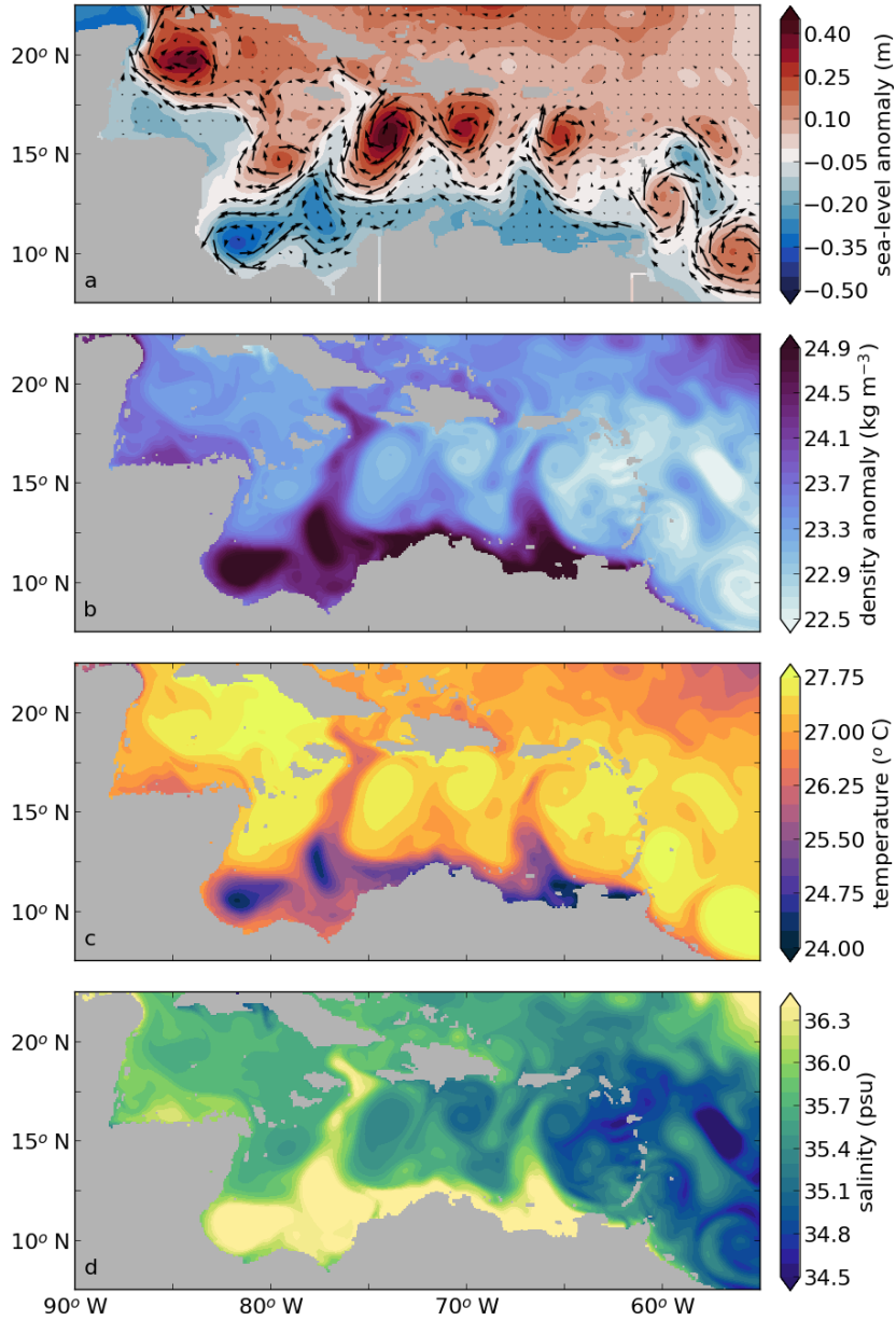
Figure 4.5: Near-surface properties of the Caribbean Sea, averaged over a 5-day period during the final year of the simulation Ekman100. (a) Mean sea-level anomaly (SLA, in m) with velocity vectors. Surface current vectors are only shown every eighth grid cells for clarity purposes. (b) Density ( \sigma = \rho - 1000 ) in \text{kg m}^{-3} , (c) Temperature in ^{\circ}\text{C} and (d) salinity in psu. Properties in panels are averages over the upper 50 m.
