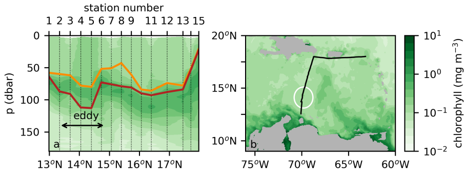
Figure 2.5: (a) Chlorophyll-a fluorescence concentrations ( \text{mg m}^{-3} ) along the hydrographic section. The thermocline and halocline, indicated with the red and orange lines respectively, were computed following Mignot et al. (2012). (b) Surface chlorophyll concentrations from merged satellite products at 5 February 2018 obtained from E.U. Copernicus Marine Service Information. The cruise track is shown by the black line and the location of the eddy is indicated by the white circle. Note the logarithmic color scale.
