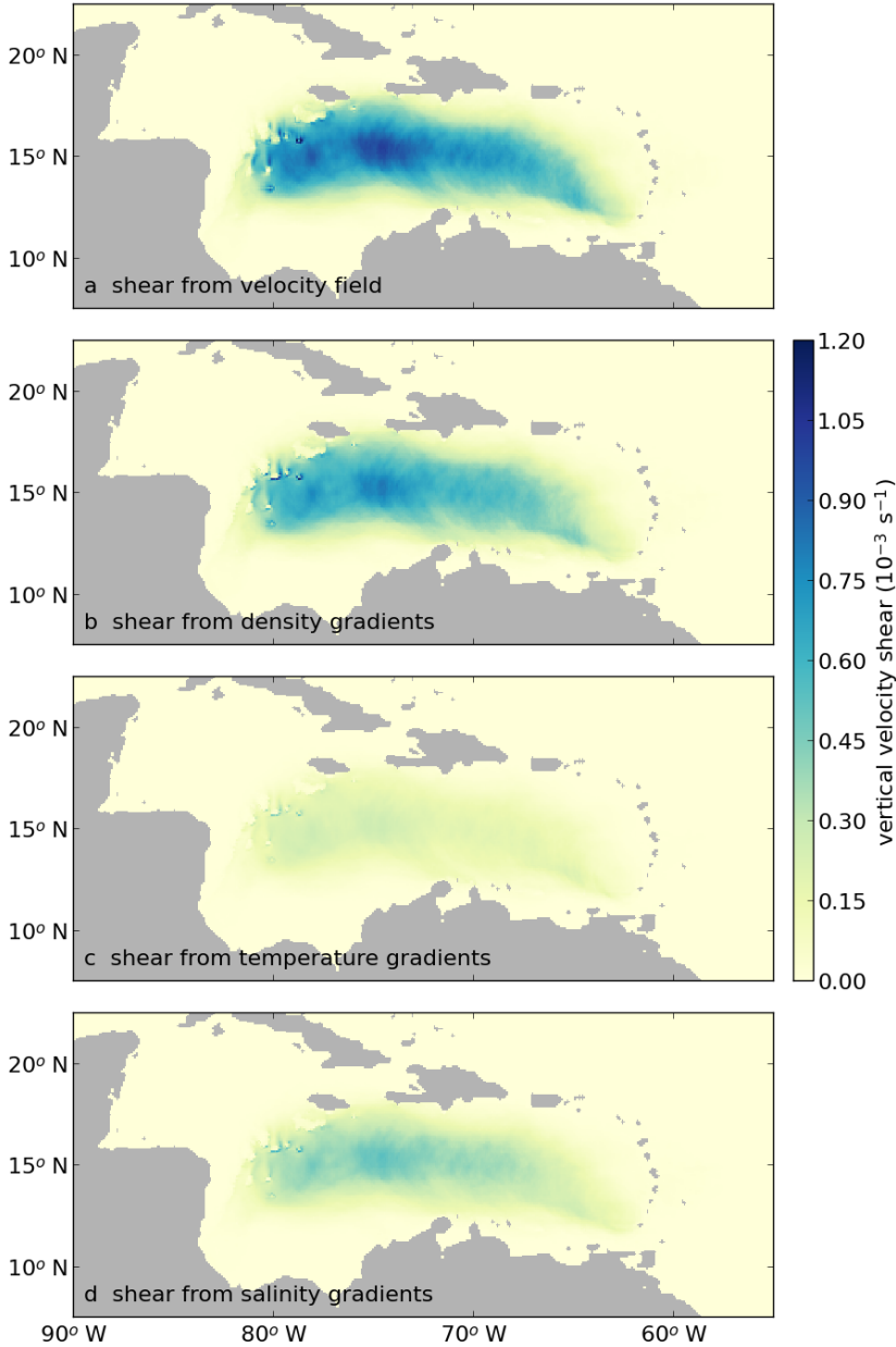
Figure 4.7: (a) Vertical shear of the anticyclones, averaged over the upper 50 m. (b) Horizontal density gradients of the anticyclones, scaled with g/(\rho_0 f) according to the thermal wind equation. Horizontal density gradients due to (c) temperature gradients and (d) salinity gradients of the anticyclones.
