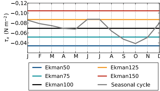
Figure 4.2: Average zonal wind stress in \text{N m}^{-2} in the southern Caribbean Sea ( 10.5^\circ\text{N} - 12.5^\circ\text{N} , 65^\circ\text{W} - 70^\circ\text{W} ) in the simulations. The seasonal variation of the zonal wind stress at this location, obtained from ERA-Interim (Dee et al., 2011), is shown for reference. Negative values correspond to easterly winds.
