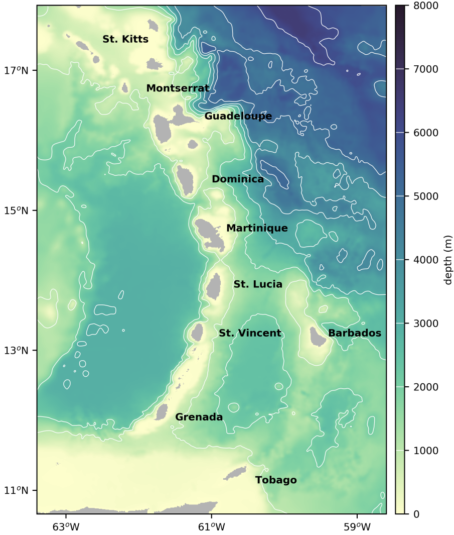
Figure 3.2: Bathymetry used in the nested grid of the Lesser Antilles ( LA-nest ). The white contour lines corresponds to the isobaths between 0 and 8000 meter at intervals of 1000 m.
