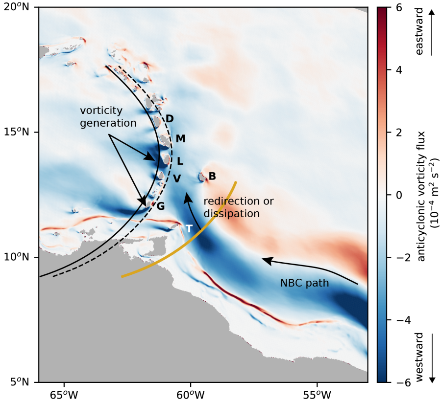
Figure 3.8: Zonal component of the anticyclonic vorticity flux integrated over the upper 300 m of the water column and averaged over 2 years model data from CS-nest . Negative values correspond to a flux in westward direction. Dashed and solid lines indicate the locations of the cross sections east and west of the Lesser Antilles, respectively. Letters are placed east of the islands to indicate their location: D = Dominica, M = Martinique, L = St. Lucia, V = St. Vincent, G = Grenada, T = Tobago, B = Barbados. The yellow curve indicates the location of the cross section along which the maximum sea-level anomaly is obtained that is used to gain insight into the passage of NBC rings in Section 3.5 (Fig. 3.10d).
