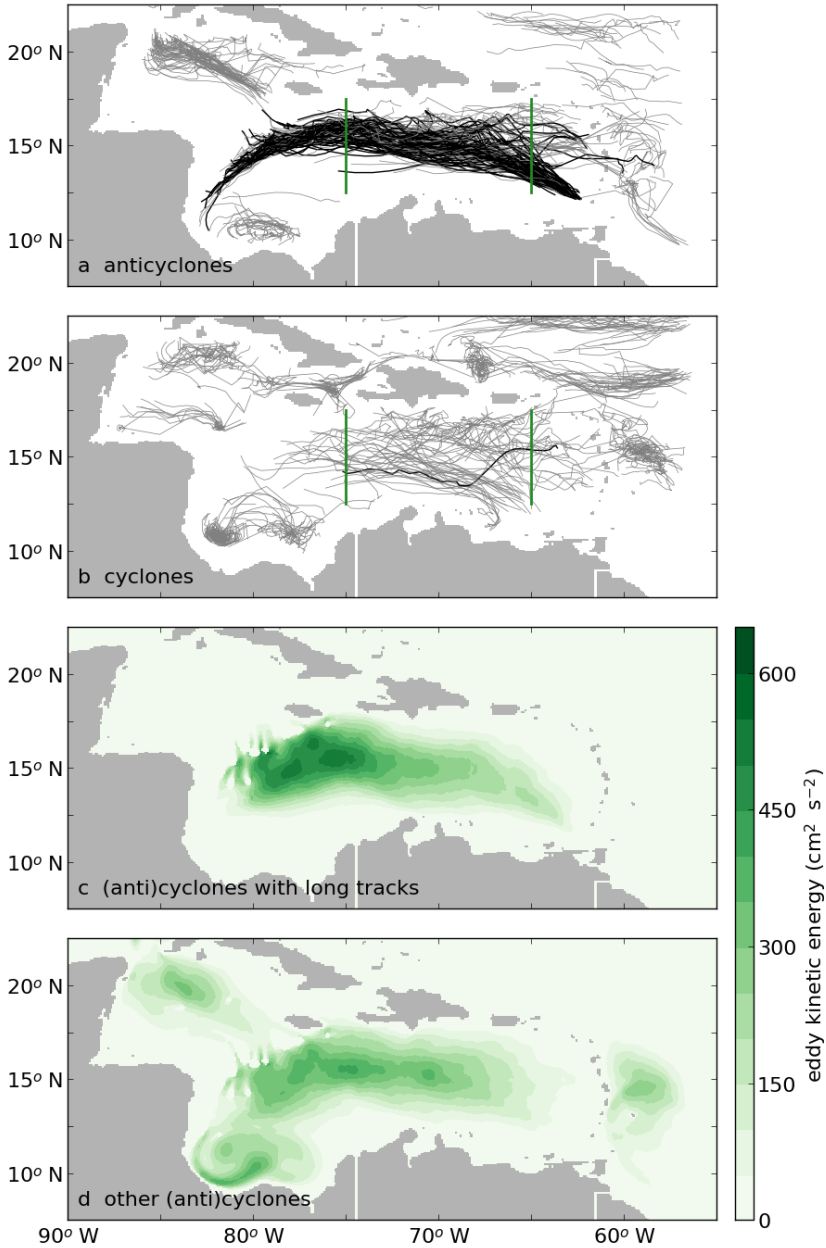
Figure 4.6: Paths of (a) anticyclones, and (b) cyclones that are identified by the py-eddy tracker (Mason et al., 2014) in Ekman100 during 20 years of model simulation. The black lines indicate tracks that pass both cross-sections at 65°W and 75°W (green lines). All other tracks are indicated in grey. (c) Estimate of EKE in \text{cm}^2 \text{s}^{-2} of the long tracks (black lines in panels a and b). (d) Estimate of EKE of all other tracks (grey lines in panels a and b).
