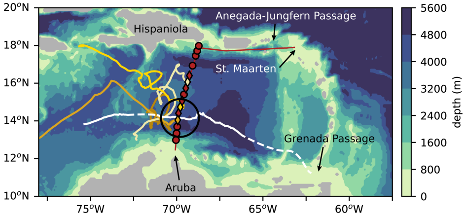
Figure 2.1: Bathymetry (m) of the eastern Caribbean Sea showing the cruise track (red line) and track of the center of the eddy (white line). The black circle indicates the location of the anticyclone, estimated from satellite altimetry, at the time of the survey. The track is obtained with the py-eddy tracker of Mason et al. (2014, white solid line) and extended with visual tracking of sea-level anomalies (white dashed line). Hydrographic stations along the cruise track that were sampled down to the bottom and down to 2000 m are shown with dots and diamonds, respectively. Red markers indicate a hydrographic stations, yellow markers indicate hydrographic stations where also Argo floats were deployed. The tracks of the Argo floats from February 2018 to September 2018 are shown with the yellow solid lines.
