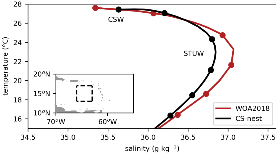
Figure 3.3: Temperature-Salinity diagram of the time-mean conservative temperature and absolute salinity in the eastern Caribbean Sea ( 63^{\circ}\text{W} - 66^{\circ}\text{W} , 13^{\circ}\text{N} - 17^{\circ}\text{N} , see dashed box in inlay) for the simulations with the CS-nest (black) and WOA2018 (red). Dots correspond to depth levels from 0 m to 250 m with intervals of 50 m. The approximate locations of Caribbean Surface Water (CSW) and Subtropical Underwater (STUW) are indicated.
