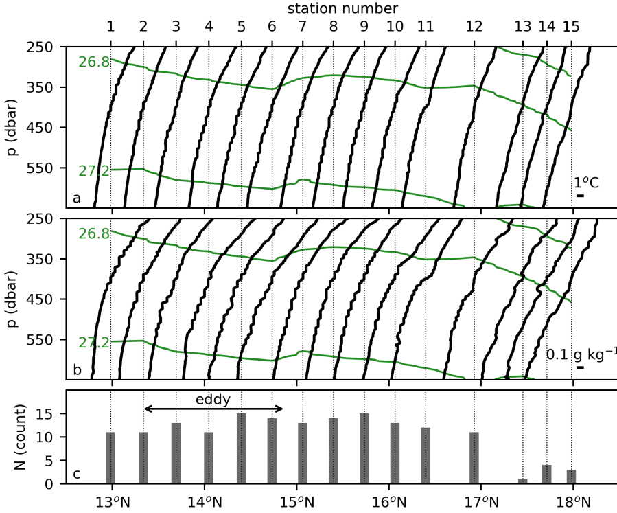
Figure 2.7: (a) Conservative temperature ( ^{\circ}\text{C} ) profiles and (b) absolute salinity ( \text{g kg}^{-1} ) profiles obtained with the CTD, between 250 and 650 dbar. \sigma -contours are indicated. Each profile is projected upon the latitude of the station, indicated with the dashed black lines. The green lines show the density contours along the track. (c) The number of staircases that were found in each profile.
