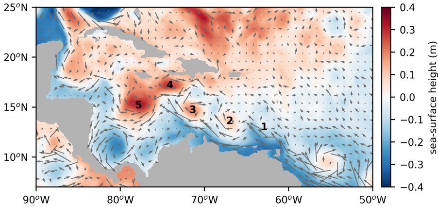
Figure 1.2: Sea-surface height with respect to the mean sea level in the Caribbean Sea ( 50^{\circ}\text{W} - 90^{\circ}\text{W} , 8^{\circ}\text{N} - 25^{\circ}\text{N} ) on 4 January 2018. Arrows indicate direction of the flow. Numbers 1-5 indicate anticyclonic eddies present at that time in this domain. Numbers increase along the direction of the mean flow. Data is taken from the GLORYS Ocean Re-analysis model, and downloaded from the Copernicus Marine Environment Monitoring Service ( http://marine.copernicus.eu ).
