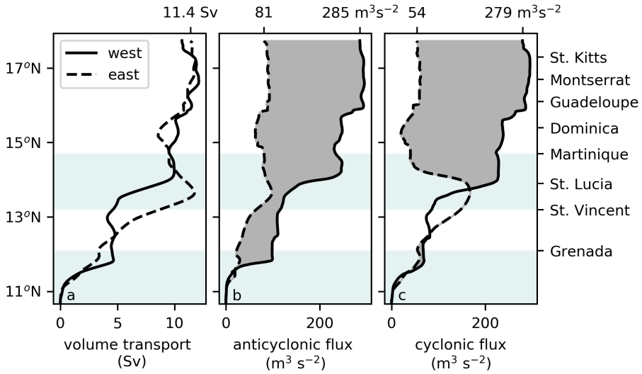
Figure 3.15: Same as Fig. 3.9, but then during the collision of an NBC ring with the Lesser Antilles (3 June to 28 June, as simulated by the LA-nest configuration).
