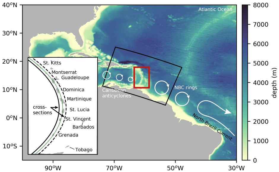
Figure 3.1: Map of the bathymetry of the Caribbean Sea, used in the numerical simulations. The black box indicates the domain of the first nested grid ( CS-nest ), the red box indicates the second nested grid ( LA-nest ). Typical locations and size of Caribbean anticyclones, North Brazil Current rings and the North Brazil Current are sketched in white. The inlay zooms in on the islands of the Lesser Antilles, and indicates the locations of the eastern (dashed line), middle (green line) and western (solid line) cross sections used in the analyses.
