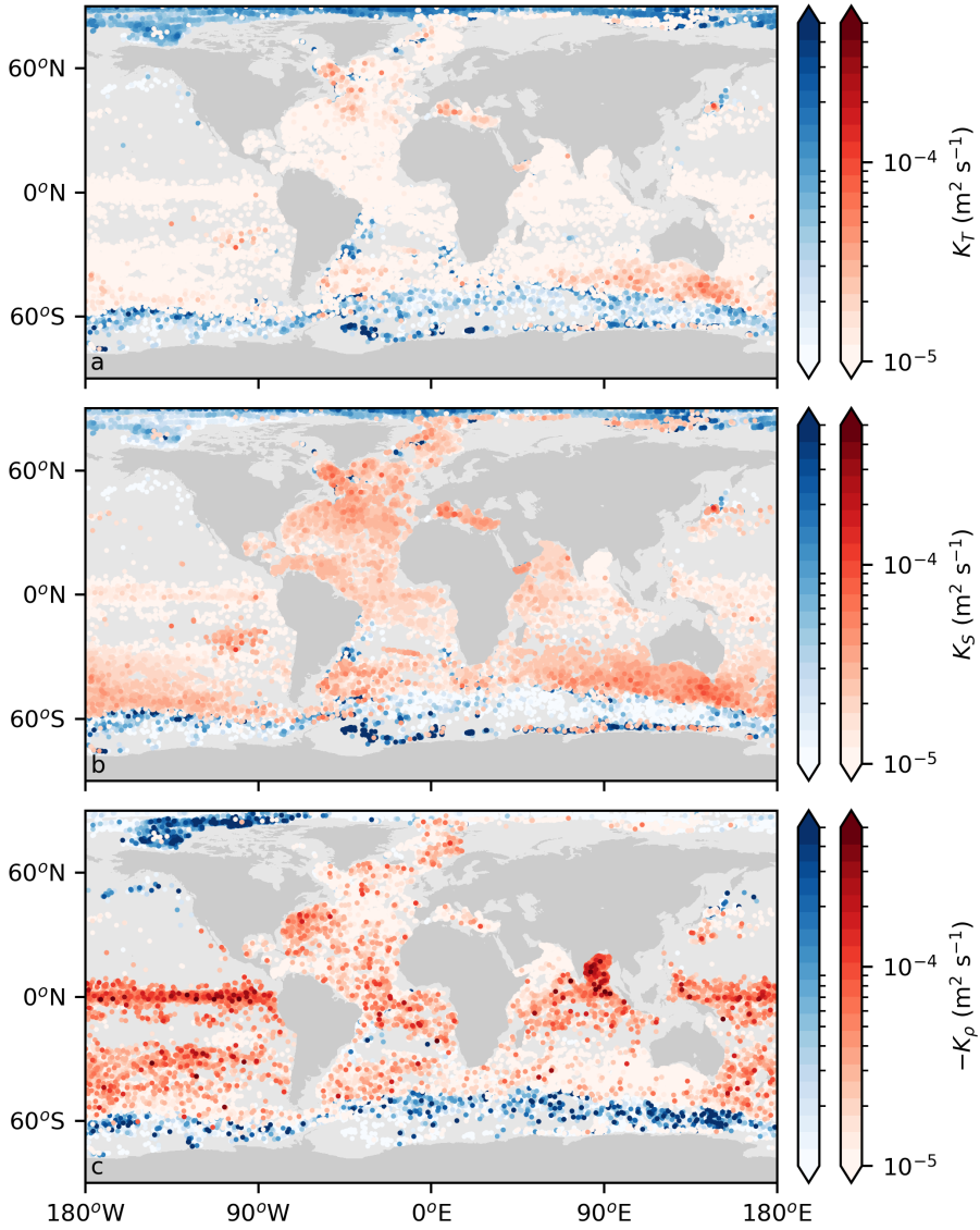
Figure 6.3: Effective diffusivities (per profile) computed in each profile with a thermohaline staircase. For each profile, the average diffusivities per staircase in the salt-finger regime (red dots) and diffusive-convective regime (blue dots) are plotted. Panels show the average effective diffusivity of (a) heat ( K_T ) and (b) salt ( K_S ) and (c) buoyancy ( K_\rho ) per profile.
