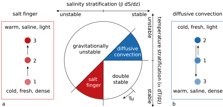
Figure 1.7: Schematic of double-diffusive convection in the (a) salt-finger regime and (b) diffusive-convective regime. The shading of the water parcels indicates the density. The middle panel is modified from Ruddick (1983), and indicates the types of stratification that result in double-diffusive mixing as a function of the Turner angle ( T_u , Ruddick, 1983).
