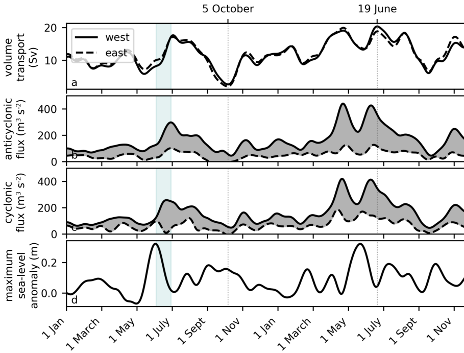
Figure 3.10: Total (a) transport (b) anticyclonic vorticity flux and (c) cyclonic vorticity flux at the Lesser Antilles integrated along the eastern (dashed lines) and western (black solid line) cross section (Fig. 3.1) and over the upper 300 m of the water column. (d) Maximum sea-level anomaly between Barbados and Tobago along the yellow line in Fig. 3.8. Red lines indicate the percentage of generated vorticity compared to total vorticity flux into the Caribbean computed at the western cross section. The grey shaded area corresponds to the vorticity flux that is generated between the cross sections. The light blue shading indicates the collision studied in Figures 3.12-3.15. The data is from CS-nest and smoothed with a Hanning window of 30 days.
