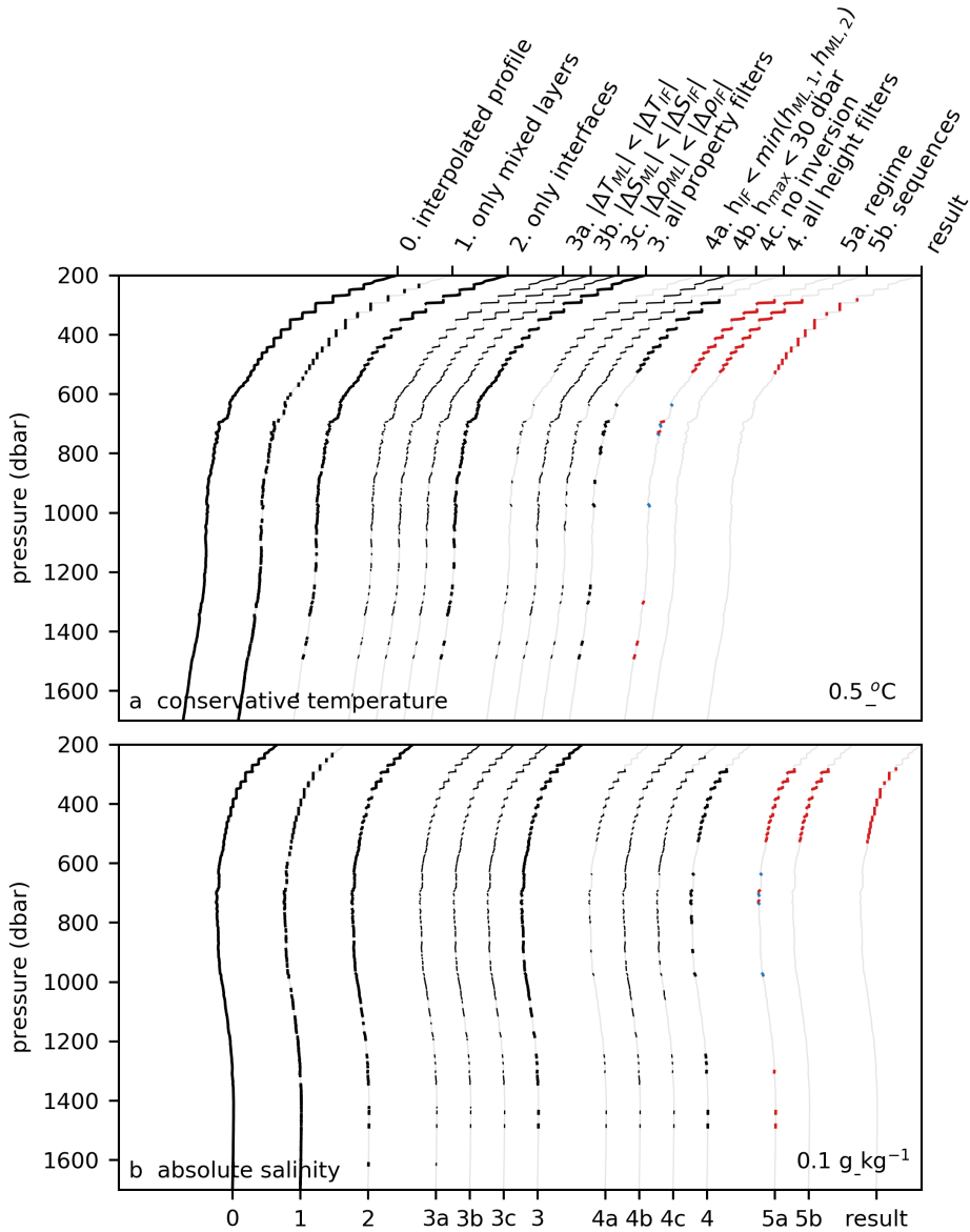
Supplementary Figure 5.11: as Supplementary Figure 5.9, but for a profile in the western tropical North Atlantic. Original profile is taken from Argo float 4901478 at 53.3°W and 11.6°N on 9 August 2014.
