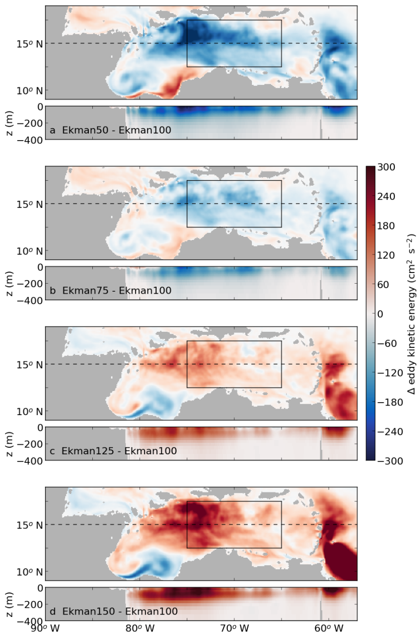
Figure 4.11: EKE anomaly compared to Ekman100 (Fig. 4.4) at the near-surface and at a cross-section at 15°N in (a) Ekman50, (b) Ekman75, (c) Ekman125 and (d) Ekman150. Positive values correspond to enhanced EKE compared to Ekman100. The black box indicates the interior of the Caribbean Sea (12.5°N-17.5°N, 65°W-75°W). The dashed line shows the location of the cross-sections in the lower panels.
