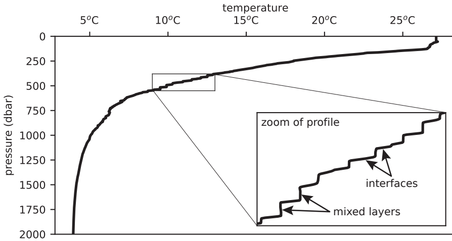
Figure 1.6: Temperature profile as observed during a hydrographic survey on 6 February 2018 at 14.7°N, 69.8°W (see Chapter 2 of this thesis). The inlay shows a zoom of the thermohaline staircase.
