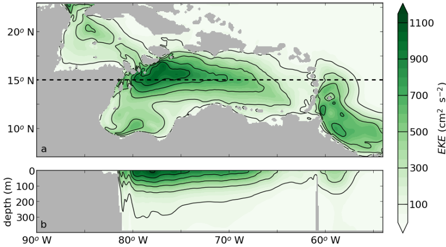
Figure 4.4: Eddy kinetic energy (EKE) in \text{cm}^2 \text{s}^{-2} of Ekman100 obtained from 5-day averaged velocity fields that are high-passed filtered with a 125-day mean. (a) 20-year average of the EKE in the upper 50 m of the water column and (b) cross section of EKE at 15°N over the upper 400 m.
