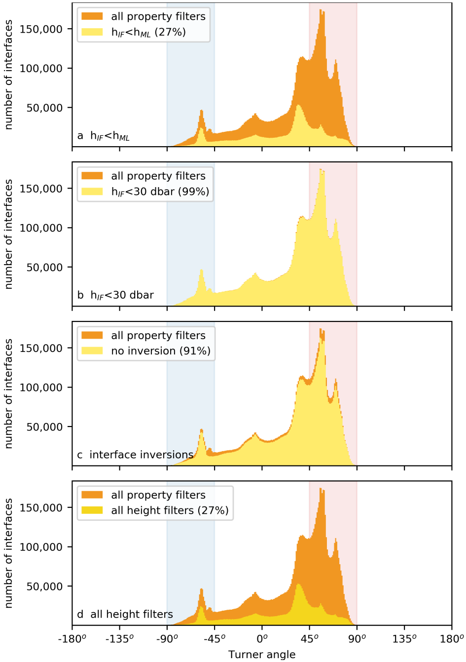
Figure 5.5: Histogram of the number of detected interfaces as a function of the Turner angle ( Tu ) by applying a criterion for (a) height, (b) maximum height, (c) inversions and (d) all three height limitations (yellow shading). Each panel shows the data remaining compared to the interfaces detected based on the conservative temperature and absolute salinity requirements shown in Fig. 5.4d (orange shading). Vertical shaded bands correspond to Turner angles in the diffusive-convective (blue) and salt-finger (red) regime.
