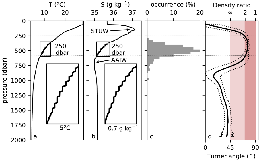
Figure 7.2: (a) Temperature and (b) salinity profile of Caribbean staircase obtained with Argo float 4901720 at 75.5°W and 13.9°N on 9 November 2018. (c) Depth of detected mixed layers of all thermohaline staircases in the Caribbean Sea (62°W-82°W and 10°N-18°N, dashed box in Fig. 7.1) obtained from the global dataset of thermohaline staircases (Chapter 5 of this thesis). (d) Average Turner angle (Ruddick, 1983) computed from 1565 Argo float profiles in the Caribbean Sea. The dashed lines correspond to one standard deviation from the mean Turner angle. The (dark) red shading corresponds to Turner angles that are susceptible to (strong) salt fingering. The upper and lower bound of the Turner angles with strong salt-fingering are indicated by the horizontal lines in all panels. The density ratios that correspond to these Turner angles are indicated on the upper axis. The inlays show a zoom over 250 dbar and 5°C and 0.7 g kg -1 of the thermohaline staircase. The approximate locations of Antarctic Intermediate Water (AAIW) and Subtropical Underwater (STUW) are indicated in panel (b).
