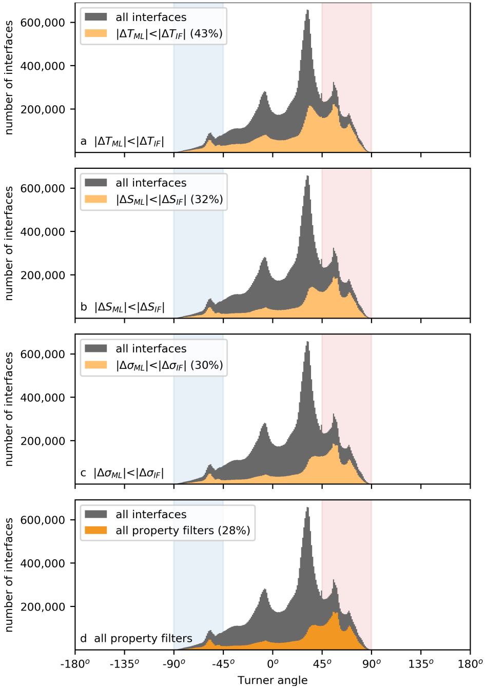
Figure 5.4: Histogram of the number of detected interfaces as a function of the Turner angle ( Tu ) by applying a criterion for (a) conservative temperature, (b) absolute salinity, (c) potential density and (d) all three properties given in equation 6.7 (orange shading). Each panel shows the data remaining compared to the raw interface data (grey). Vertical shaded bands correspond to Turner angles in the diffusive-convective (blue) and salt-finger (red) regime.
