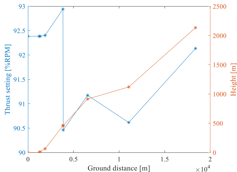
Figure 3.17. Take-off profiles 4690501
