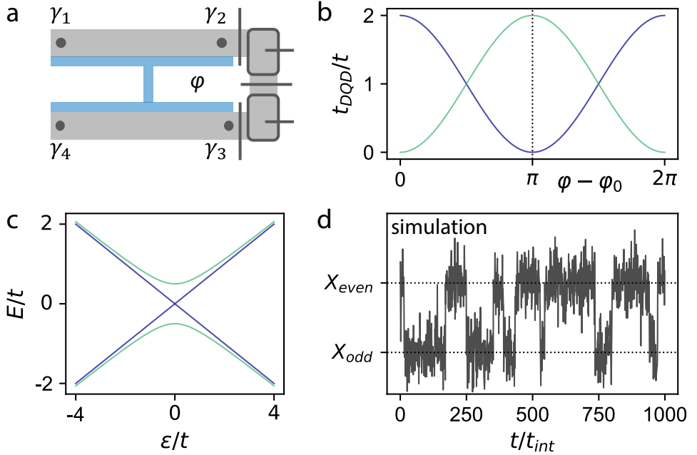
Figure 9.3 – Majorana parity readout in a Majorana box qubit. a Minimal setup to do a Majorana parity measurement using a Majorana box qubit. Because of the loop, this device is sometimes referred to as the loop qubit. b Tunnel coupling between the dots as a function of flux through the loop for different parity states (with even/odd in blue/green). When \phi - \phi_0 = n\pi with integer n , the contrast between the parity states is maximal. c Energy spectrum of the double dot at the point of maximal contrast. d Time trace of the reflected signal X showing parity fluctuations. For this simulation, we used an exponential distribution for the parity switches with \tau_{even} = 100 t_{int} and \tau_{odd} = 50 t_{int} , and a signal-to-noise ratio of 2.
