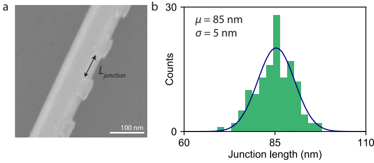
Figure 3.6 – Calibration of the transene D etch. a Scanning electron micrograph of a test sample used to calibrate the etching recipe. The remaining aluminium patches are visible on the top-right facet of the wire. b Histogram of the junction length obtained by analyzing 134 junctions made using the optimized recipe. The histogram shows that we can reliably make 85 nm long junctions.
