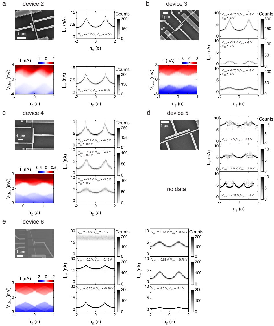
Figure 4.S1 – Scanning electron micrographs, Coulomb diamonds, and gate dependence of the 2e -periodic signal for device 2-6 (a – e). The E_C^0 and \Delta extracted from Coulomb blockade are summarized in Table 4.S1. Apart from device 5 which shows an even-odd pattern in the switching current modulation, all devices show a 2e modulation, illustrating that the 2e signal does not correspond to a fine-tuned gate setting. The gate settings corresponding to the measurements are specified in each subfigure. The gates are labeled using the same convention as in the main text. For device 2, 5, and 6 the backgate is fixed at V_{BG2} = -10 V, V_{BG5} = -8.5 V, and V_{BG6} = 0 , respectively.
