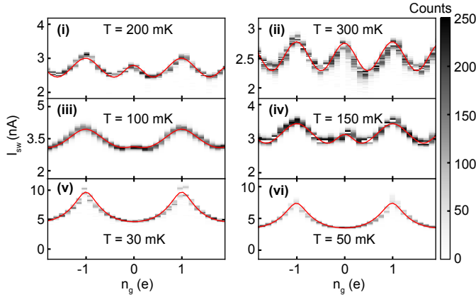
Figure 4.S4 – Switching current modulation as a function of temperature for device 2 at R_N = 10.5 k \Omega . The experimental histograms shown in grayscale are overlaid by the theoretical fit to the average switching current ( I_{\text{sw}} ) (red curves). Individual fits are for different values of \Delta , E_J , and E_C . The averaged values for these parameters are \Delta \approx 245 \mu\text{eV} , E_C \approx 192 \mu\text{eV} , and E_J \approx 111 \mu\text{eV} .
