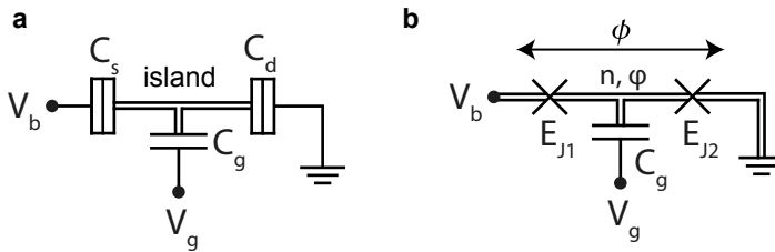
Figure 2.5 – Circuit diagram for a superconducting island (a) and a single-Cooper-pair transistor (b). The double lines indicate the superconducting sections of the device. In b , \phi is the superconducting phase across the island and \phi is the phase of the superconductor on the island. \phi and n are conjugate variables and cannot be determined simultaneously.
