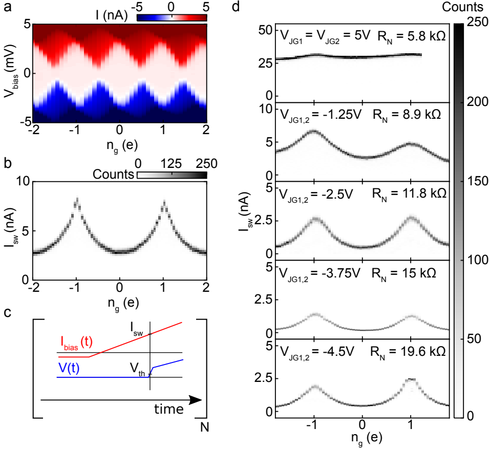
Figure 4.2 – Gate dependence of the 2e -periodic switching current modulation. a Coulomb diamonds measured in the strongly Coulomb-blockaded regime with \Delta = 180\text{ }\mu\text{eV} and E_C^0 = 1.5\text{ meV} . b Histogram of the 2e -periodic switching current I_{\text{sw}} in the weakly Coulomb-blockaded regime, indicating that \Delta > \delta E_{\text{eq}} . At this gate setting, V_{\text{JG1}} = -4.1\text{ V} and V_{\text{JG2}} = -5.7\text{ V} , R_N = 14.8\text{ k}\Omega . c Schematic representation of the current ramp (in red) used to obtain the I_{\text{sw}} histograms and the resulting voltage across the SCPT (in blue). The switching current I_{\text{sw}} is recorded when the voltage drop on the SCPT reaches a threshold value V_{\text{th}} . d Switching current histograms for varying normal state resistance. The normal state resistance is calculated as the average over the n_g range at high bias. Note the change of vertical scale for the two topmost panels. The peak height asymmetry seen for R_N = 8.9\text{ k}\Omega and R_N = 19.6\text{ k}\Omega is due to cross coupling between the junctions and V_{\text{PG}} .
