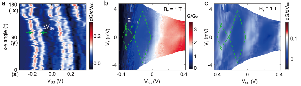
Figure 7.S5 – g -factors in B_y (in-plane but perpendicular to current flow) for the etch-defined QPC in the main text. Figure 7.5 in the main text shows the bias spectroscopy of the QPC transconductance in B_x and B_z , from which anisotropic g -factors are extracted. As shown in Fig. 7.4d in the main text, the roughly constant width of the 0.5 plateau when the magnetic field is rotated in the z - y plane implies an isotropic in-plane g -factor. This figure shows a the numerical transconductance of Fig. 7.4d in the main text, b bias spectroscopy with B_y = 1 T and c its numerical transconductance. The high dG/dV_{SG} in a (red color) represents transitions between conductance plateaus and the green arrow illustrates the width of the 0.5 plateau \Delta V_{SG} , which is roughly constant. The energy separation E_{1\downarrow-1\uparrow} \approx 1.6 meV is small (indicated by the green dashed and solid lines in b ) as it is limited by the low maximal field for the y component of the vector magnet. This leads to a relatively large uncertainty. Still, from E_{1\downarrow-1\uparrow} = |g_{1,y}|\mu_B B , we find |g_{1,y}| \approx 28 , close to |g_{1,x}| \approx 26 as shown in the main text.
