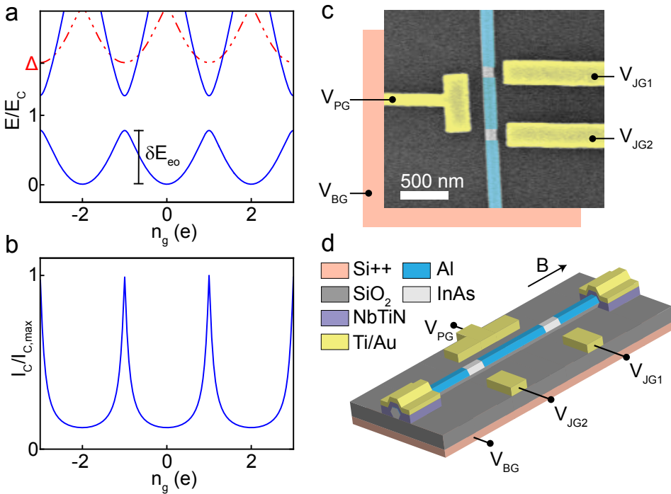
Figure 4.1 – Theoretical background and device layout. a The band structure of a SCPT as a function of gate-charge n_g for \phi = 0 , \Delta/E_C = 1.5 , and E_I/E_C = 0.25 . The charge dispersion of the odd parity branch (in red) is displaced from the even parity branch (in blue) by the superconducting gap \Delta and \delta n_g = 1 . The amplitude of the ground state charge dispersion is denoted by \delta E_{eo} . b The corresponding critical current modulation as a function of n_g . c A false-coloured scanning electron micrograph of a nanowire SCPT. The etched regions in the Al shell define the junctions and the island. By applying voltages to the electrostatic gates, we can tune the chemical potential (with V_{BG} ), the junction transparency (with V_{JG1,2} ) and the charge occupation of the island (with V_{PG} ). d 3-dimensional device schematic. The nanowire is deterministically placed on top of a \text{SiO}_2/\text{Si}^{++} substrate. It is then contacted by a stack of NbTiN and Ti/Au 1\mu\text{m} away from the etched regions. Finally, the local gates are deposited. The arrow indicates the direction of the magnetic field for the data presented in Fig. 4.4.
