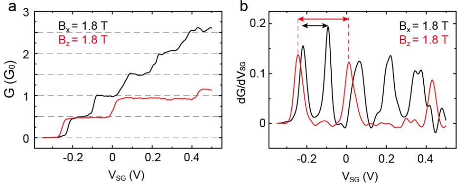
Figure 7.S4 – Linecuts taken from Fig. 7.4c in the main text. a Two line cuts at x - z angle = 0 (along current flow, B_x = 1.8 T, black) and 90 degrees ( B_z = 1.8 T, red). For the whole 2D color plot of Fig. 7.4c a series resistance of 6.5 k \Omega from the adjacent InSb 2DEG is subtracted to match the quantized conductance at B_x = 1.8 T (black). However, when the B_z component increases, the magnetoresistance of the adjacent 2DEG rises and therefore the calculated conductance of the QPC drops below the actual value. As shown by the red line, the conductance at the quantized plateaus is lower than the expected value. Nevertheless, the width of the 0.5 plateau at B_z = 1.8 T is wider than that at B_x = 1.8 T, indicating a g -factor anisotropy. The exact width can be obtained from the numerically calculated transconductance dG/dV_{SG} as shown by the red and black arrows in b , \Delta V_{SG} = 0.256 V and 0.126 V respectively. Therefore, an out-of-plane and in-plane g -factor anisotropy of about two is inferred.
