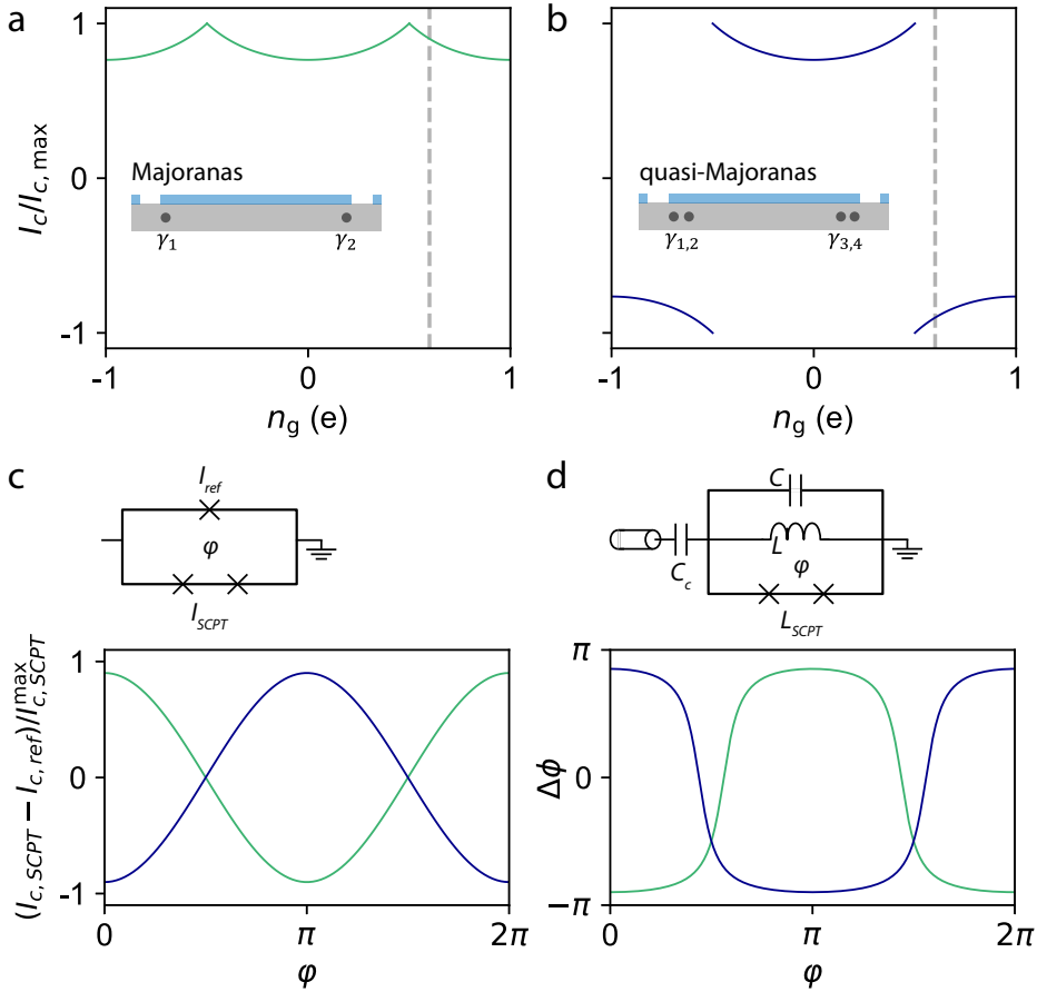
Figure 9.1 – Current-phase relation of a (quasi-)Majorana single-Cooper-pair transistor. a
