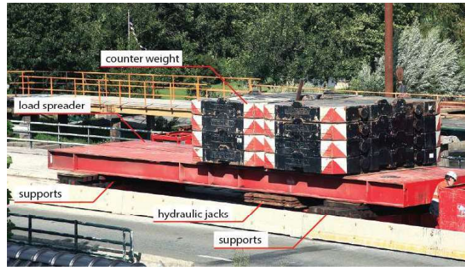
Fig. 3. Photograph of proof loading configuration as used by DUT
