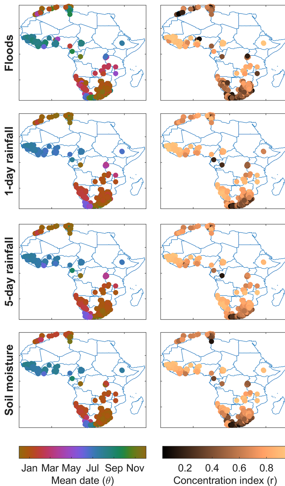
Figure 4. Mean dates of occurrence of annual maximum flood (top row), 1-day (second row) and 5-day (third row) annual maximum precipitation (based on CHIRPS), and annual maximum soil moisture (based on ERA5-land's second soil layer) (bottom row). The concentration around these dates is shown in terms of the concentration index ( r ) in the right column.
