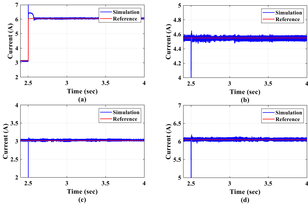
Fig. 13. PV string current, Case II → Case III: PV (a) string #1, (b) string #2, (c) string #3, and (d) string #4.
