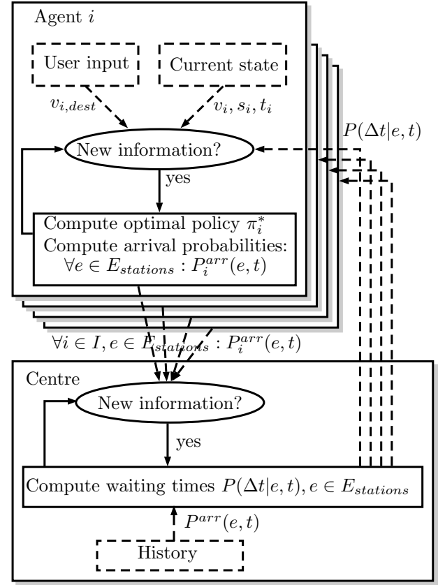
Fig. 2. Intention-Aware Routing System Architecture
