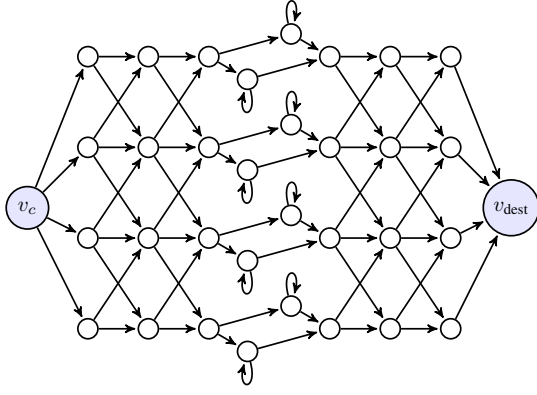
Fig. 1. Example road network from the perspective of a single EV with current position v_c and destination v_{dest} . Vertices indicate decision points, and edges are either roads or charging stations. Charging stations are indicated by self loops.
