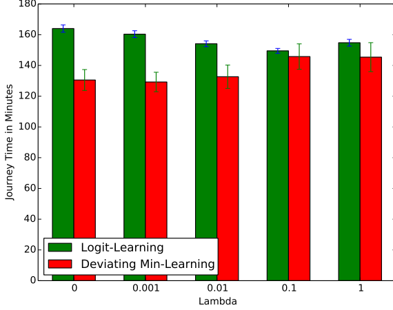
Fig. 6. All (except for one) agents use LOGIT( \lambda ) in a scenario with station capacity of two.
