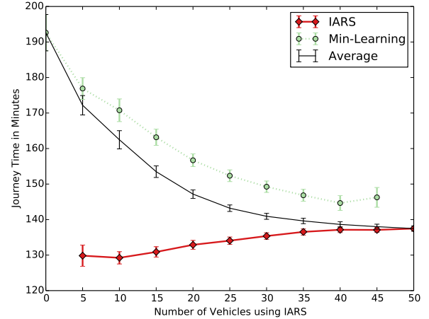
Fig. 10. In a scenario with station capacity of two, the more agents use IARS, the lower the average journey time (if other agents use MIN).
