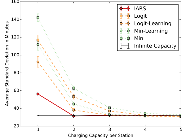
Fig. 9. The standard deviation is significantly lower for IARS than for any of the other approaches.
