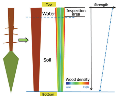
Fig. 2. Sketch of a sound tree stem as foundation pile upside down; possible density development along the length of the pile (colored picture); possible strength development along the length; accessible inspection zone at the top of the piles.
