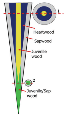
Fig. 3. Sketch of 2 cross sections (circular areas 1 and 2) of the pile at different heights of the pile.
