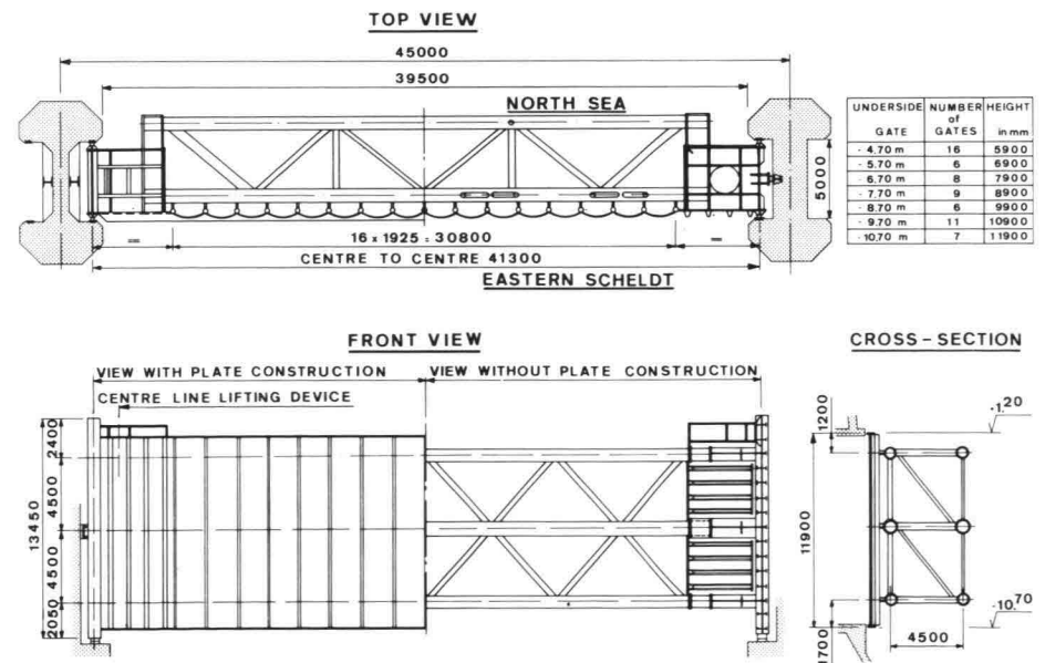
7 Construction of gates
