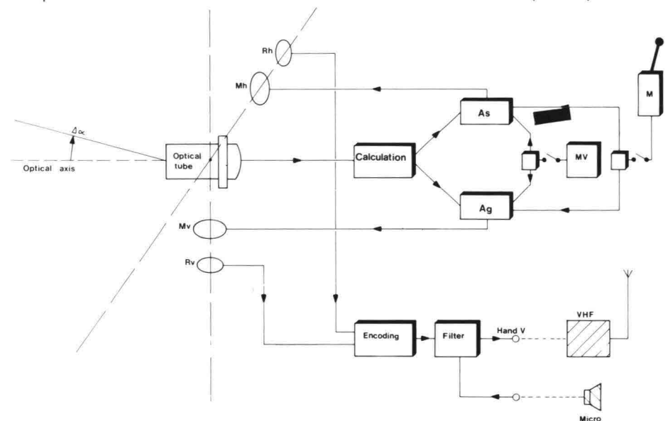
2 Schematic operation (Minilir)
