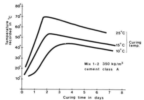
1 Typical curves for the average temperature in 1 m cubes (with 350 kg cement per m 3 concrete) under almost adiabatic conditions
