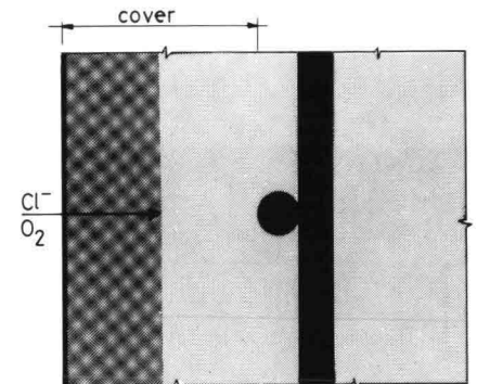
PHASE 1 \text{Cl}^- penetration
