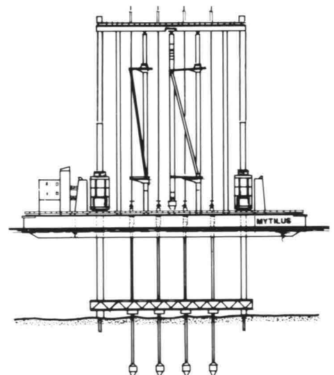
13 Compacting barge
