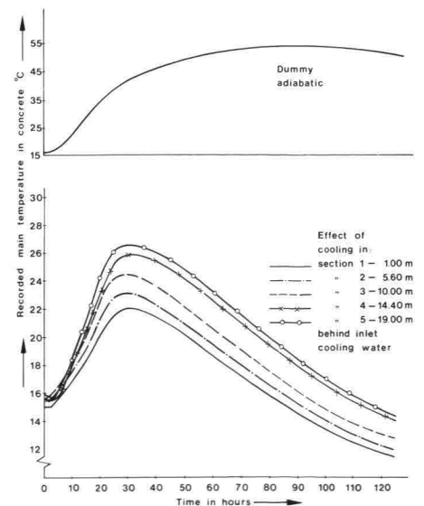
9 Effect of cooling in a concrete cross-section of 650 x 650 mm with 1" pipe in the centre, water flow 0,48 m 3 /hour of 5°C
