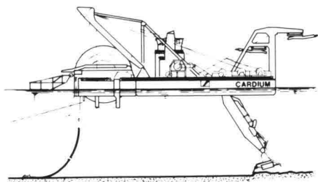
14 Mattress-laying vessel
