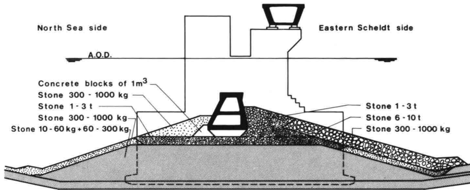
7 Sill construction
