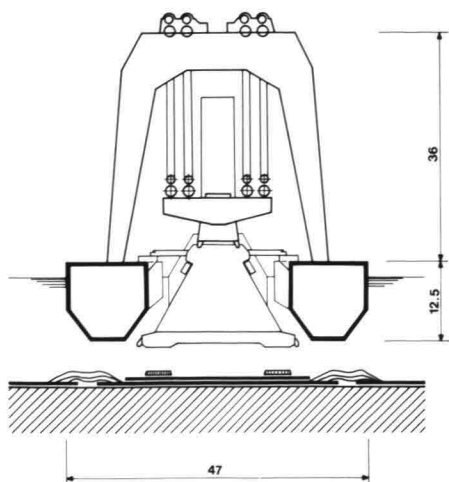
5 Lifting vessel Ostrea
