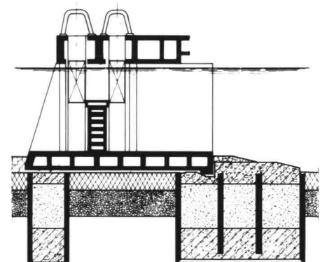
6 Gated caissons on a pile foundation
