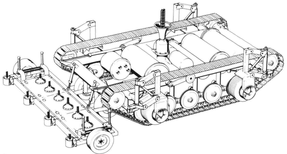
3 Seabed crawler 'Portunus'
