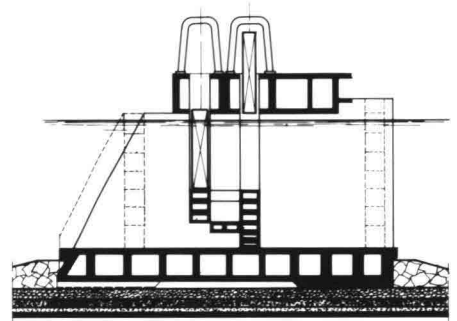
5 Gated caisson on a rubble base
