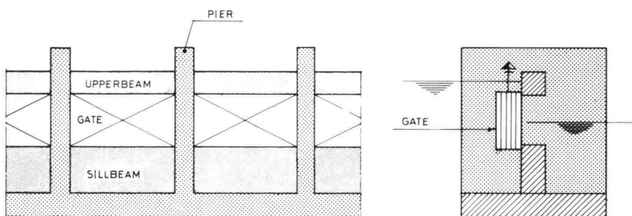
1 Schematization of the barrier
