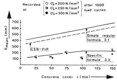
11c Mean crack spacing S_{mean}
