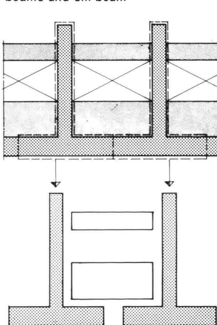
2b Method 2: joint between piers upper beams and sill beam
