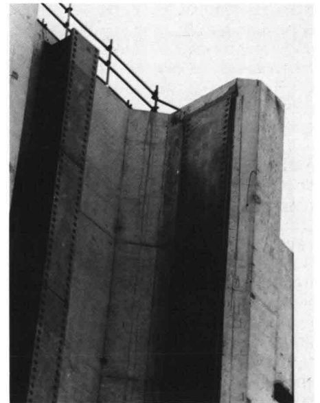
12 Alu-bronze rubbing faces mounted on the pier
