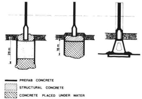
9 Evolution of the design of the foundation
