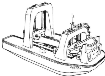
15 Pier-lifting vessel
