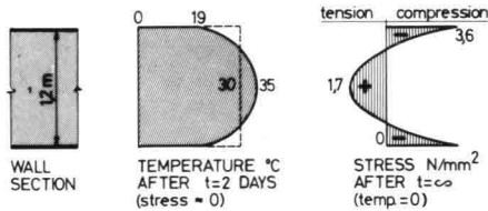
8 Temperature gradient and stresses in uncooled wall section
