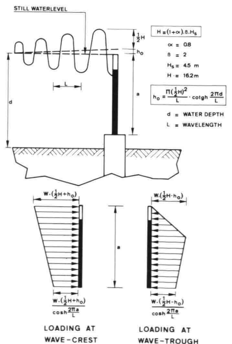
3 Wave loading of the gate
