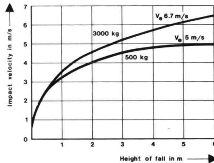
8 Underwater movement of the stones
