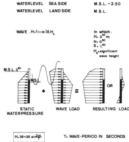
4 Loading of the gate at moment of closing
