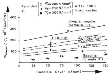
11b Mean crack width W_{mean}
