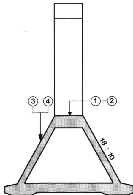
9 Impact areas on the pier
