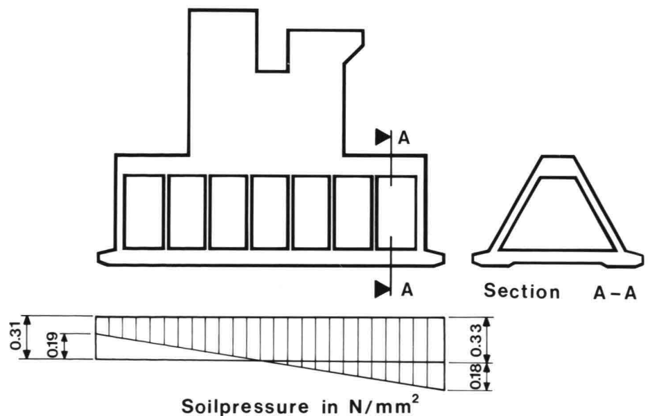
6 The cross-section subjected to probabilistic calculations
