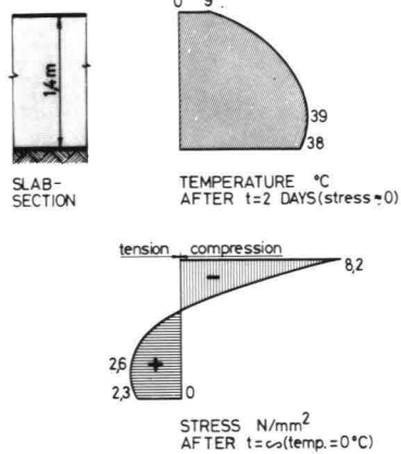
10 Development of temperature and stress in bottom slab (non-insulated)
