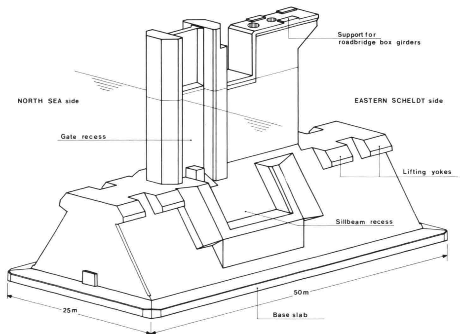
2 Concrete pier
