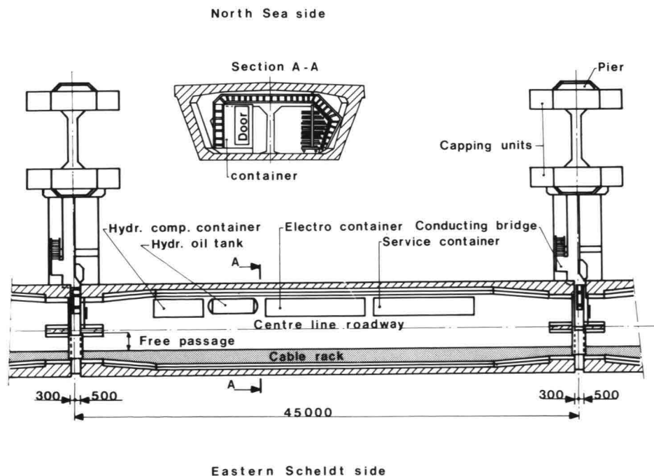
6 Components in box girders
