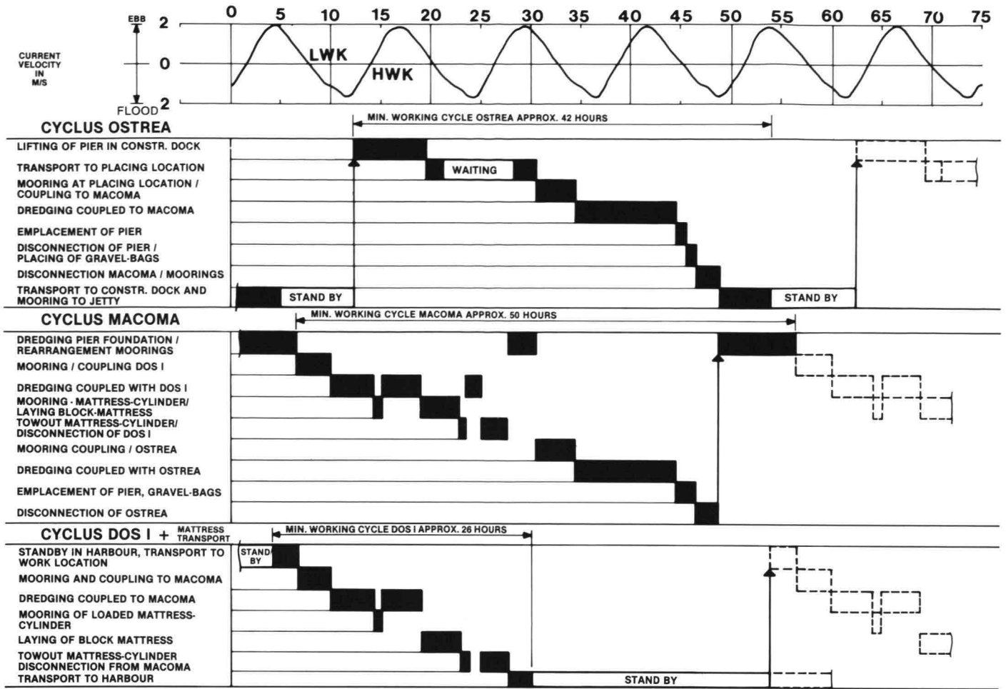
14 Working cycle of Ostrea, Macoma and Dos I
