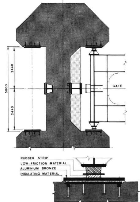
9 Rubbing faces in the piers
