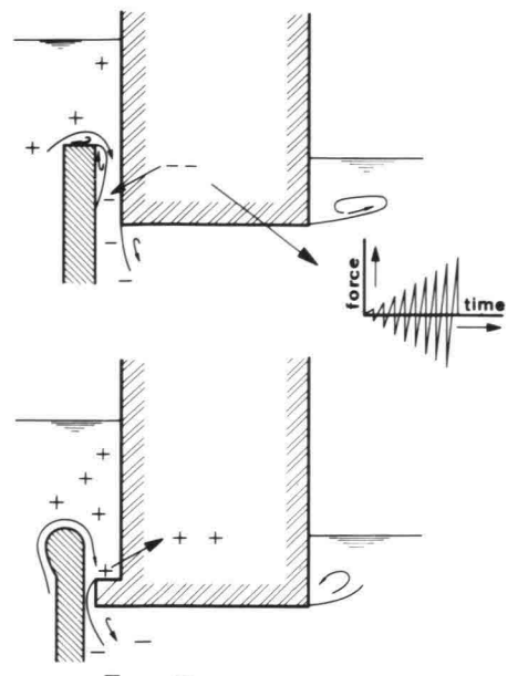
18 Nose construction upper beam for suppressing vibrations
