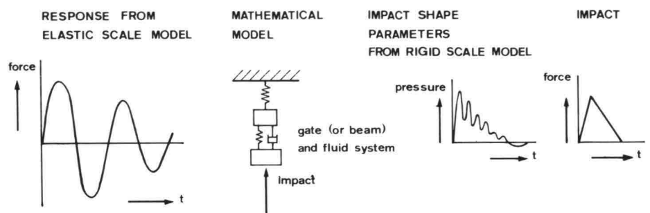
19 Calculation of wave impact
