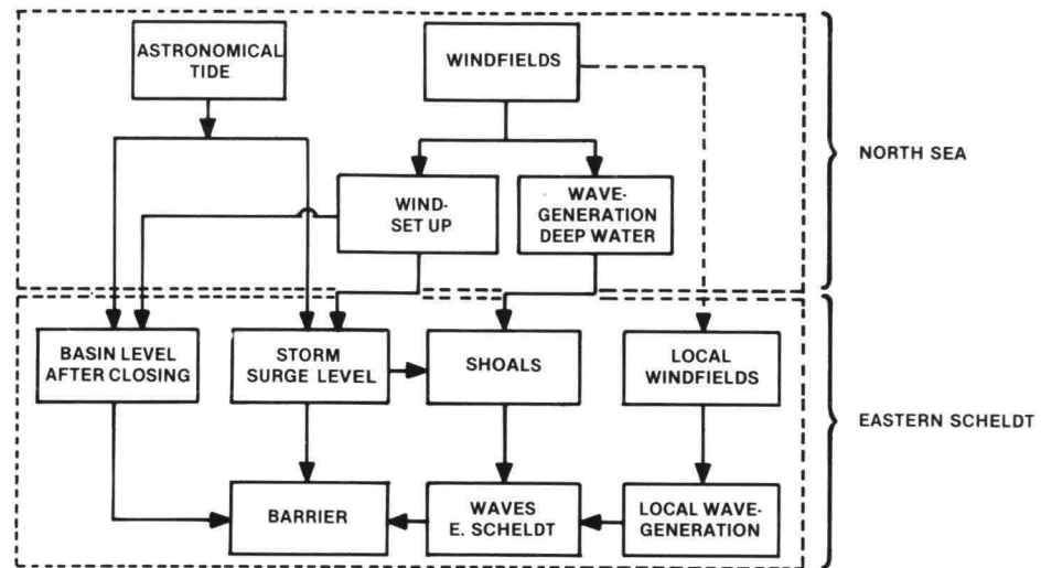
1 A schematic diagram of the physical relations used for the derivation of the three dimensional probability function of the storm surge level, wave energy and basin level
