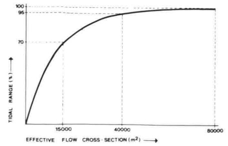
4 Relationship between tidal range and flow cross section
