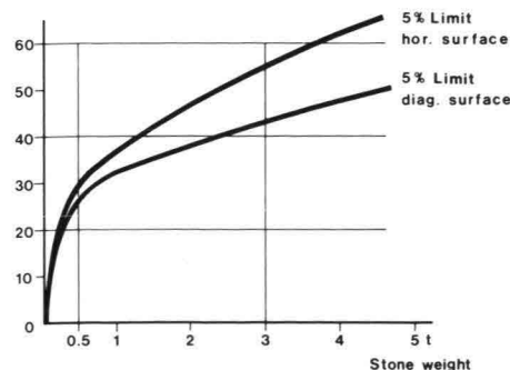
13 5% limit of damage depth on concrete
