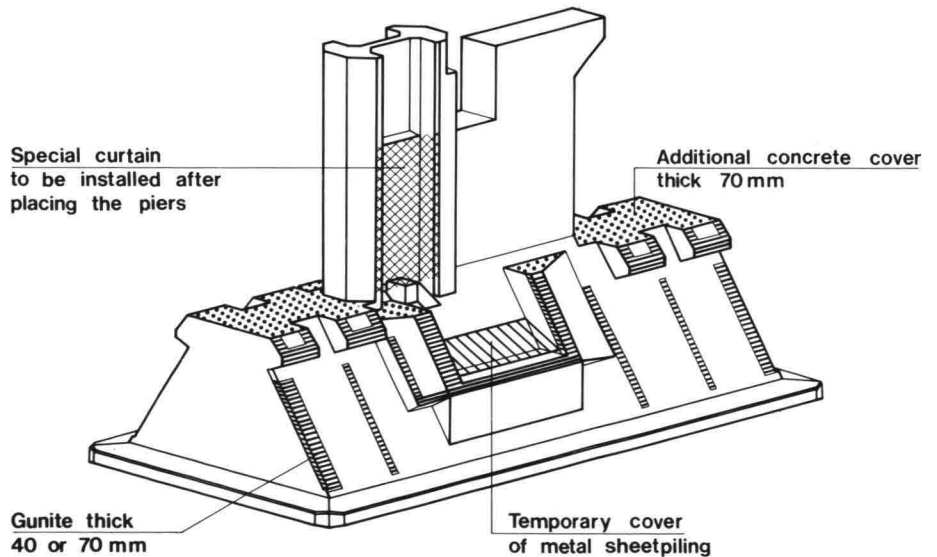
14 Protection against falling stones
