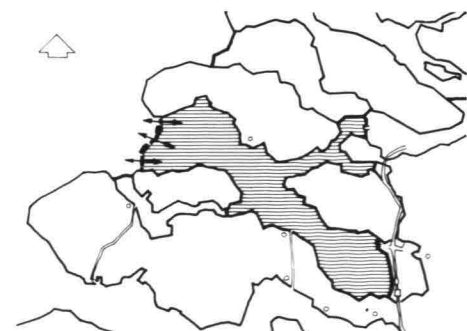
3 Modified Delta project
