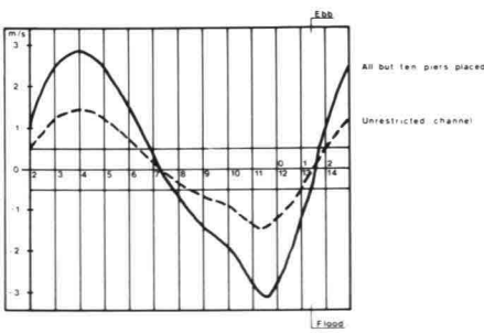
4 Velocity of tidal current in Roompot
