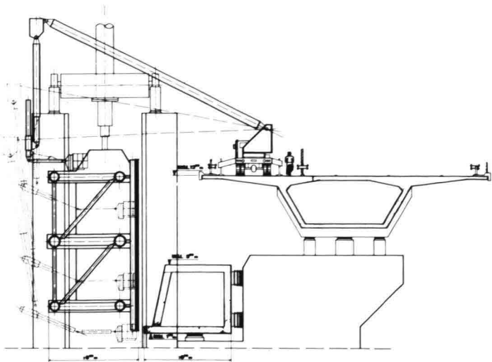
22 Inspection car
