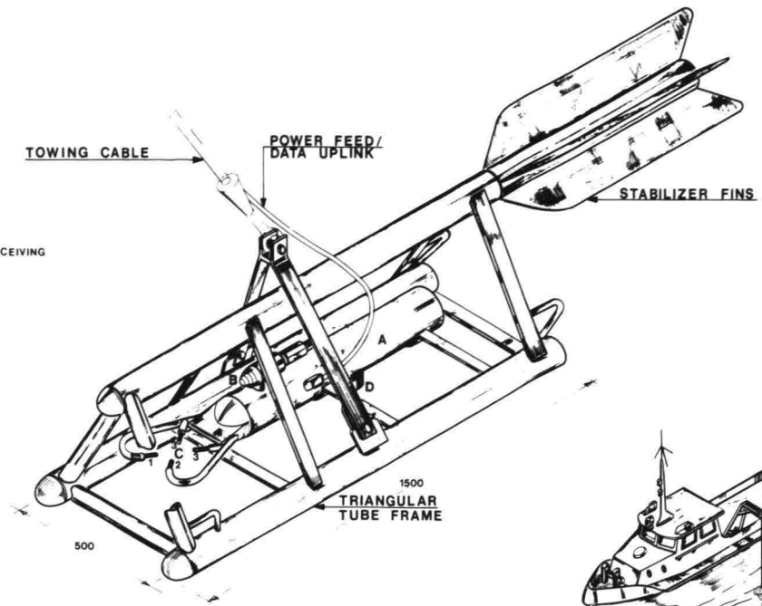
ACCOUSTIC DOPPLER SAMPLER WITH COMBINED ABSORPTION AND TRANSMISSION
