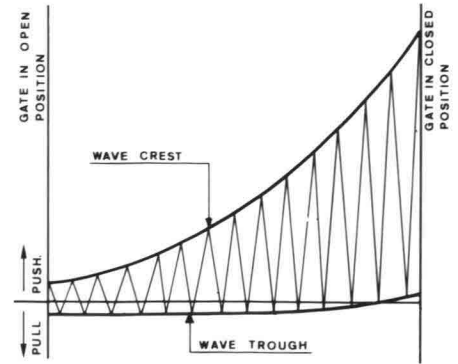
5 Forces required for closing the gate
