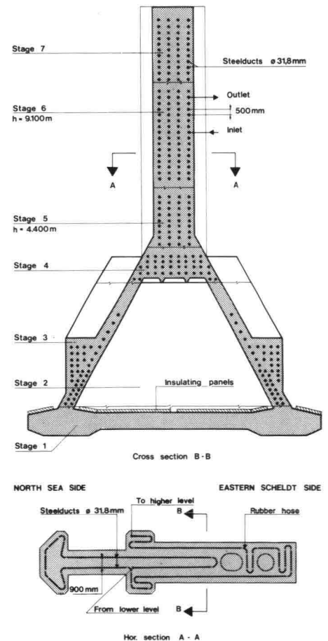
10 Cooling of concrete during curing
