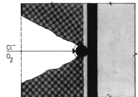
PHASE 3 loss of cover (free corrosion)
