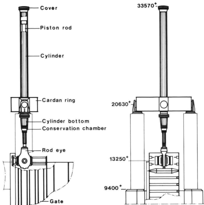
4 Operation machinery for gate h = 11,900 \text{ mm}
