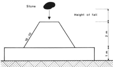
10 Testing arrangement
