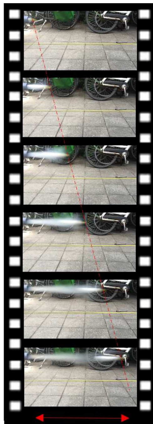
Figure 7 – Example of high-speed frame shots, used to verify the exit velocity (here with horizontal setup).
