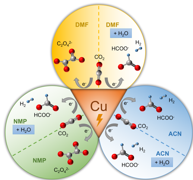
Figure 8. Schematic summarizing the major products produced on a copper electrode during electrochemical \text{CO}_2 reduction with DMF, NMP, and ACN electrolytes with and without the addition of water.
