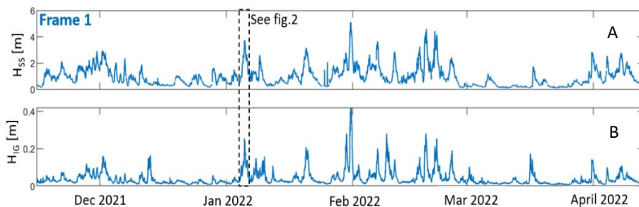
Fig. 1: Sea-swell (SS, f > 0.05 Hz) and infragravity (IG, 0.005 < f < 0.05 Hz) significant wave heights at the most offshore frame ( \bar{d} = 14.5 m) during the 5-month campaign.
