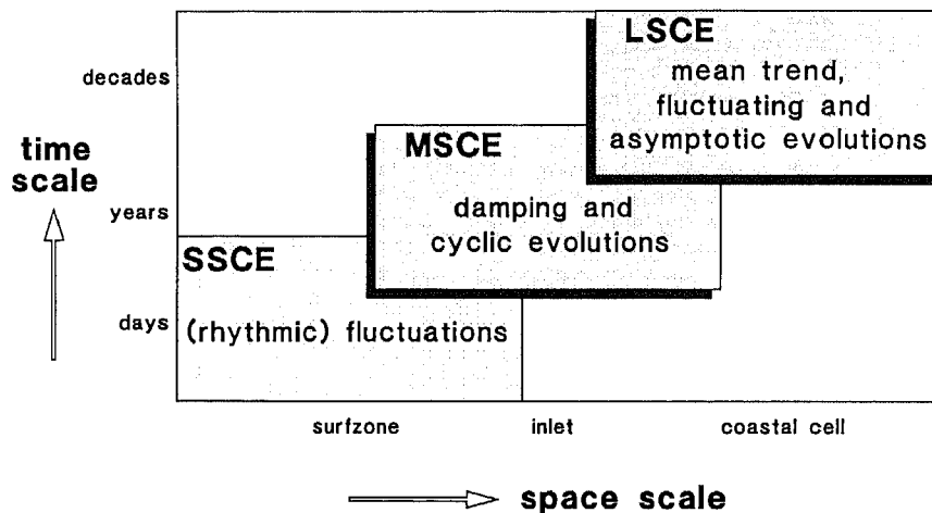
Figure 2 Coastal evolution scales
