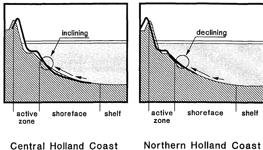
Figure 5 Typical behaviour of the transition between the active zone and the middle shoreface
