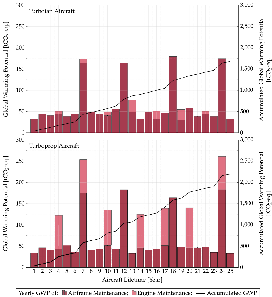
Fig. 6. Yearly distribution of the GWP of the airframe and engine maintenance (primary axis) and the accumulative GWP of total maintenance over the turbofan (top) and turboprop (bottom) aircraft lifetimes (secondary axis).
