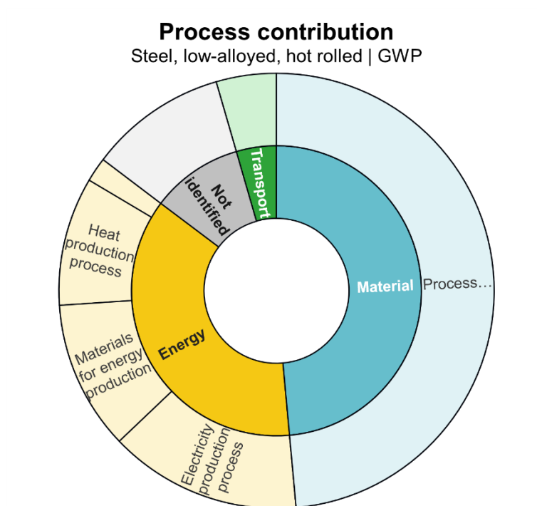
Figure 1 Process contribution (cut-off 0,1%) for the global warming potential (in CO 2 eq.) of low-alloyed hot rolled steel global industrial average assessed from Ecolnvent v3.9 [36]
