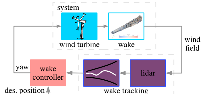
Fig. 1: A block scheme of the general idea of lidar-based closed-loop wake redirection concept.
