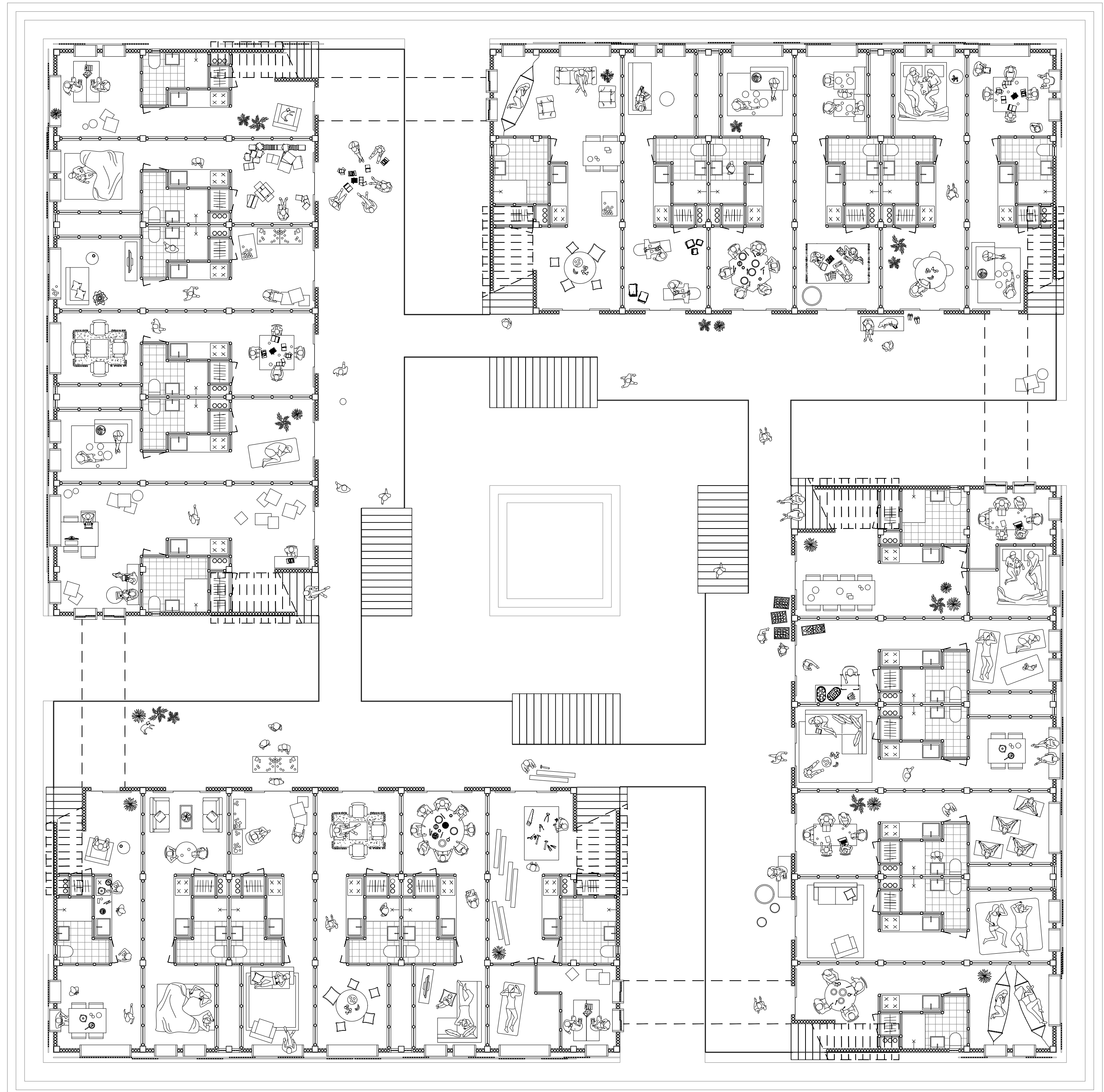
FIRST FLOOR 1 : 100
