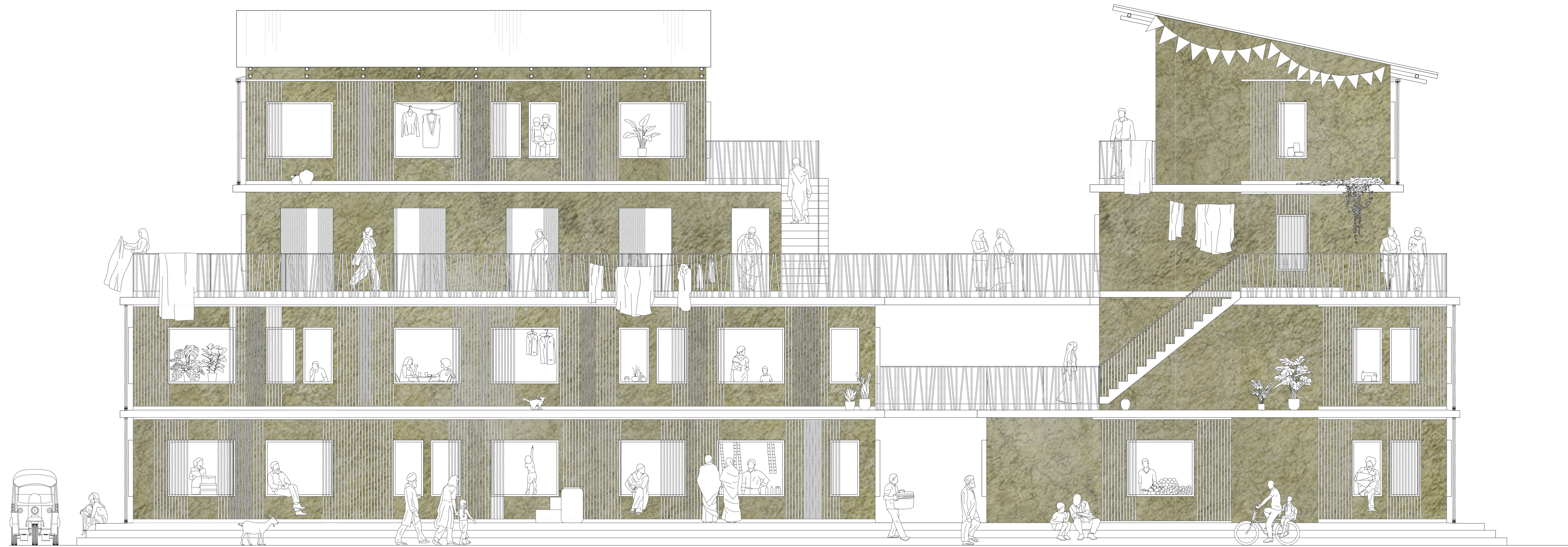
FACADE 1 : 50
