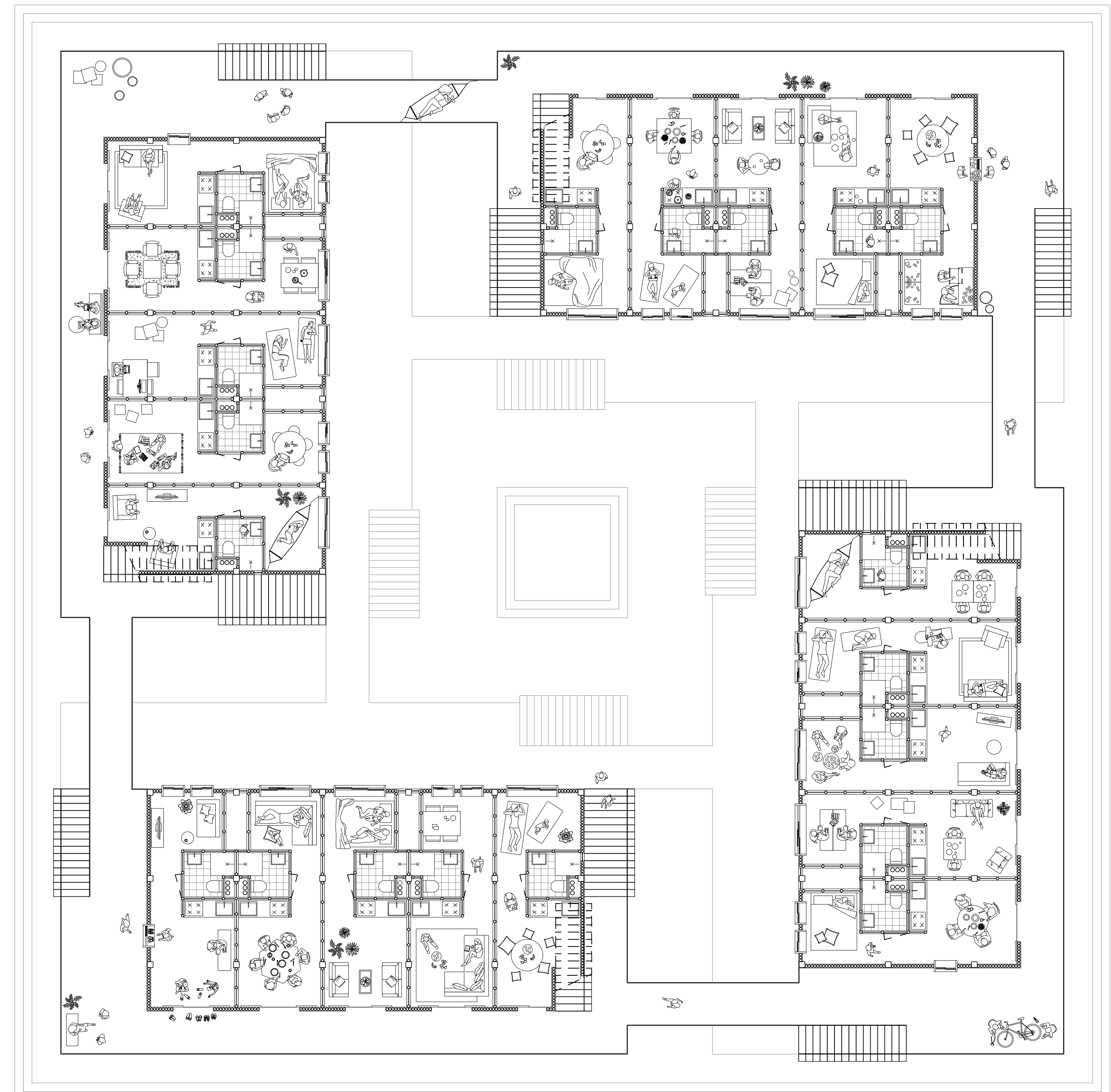
SECOND FLOOR 1 : 100
