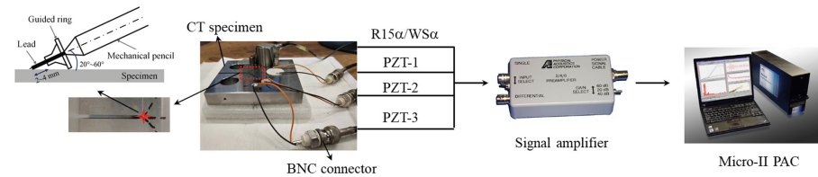
Fig. 7. Experimental set-up
