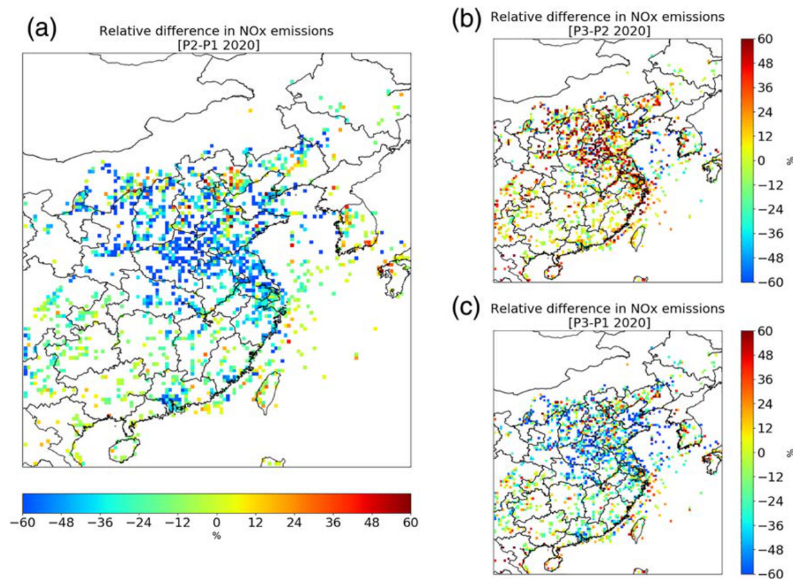
Figure 2. The relative difference in NO x emissions between (a) P2 and P1, (b) P3 and P2, and (c) P3 and P1. P1 is 3–23 January. P2 is 8–28 February. P3 is 18 March–7 April. The changes in emissions are shown in the figure for emissions higher than 3 kg(N)/km 2 /day in P1 to remove areas with dominating biogenic emissions or rural areas.
