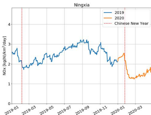
Figure 4. Time series (1 January 2019–28 April 2020) of daily \text{NO}_x emissions in Ningxia Province.
