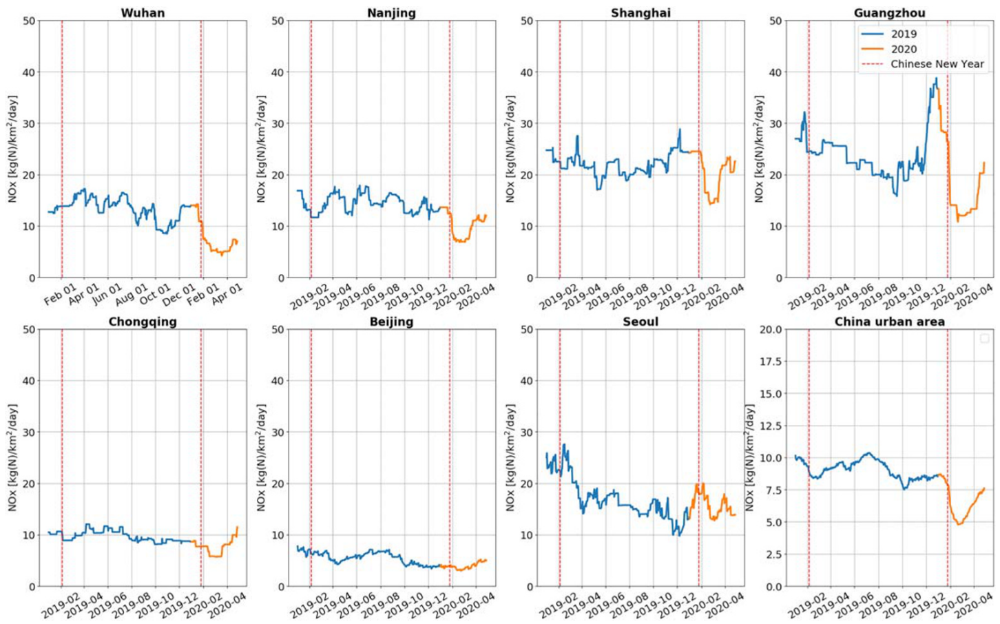
Figure 3. Time series (1 January 2019–28 April 2020) of daily \text{NO}_x emissions in seven cities and urban China. Six Chinese cities are considered (Wuhan, Nanjing, Shanghai, Guangzhou, Chongqing, and Beijing) as well as Seoul. The location of Chinese cities is shown in Figure S4.
