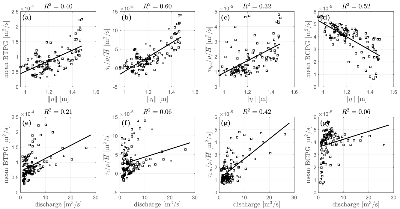
Figure A1. Correlation between the mean barotropic pressure gradient (BTPG), \tau_t , \tau_{b,u} , the mean baroclinic pressure gradient (BCPG), and tidal amplitude, river discharge.
