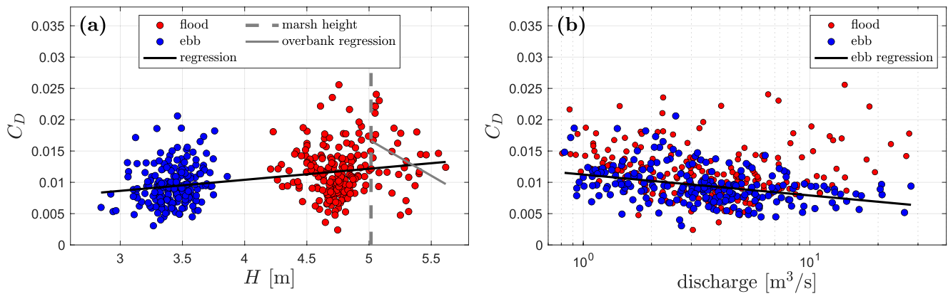
Figure 6. (a): Drag coefficient versus water depth at the bend apex. Linear regressions give R^2 = 0.10 (p - value < 0.001) for the overall data and R^2 = 0.14 (p - value = 0.03) for the overbank cases (water depth exceeds marsh height). (b): Drag coefficient versus river discharge. R^2 = 0.13 (p - value < 0.001) for ebb tides, and R^2 = 0.00 (p - value > 0.05) for flood tides.
