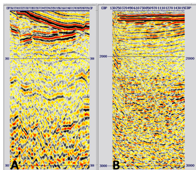
Figure 8 Comparison of the Pre-Stack-Time-Migrated Stack between (A) explosive data and (B) eVibe data til 1500ms.
