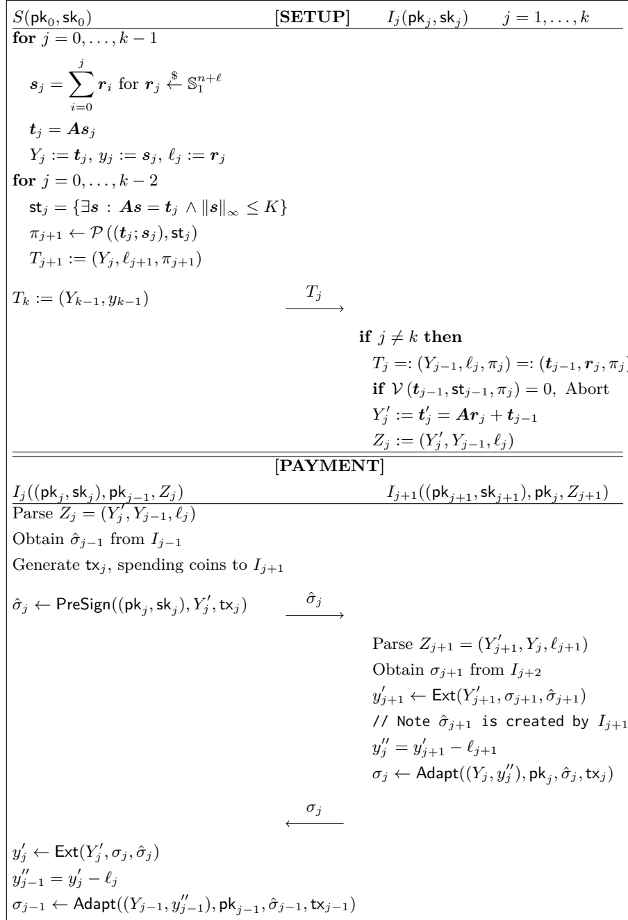
Fig. 2: Anonymous multi-hop payments using LAS. We assume that (i) T_j 's are transmitted confidentially, (ii) pre-signature transmission from I_j to I_{j+1} happens only if that from I_{j-1} to I_j already happened, and (iii) signature transmission from I_{j+1} to I_j happens only if that from I_{j+2} to I_{j+1} already happened.
