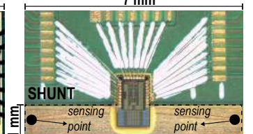
Fig. 5b: Chip on PCB trace.
