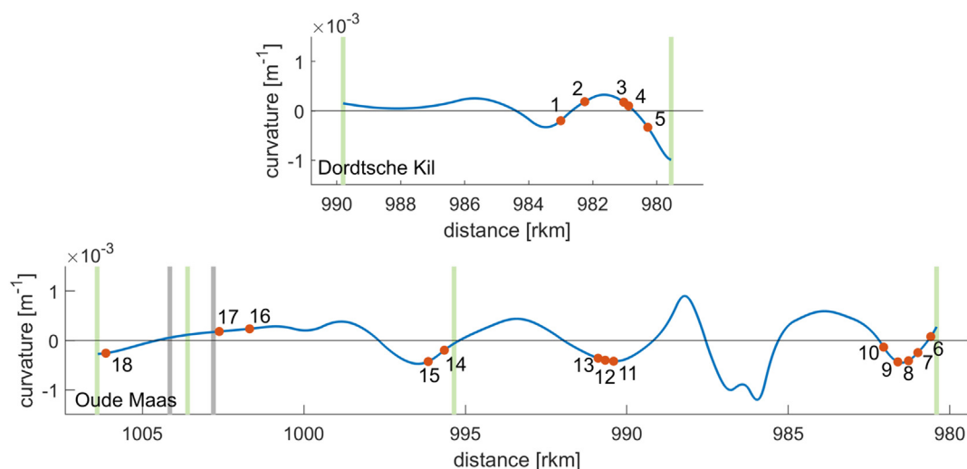
Fig. 5. Inverse value of the radius of curvature plotted against the distance along the river. Red dots indicate the scour hole locations, the green bars the confluences and the grey bars the bridges. As groyne scours are excluded from the database, these are not indicated.
