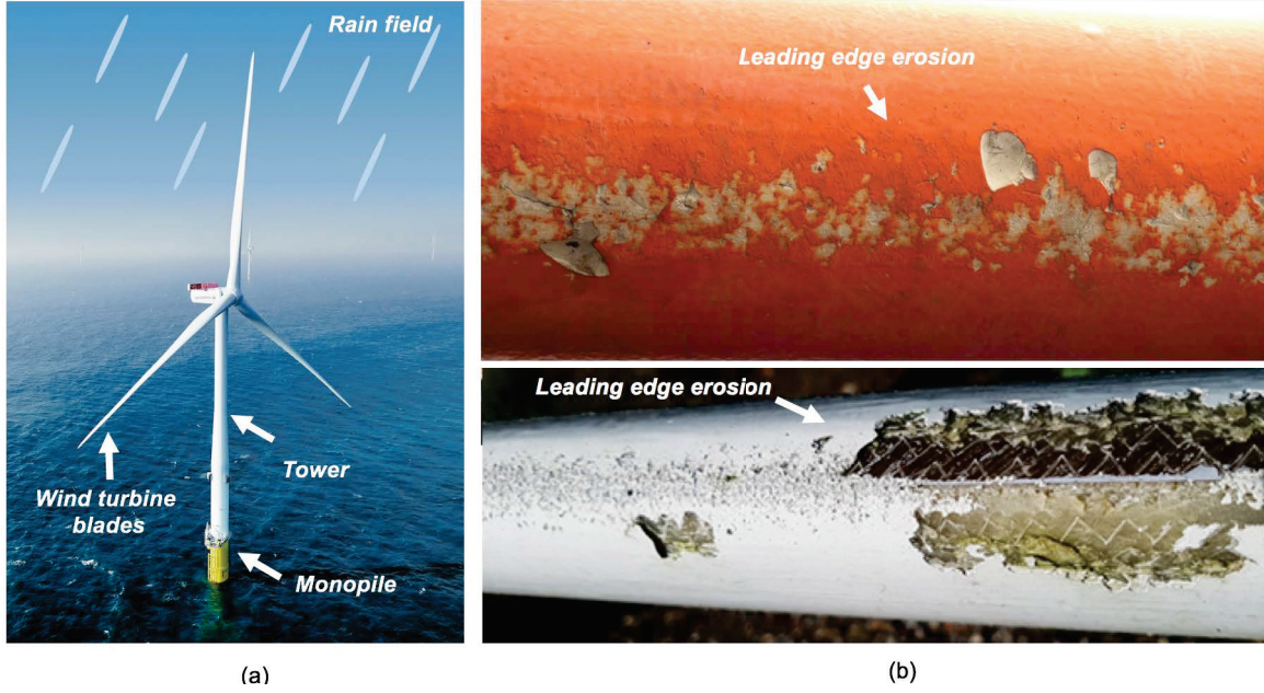
Figure 1: (a) Wind turbine exposed to rain field [Modified picture from source: Vattenfall group[11]] (b) Leading edge erosion of wind turbine blades [12, 13][Source: TNO and DURALEDGE project]
