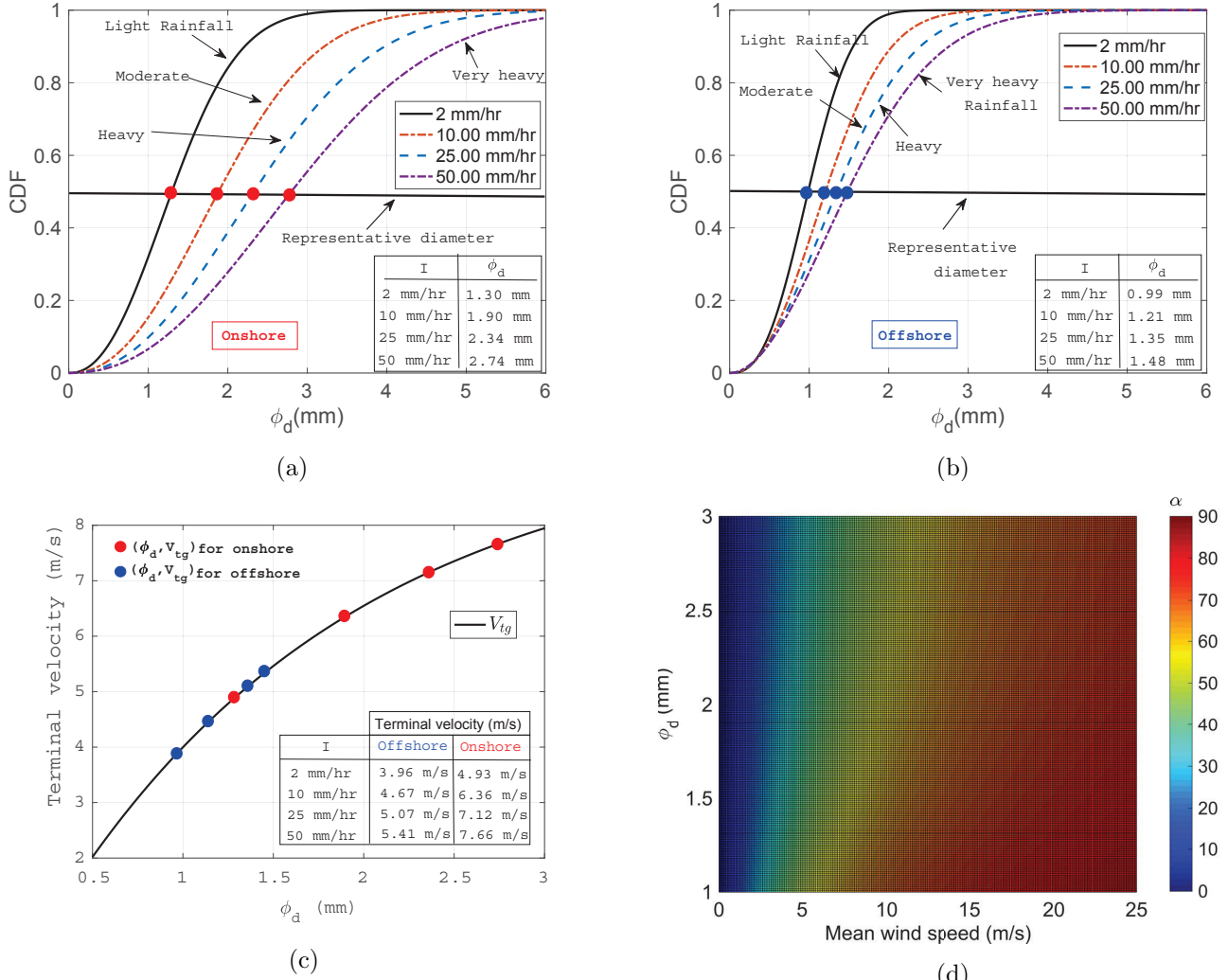
Figure 8: Choice of \phi_d for different I (a) Onshore - Best distribution (b) Offshore - distribution by [25] (c) V_{tg} (red - onshore; blue-offshore) (d) Variation of \alpha (degrees) with varying \phi_d and U_w
