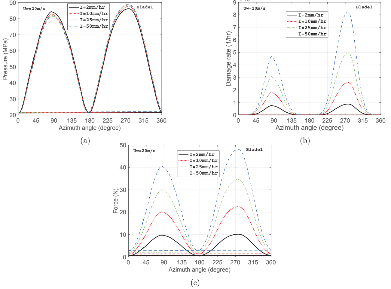
Figure 11: Comparison of (a) p_{wh} (b) \dot{D}_i (c) F_{imp} for I = 2mm/hr, 10mm/hr, 25mm/hr, 50mm/hr
