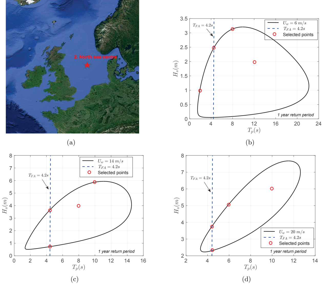
Figure 7: (a) North sea centre offshore site; 2D contour surface for H_s , T_p for (b) U_w=6m/s (c) U_w=14m/s (d) U_w=20m/s and selected load cases
