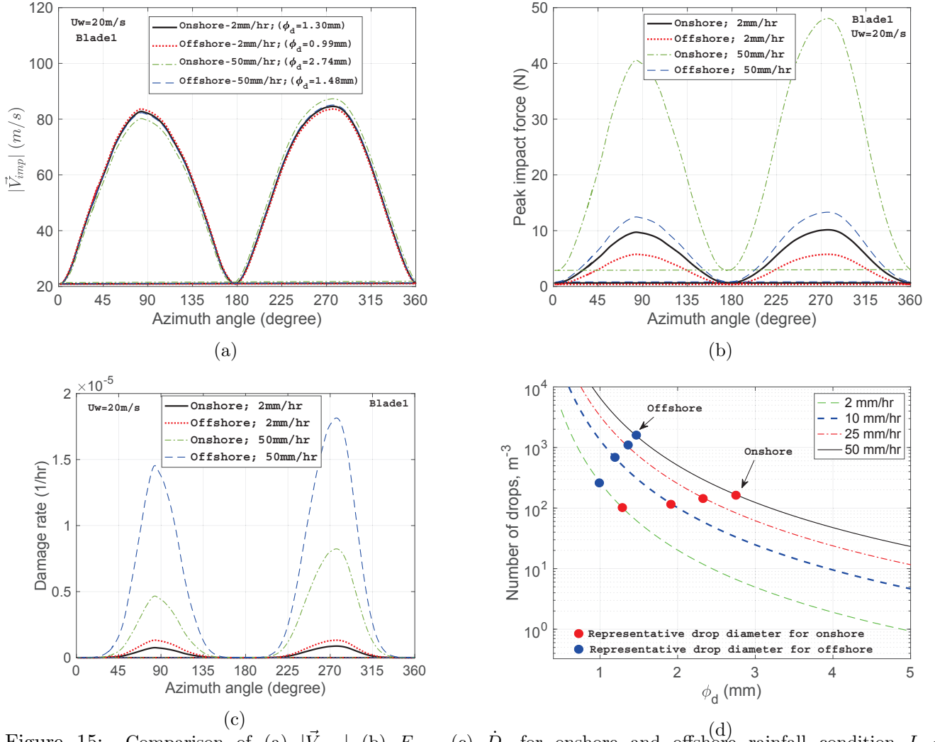
Figure 15: Comparison of (a) |\vec{V}_{imp}| (b) F_{imp} (c) \dot{D}_i for onshore and offshore rainfall condition I = 2mm/hr, 50mm/hr (d) q for several \phi_d and I = 2mm/hr, 10mm/hr, 25mm/hr, 50mm/hr
