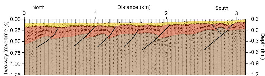
FIGURE 10 Interpreted version of the passive seismic section from Figure 9a; Middle Miocene -yellow, Paleogene - dark red and Basement - brown, possible Miocene faults - black lines.
