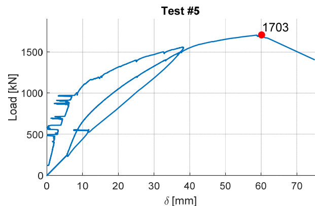
Figure 14 Load-displacement beam test 5
