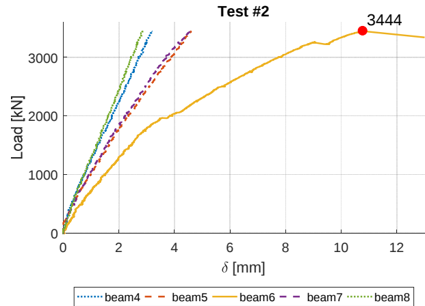
Figure 12 Load-displacement beam test 2.
