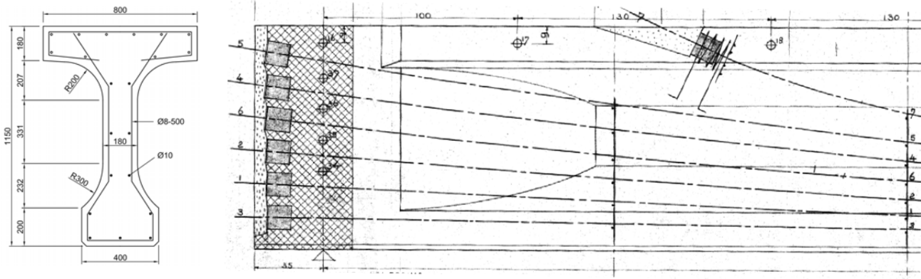
Figure 3 Cross section beam with reinforcement, measurements in mm (left), side view of beam close to the support showing the curved prestressing cables, measurements in cm (right).
