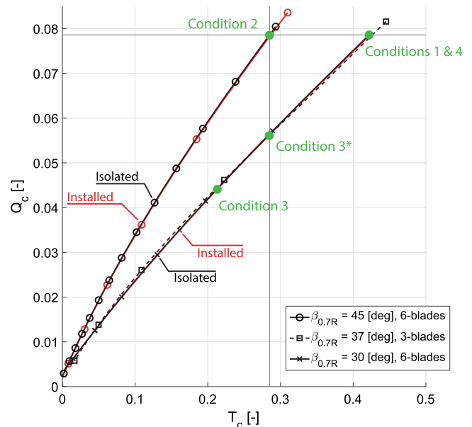
Fig. 15 Calculated performance curves for the TUD-XPROP-S with six and three blades, in isolated and installed conditions. Chosen operating conditions marked in green.
