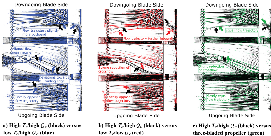
Fig. 27 Overlays of (zoomed in) processed oil flow images, comparing high- T_c /high- Q_c with each of the other conditions. Upper surface, \alpha = 8^\circ , \delta_f = 15^\circ . Freestream from left to right.
