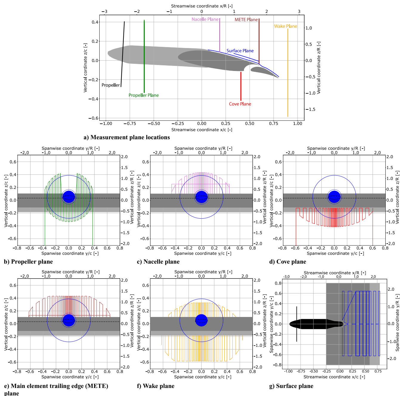
Fig. 10 Illustration of the locations and corresponding paths of the measurement planes at \alpha = 0 deg, \delta_f = 0 deg. View in freestream direction, perpendicular to the measurement planes.
