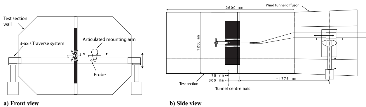
Fig. 8 Illustration of the traverse setup for the straight probe. Dimensions in mm.
