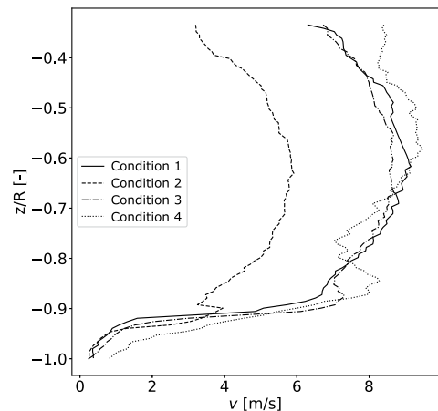
Fig. 17 Radial distribution of the y-component of velocity at \psi = 270 deg.
