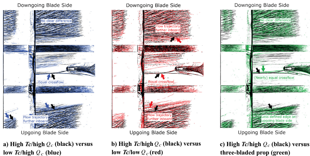
Fig. 28 Overlays of (zoomed in) processed oil flow images, comparing high- T_c /high- Q_c with each of the other conditions. Lower surface, \alpha = 8^\circ , \delta_f = 15^\circ . Freestream from right to left.
