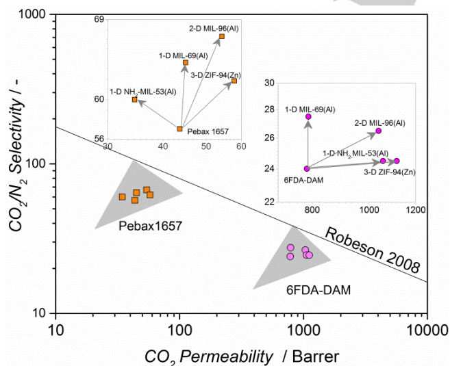
Figure 11. Robeson plot of \text{CO}_2 / \text{N}_2 couple ( \text{CO}_2 selectivity versus permeability) of MOF-MMMs and neat 6FDA-DAM and Pebax membranes at 298 K and 2 bar absolute feed pressure (mixed gases). The insets are the enlarged views of the corresponding membrane performance. The Robeson upper bound (2008) is shown for reference. The MOF loading in all MMMs is 25 wt. %.
