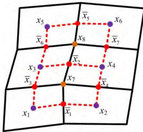
Figure 1—The schematic of control volumes and intersection volumes
