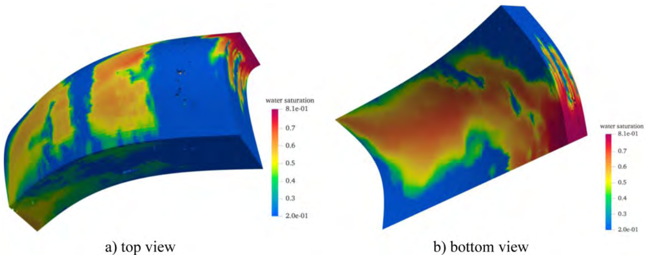
Figure 12—Water saturation distribution of the MPFA-O after 5000 days (8 cores)
