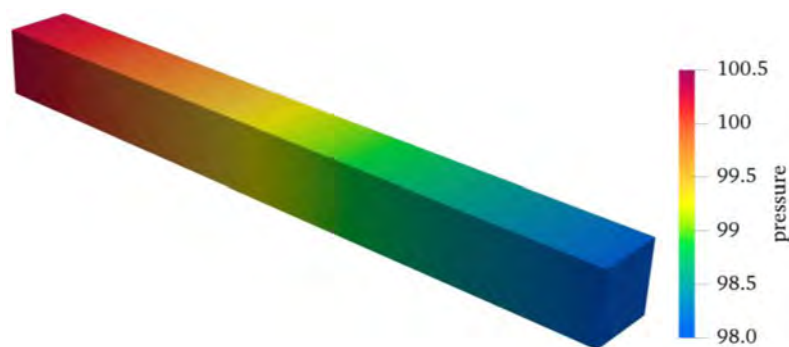
Figure 5—Pressure distribution of the numerical solution
