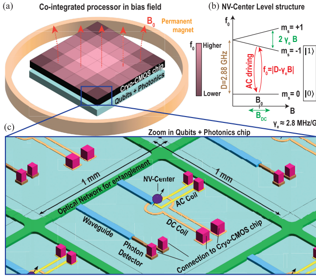
Fig. 1. Envisioned color-center-based quantum processor. (a) 3-D-integrated cryo-CMOS, photonics, and qubits that are biased in a permanent magnetic field. (b) Level structure of the NV-center's electron spin qubit. (c) Components on the Qubits + Photonics chip.
