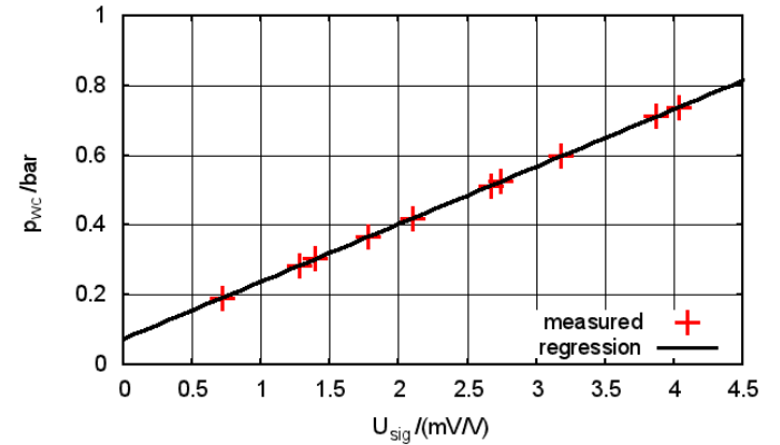
Fig. 5. Regression line and measured data points for the reference pressure sensor.
