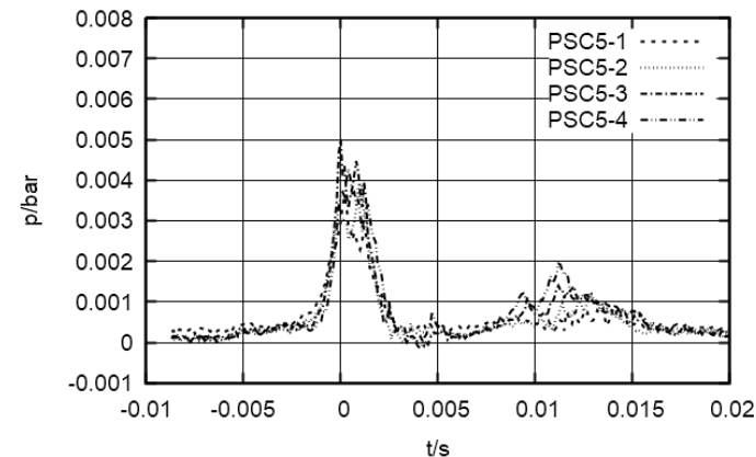
Fig. 14. PSC5 pressure time series of first popping sound.
