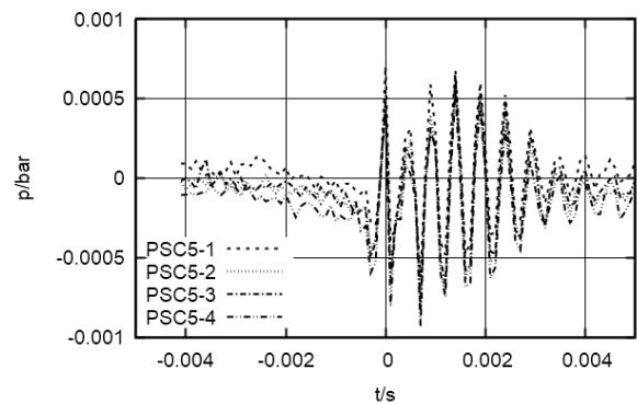
Fig. 12. PSC5 pressure time series of third snapping sound.
