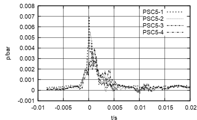
Fig. 15. PSC5 pressure time series of second popping sound.
