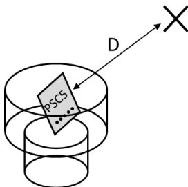
Fig. 9. Sketch of setup for dynamic tests. Mark (x) denotes approximate position of sound source.
