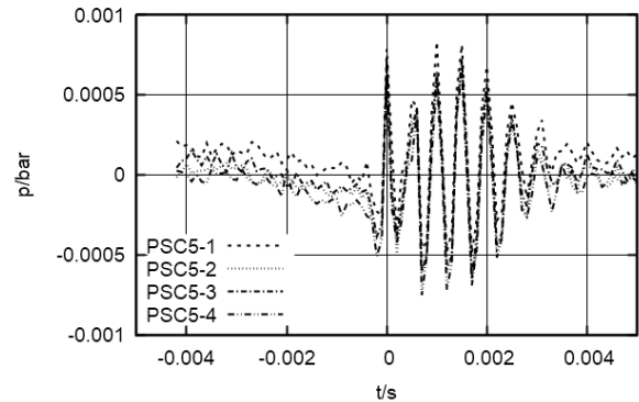
Fig. 11. PSC5 pressure time series of second snapping sound.
