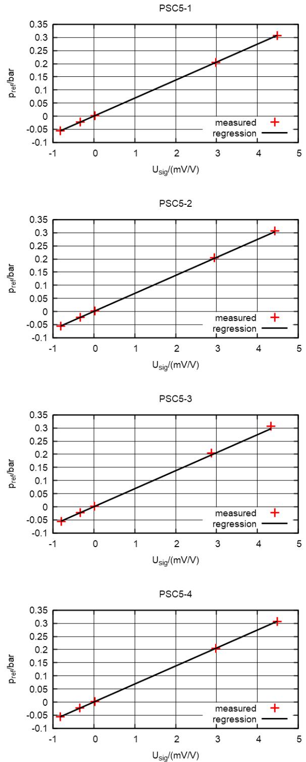
Fig. 7. Calibration lines of the four operational PSC5 sensors.
