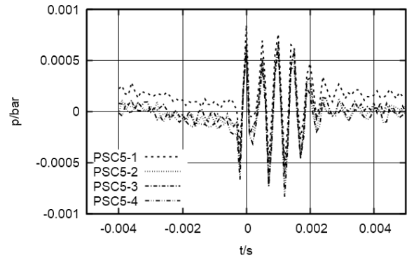
Fig. 10. PSC5 pressure time series of first snapping sound.
