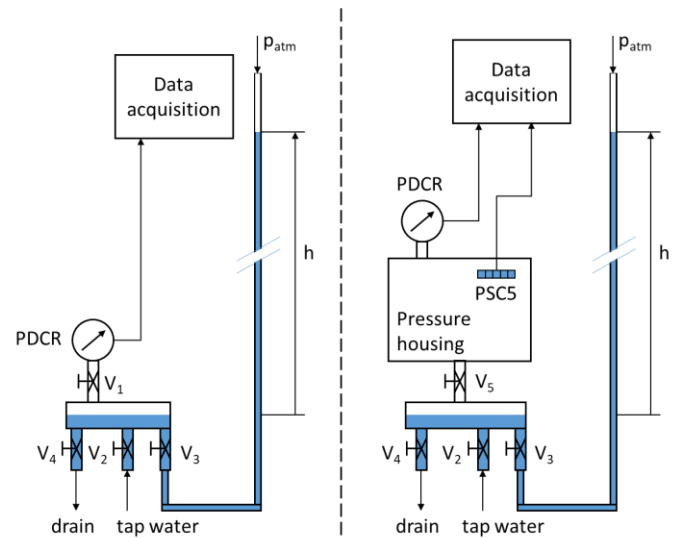
Fig. 3. Calibration test setups. Static calibration of reference sensor PDCR (left), calibration of pressure sensor cluster (PSC5) against reference sensor PDCR (right).
