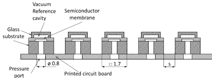
Fig. 2. Schematic elevation of a pressure sensor cluster, not to scale. Dimensions in mm.
