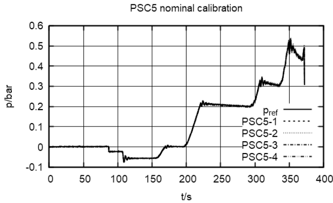
Fig. 6. Time series of PSC data and reference pressure before calibration of PSC sensors.
