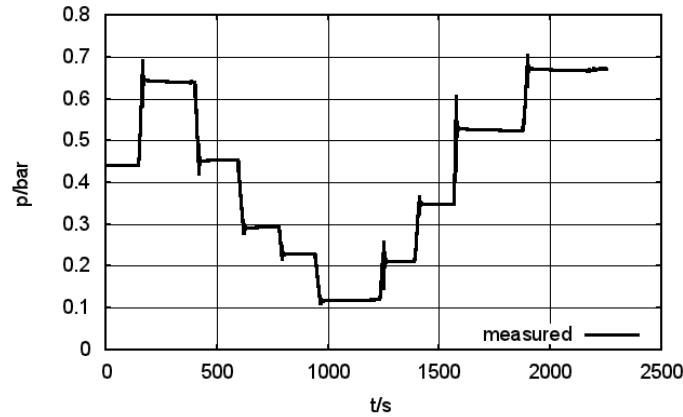
Fig. 4. Measured signal during reference sensor calibration.
