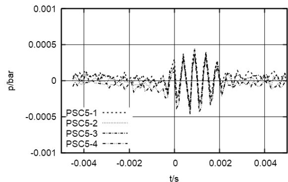
Fig. 13. PSC5 pressure time series of fourth snapping sound.
