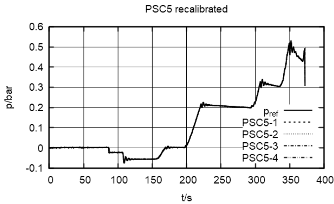
Fig. 8. Time series of PSC5 data and reference pressure after calibration of PSC5 sensors.
