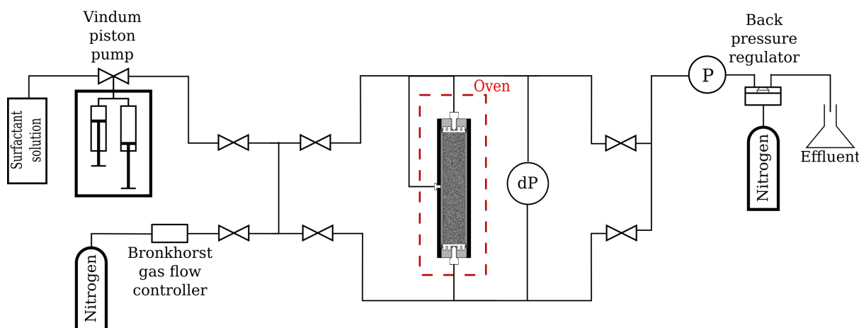
Figure 1 Schematic of the experimental apparatus.
