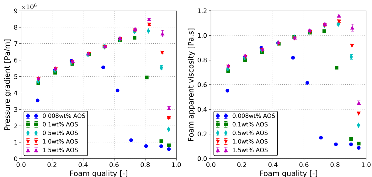
Figure 3 (a) Steady-state pressure gradient along the core and (b) calculated apparent viscosity at different foam qualities (gas fractional flow) using eq 1 for different AOS concentrations. The total flow rate was set to a constant value of 1 mL/min.
