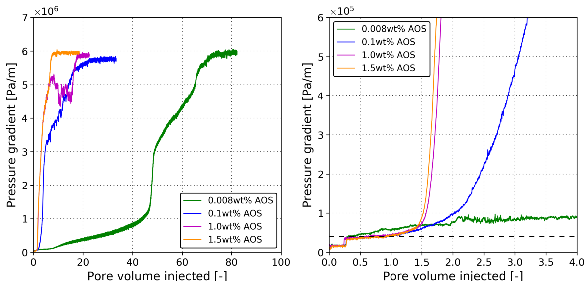
Figure 2 (a) Pressure history of the foam-generation phase of the experiments with a gas volume fraction (foam quality) of 0.30 for different AOS concentrations. (b) Magnification of the first four pore volumes of injection.
