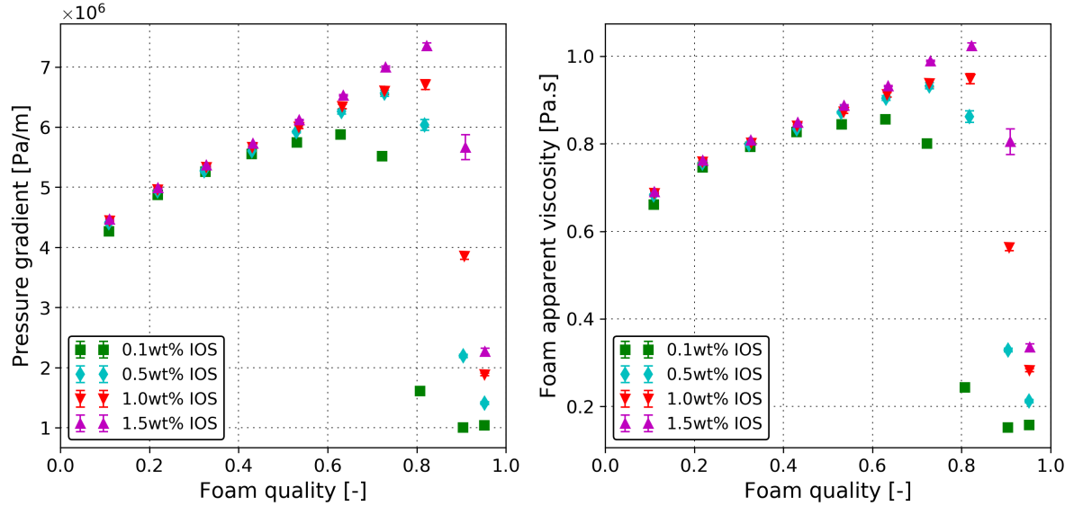
Figure 4 (a) Steady-state pressure gradient along the core and (b) calculated apparent viscosity at different foam qualities, f_g for different IOS concentrations. The total flow rate was set to a constant value of 1 mL/min.
