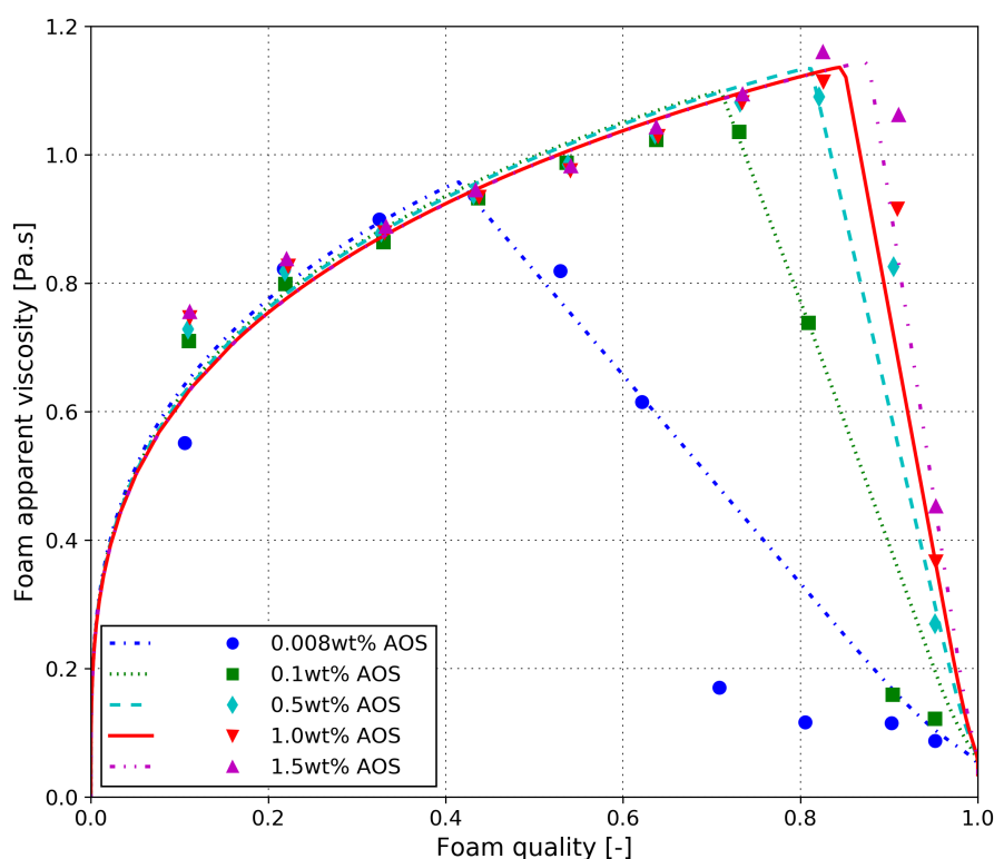
Figure 6 Simulation of the experimental data using F_2 and F_5 functions assuming constant set of parameters (Table 5) but different values of fmdry (Table 6) to capture the effect of surfactant concentration.
