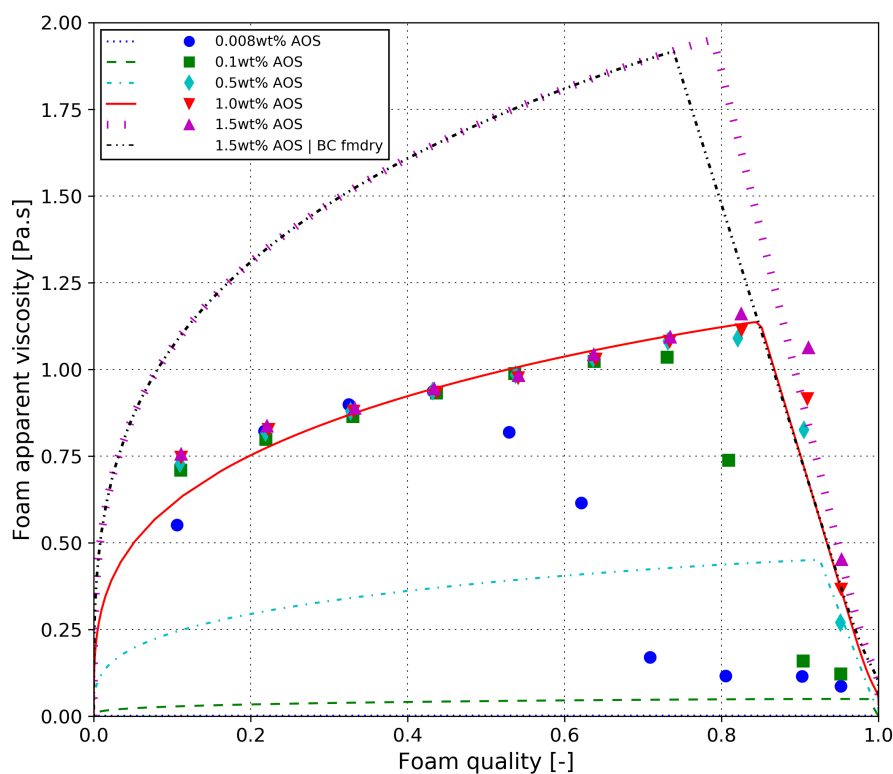
Figure 5 Modeling of foam apparent viscosity using F_1 , F_2 , and F_5 functions assuming a constant set of parameters (Table 5) but different values of C_s and f_{mdry} (Table 6) to capture the effect of surfactant concentration. The dashed-dotted-dotted line shows the 1.5 wt % AOS case using the same f_{mdry} value as in the base case.
