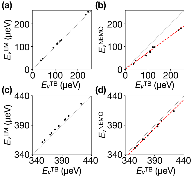
FIG. 15. Valley splitting comparisons between effective-mass theory, two-band tight-binding, and NEMO-3D models. [(a) and (b)] Using the same 10 alloy disorder realizations, we calculate valley splittings in three ways. In (a), we compare valley splittings computed from the minimal tight-binding model ( E_v^{\text{TB}} ) and effective-mass theory [ E_v^{\text{EM}} , from Eq. (8)], obtaining nearly perfect agreement. In (b), we compare the minimal tight-binding model to NEMO-3D ( E_v^{\text{NEMO}} ). The red dashed line indicates the best fit to E_v^{\text{NEMO}} = \alpha E_v^{\text{TB}} with \alpha = 0.74 . Gray dotted lines indicate y = x . For both (a) and (b), we use quantum wells of width W = 80 ML and sigmoid interfaces of width \lambda_{\text{int}} = 20 ML. [(c) and (d)] show the same data as (a), (b) for 10 heterostructures with \lambda_{\text{int}} = 1 ML. In (d), the red line indicates the best fit, with \alpha = 0.99 . In all simulations, we assume a vertical electric field of E_z = 5 mV/nm and an orbital energy splitting of \hbar\omega_{\text{orb}} = 2 meV. The NEMO-3D valley splitting results shown here are the same used in Fig. 6(c).
