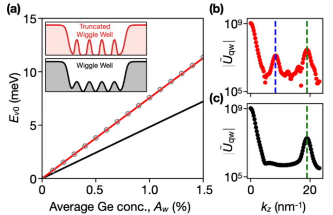
FIG. 22. For a fixed average Ge concentration in the quantum well A_w , the truncated Wiggle well yields larger E_v than the normal Wiggle well. (a) Deterministic valley splitting values E_{v0} , for normal ( E_{v0}^w , black) and truncated ( E_{v0}^{\text{tr}} , red) Wiggle wells, plotted against the average Ge concentration in the quantum well, A_w . The theoretical estimate E_{v0}^{\text{tr}} = (\pi/2)E_{v0}^w is also shown with gray circles. (Inset) Schematic illustrations of the truncated (red) and normal (black) Wiggle wells. [(b) and (c)] The weighted Fourier transforms of the weighted quantum well potentials |\tilde{U}_{\text{qw}}| for (b) truncated and (c) normal Wiggle wells, for the Ge concentrations A_w = 0.01 . Vertical green dashed lines in (b) and (c) highlight the wave vector k_z = 2k_0 , and the vertical blue dashed line in (b) highlights the wave vector k_z = 4k_0 , aliased down to a lower value by the discrete lattice spacing. All simulations are performed with a vertical electric field of E_z = 5 mV/nm, a quantum well width of W = 80 ML, a sigmoidal interface of width \lambda_{\text{int}} = 10 ML, and Ge barrier concentration of Y_s = 0.3 .
