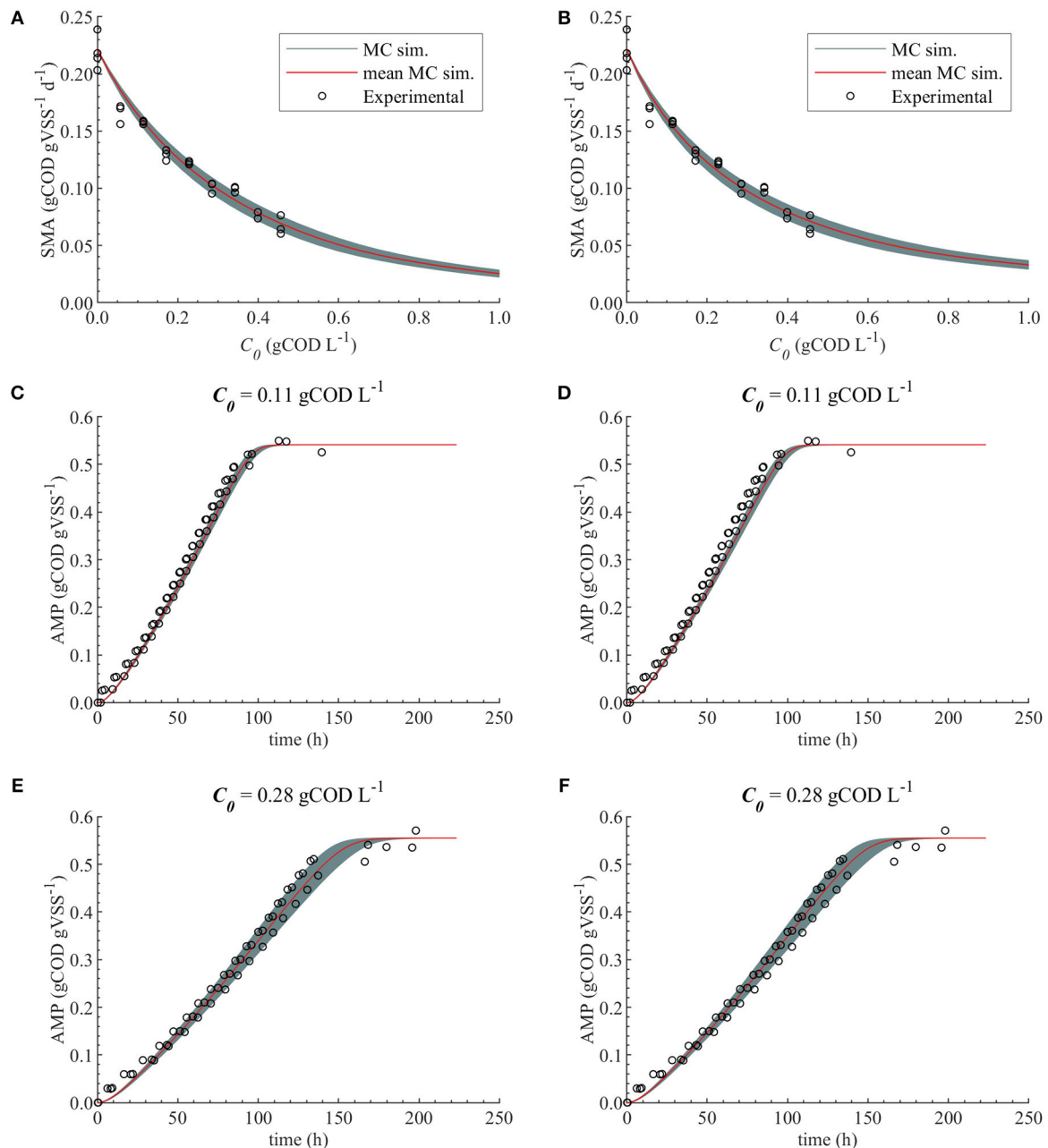
FIGURE 6 | Monte Carlo simulations with uncertainty \theta \sim N(\hat{\theta}, \sigma_{\theta}^2) and subset \theta = \{K_I\} for M2a and M2b. Experimental data, MC simulations (MC sim.) and mean MC simulations for: SMA for M2a (A) and M2b (B), AMP at 0.11 \text{ gCOD L}^{-1} of polymer for M2a (C) and M2b (D) and AMP at 0.28 \text{ gCOD L}^{-1} for M2a (E) and M2b (F).
