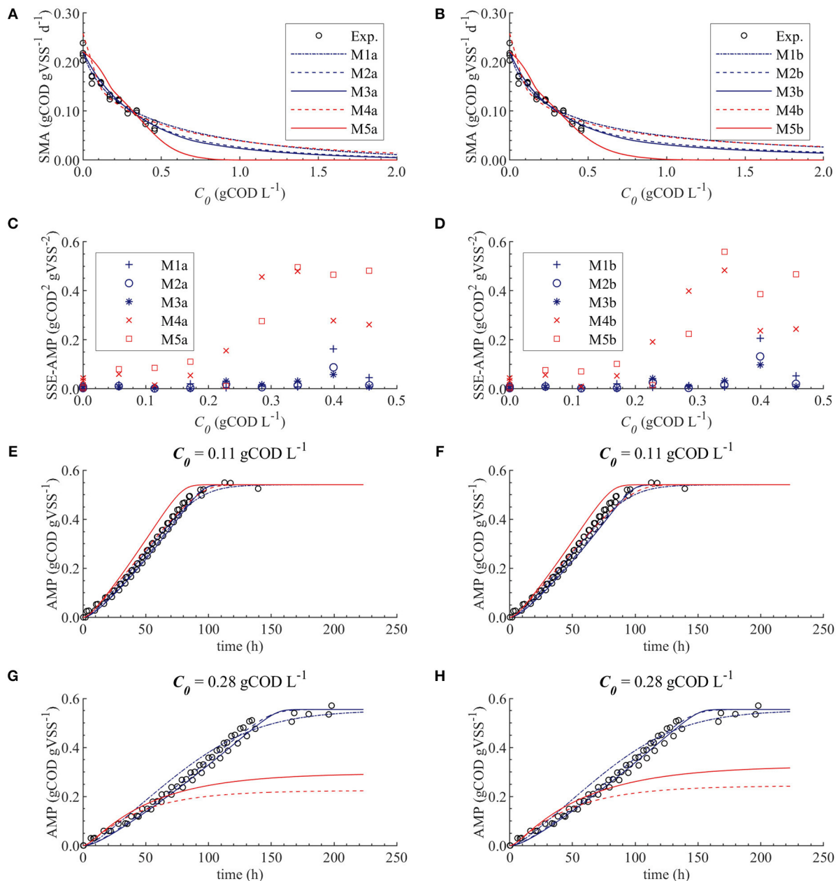
FIGURE 5 | Simulations with parameter estimation results for the SMA inhibition, with parameter subset \theta = \{K_I\} : experimental and simulated SMA for M1a to M5a (A) and M1b to M5b (B), SSE-AMP for M1a to M5a (C) and M1b to M5b (D), experimental and simulated AMP at 0.11 gCOD L -1 of polymer for M1a to M5a (E) and M1b to M5b (F) and experimental and simulated AMP at 0.28 gCOD L -1 for M1a to M5a (G) and M1b to M5b (H).
